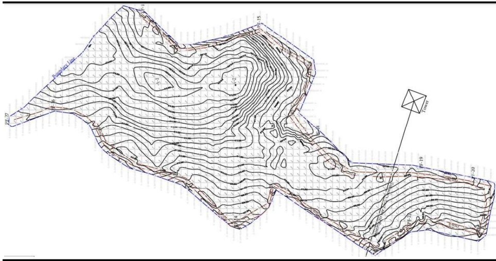
Figure 3.2 Contours of the Proposed Angara Substation Site
