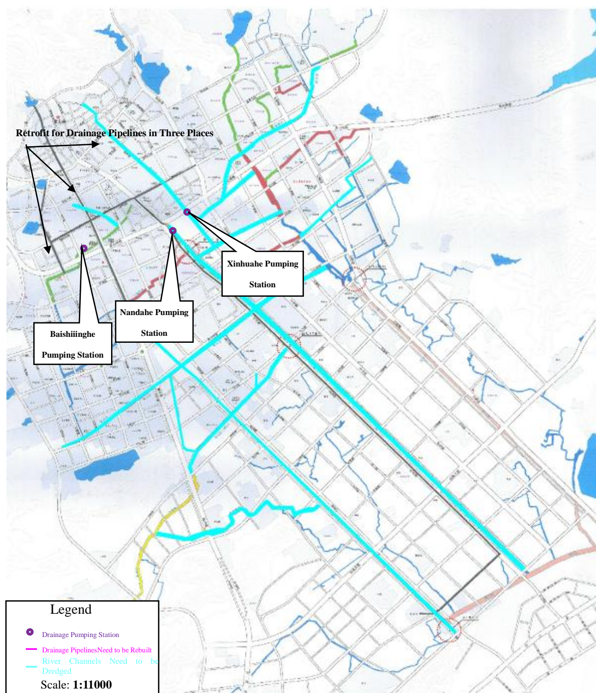
Fig. 2.5-1 Sketch Map of Urban Drainage Pipe Line Retrofit and Locations of Three Boosting Pumping Stations and Main Dredging Watercourses
