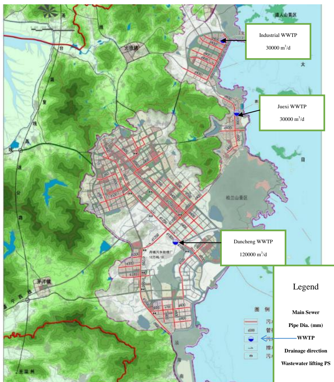
Fig1.3-1 Wastewater Works Planning for Core Urban District
