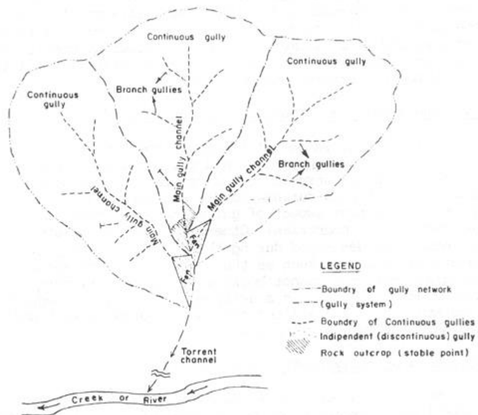
Fig. 4 A gully network (gully system).
