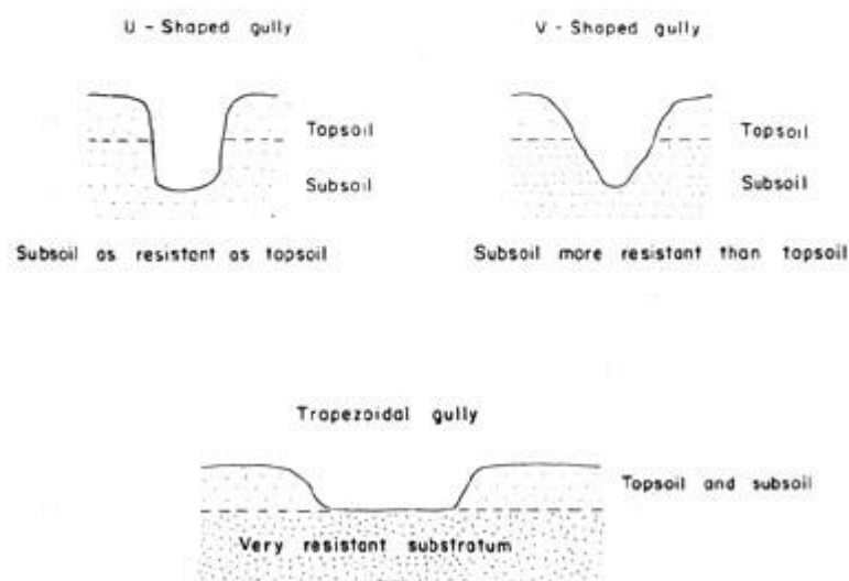
Fig. 3 Gully classes based on shape of gully cross-section. (Source: Weidelt, 1976)
