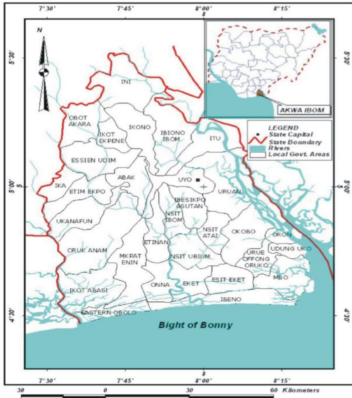
Fig. 1: Map of Akwa Ibom State Showing Geology and Soil
