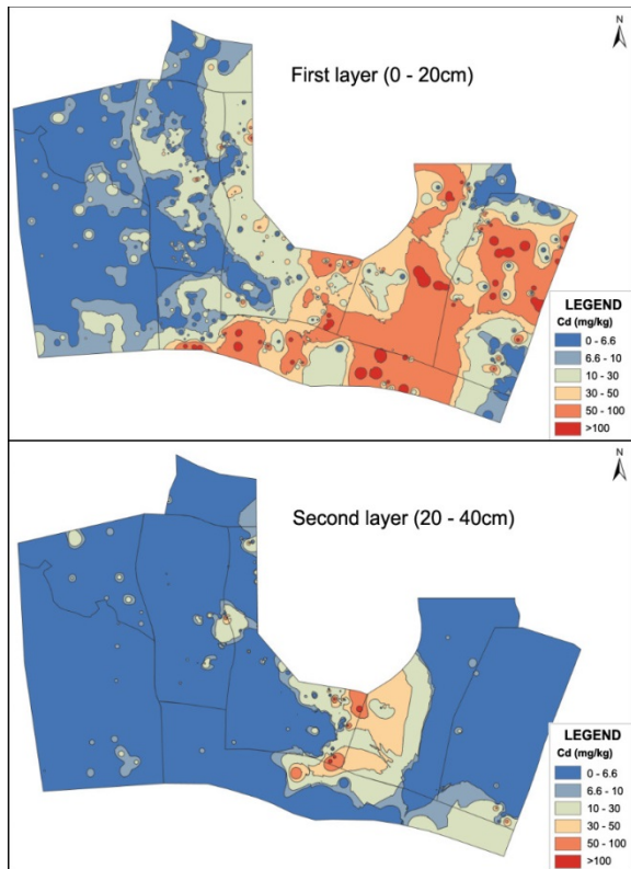
Figure 4 - Concentration Contour Map of Cd Contamination
