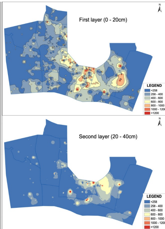
Figure 6 - Concentration Contour Map of Pb Contamination
