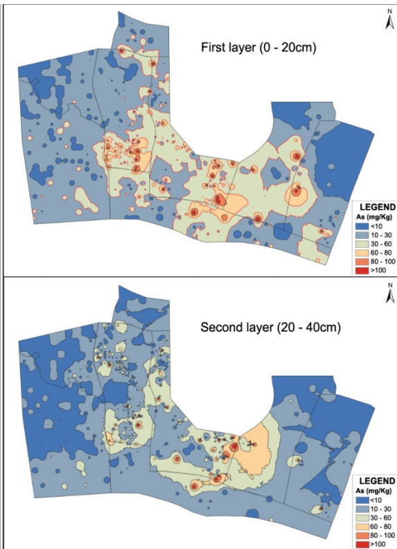
Figure 5 - Concentration Contour Map of As Contamination
