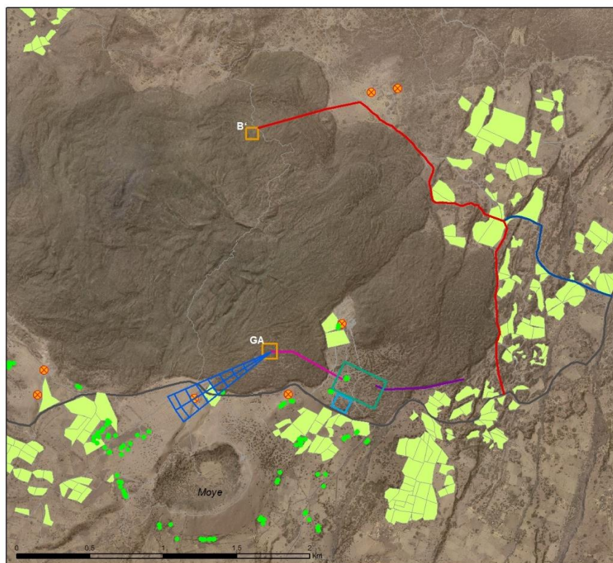
Figure 7.13 Power station, well pads, access roads, current houses around the projects and cultivated land
