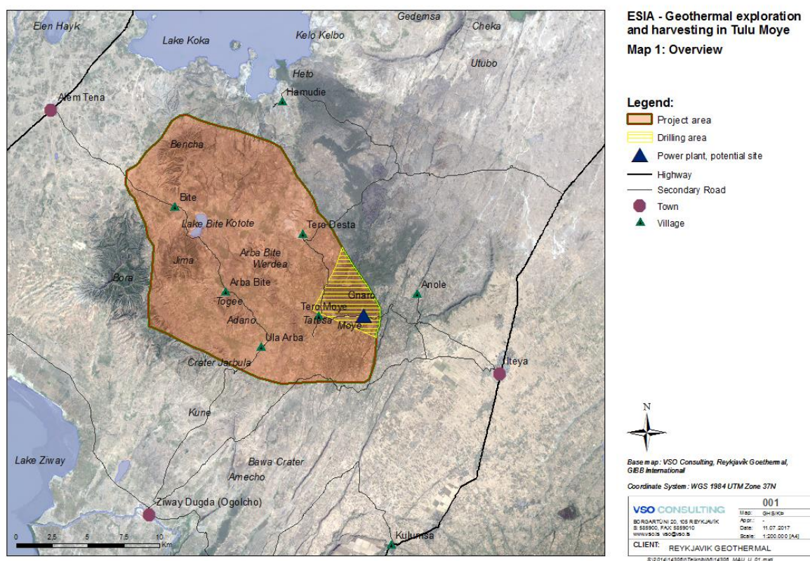
Figure 7.6 Overview of Project and drilling area and accessibility from Alem Tena and Iteya.
