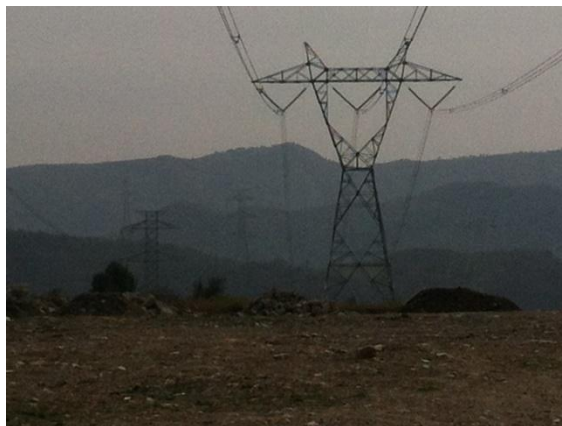
Figure 2: Double Circuit Tower and Single Circuit Flat Formation Tower
