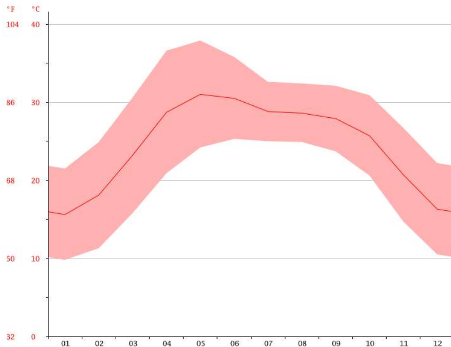
Temperature graph of Tikapur (Source: en.climate-data.org )
