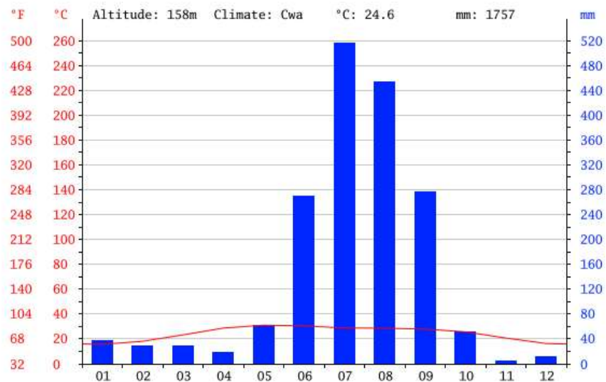
Climograph of Tikapur (Source: en.climate-data.org )
