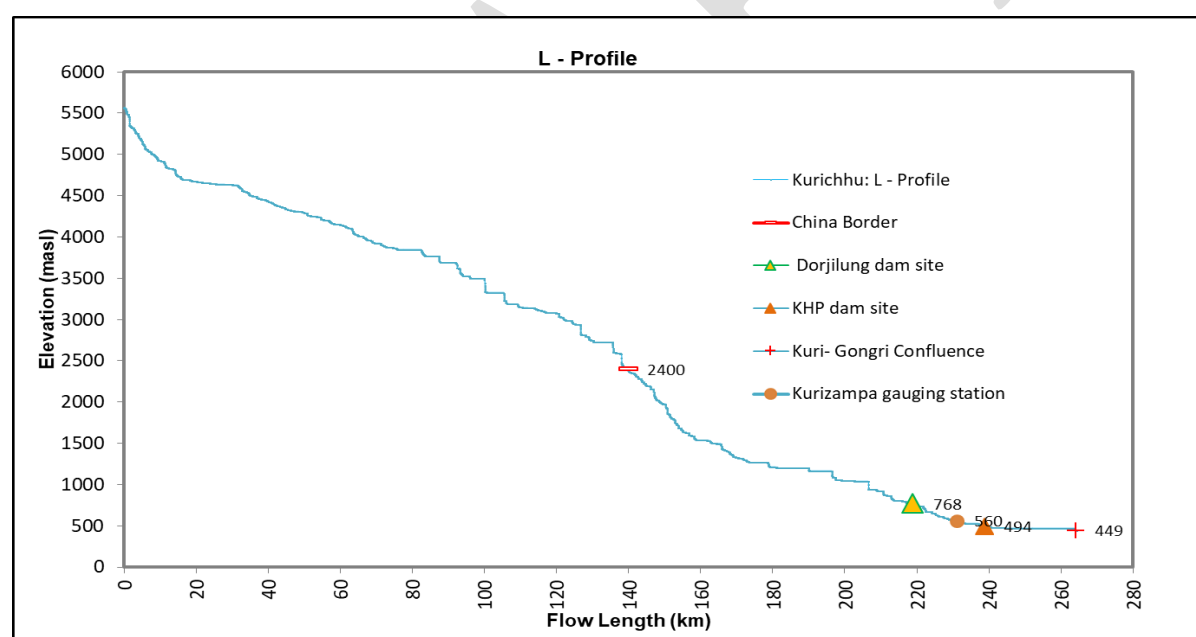
Figure 28: Longitudinal Profile of the Kurichhu
