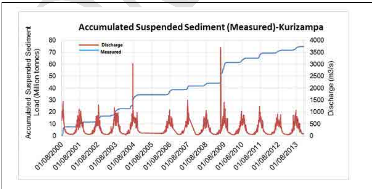
Figure 42: Accumulated suspended sediment transport from Kurizampa site, with discharge time series
