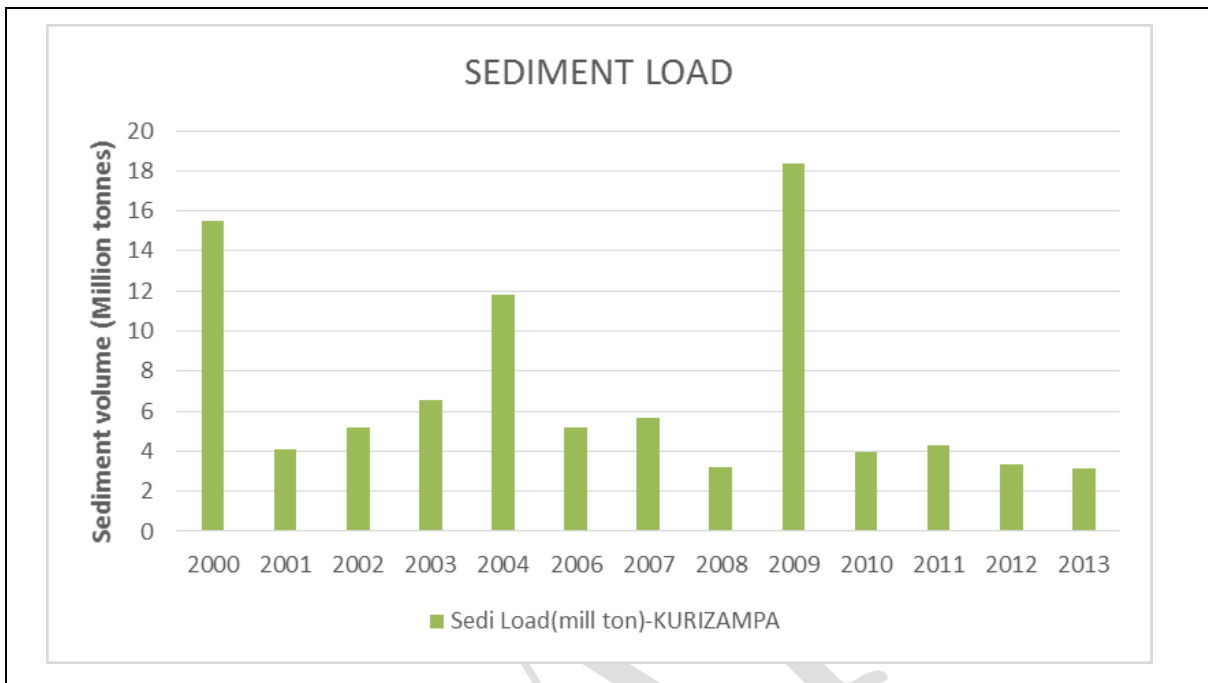
Figure 41: Plot of yearly total Suspended Load at Kurizampa
