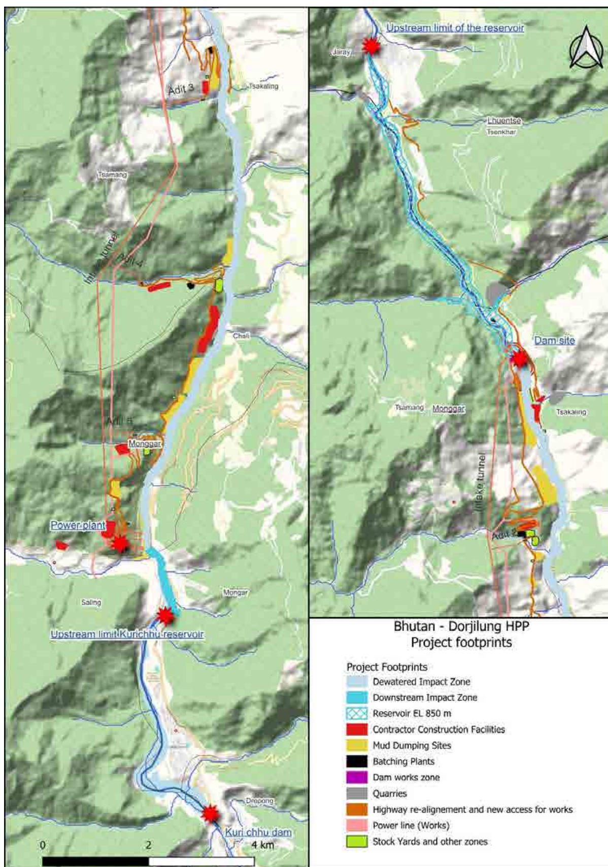
Figure 2: General arrangement of Dorjilung HPP
