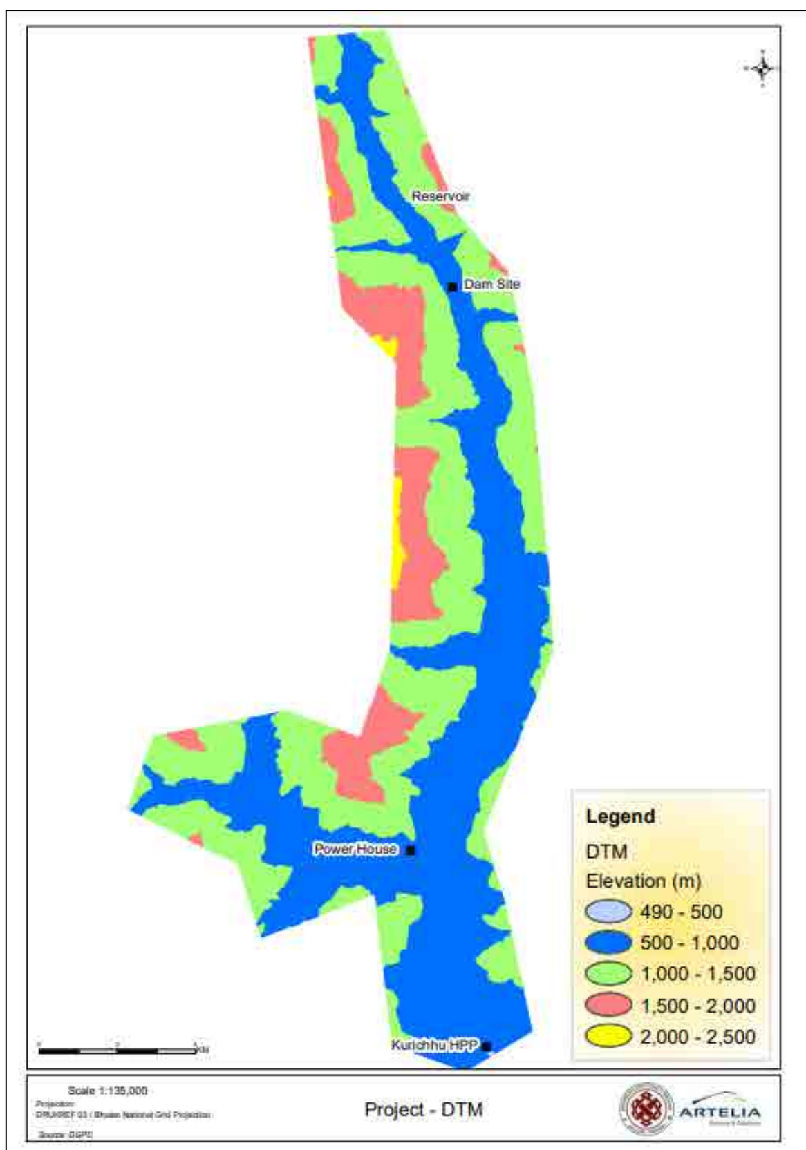
Figure 27: DEM Map of the project Area
