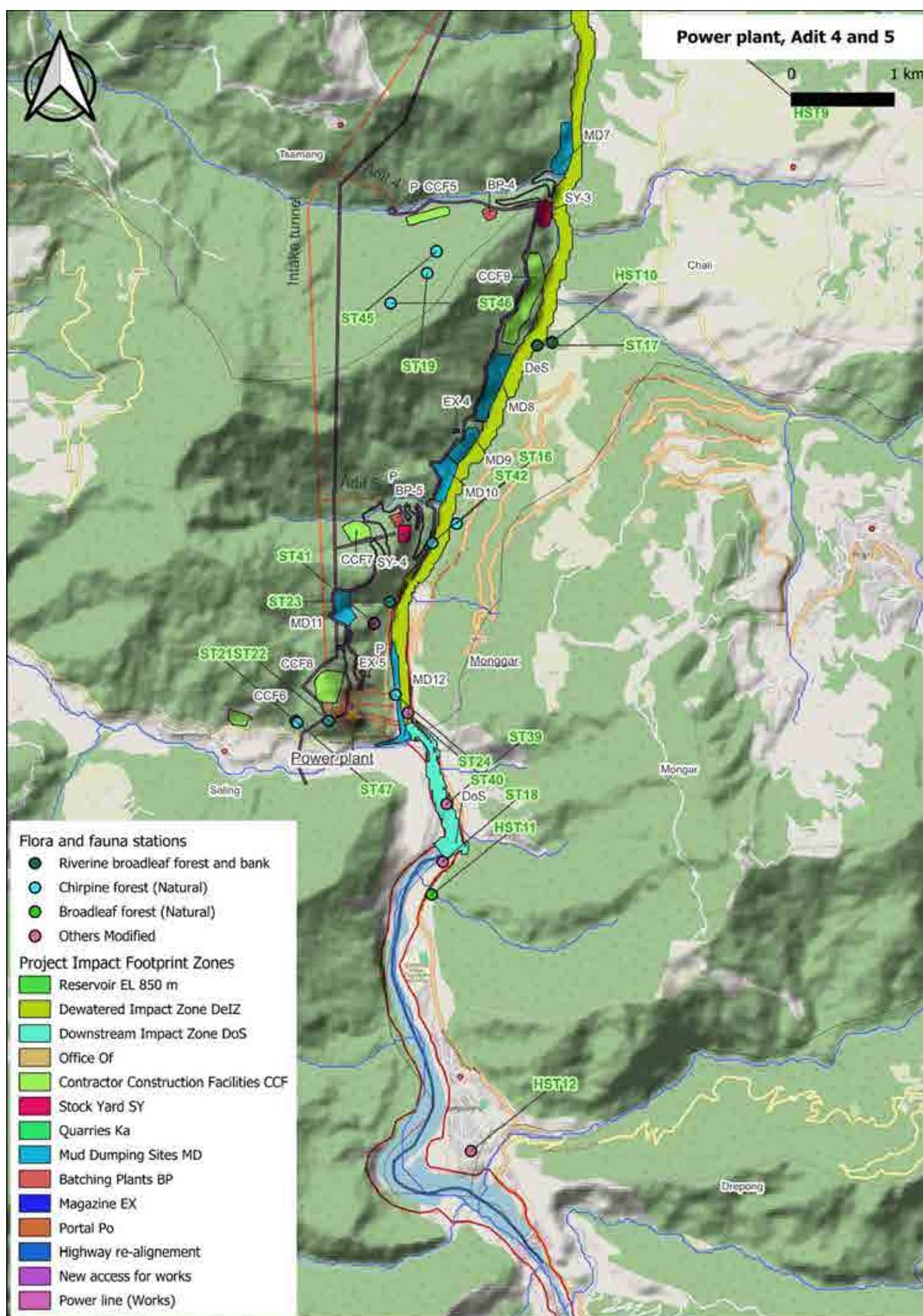
Figure 67: Location of the stations and project footprints (Power plant adit 4 and 5)
