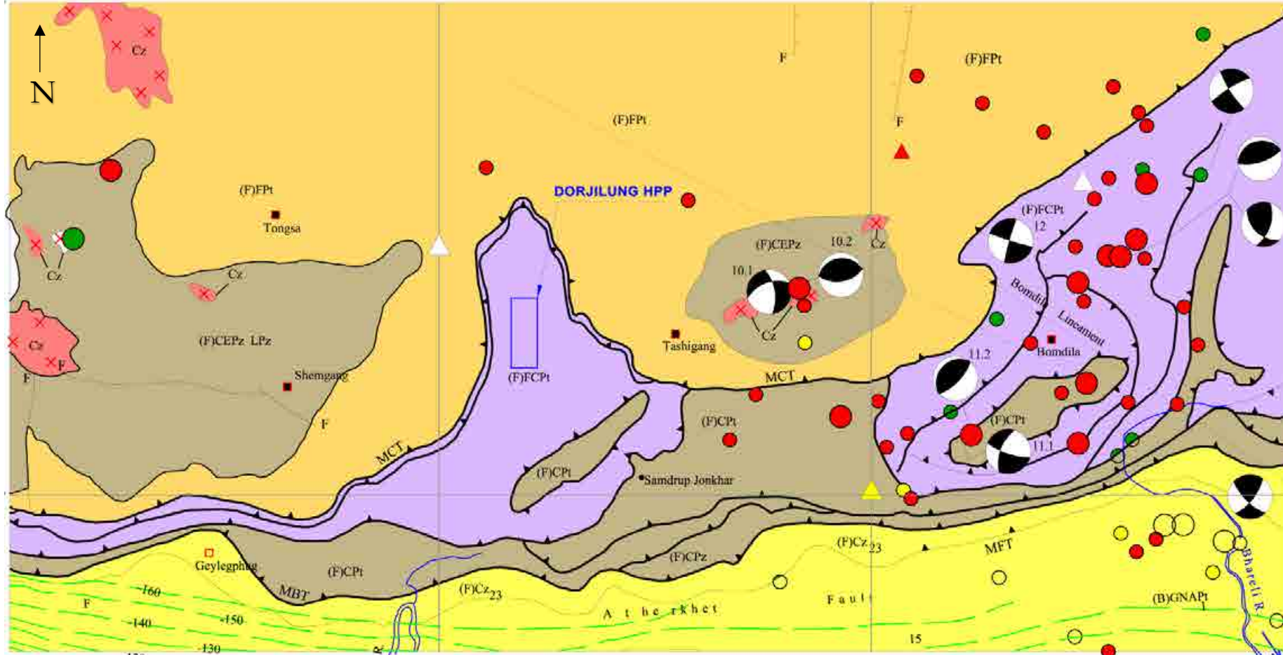
Figure 51: Seismotectonic map of the Project area (reproduced from DPR, 2016)
