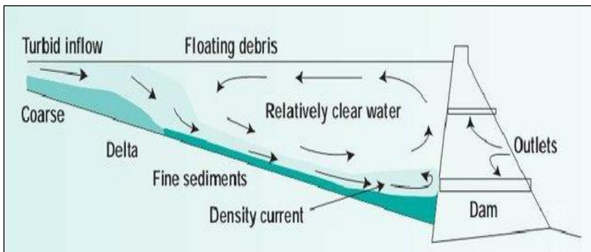
Figure 200: Conceptual diagram of sediment trapping in reservoirs (Ketelsen T. 2013)
