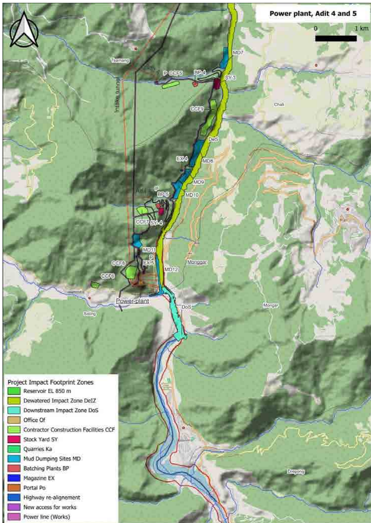
Figure 7: General Arrangement of Dorjilung HPP – Power plant, Adit 4 and 5
