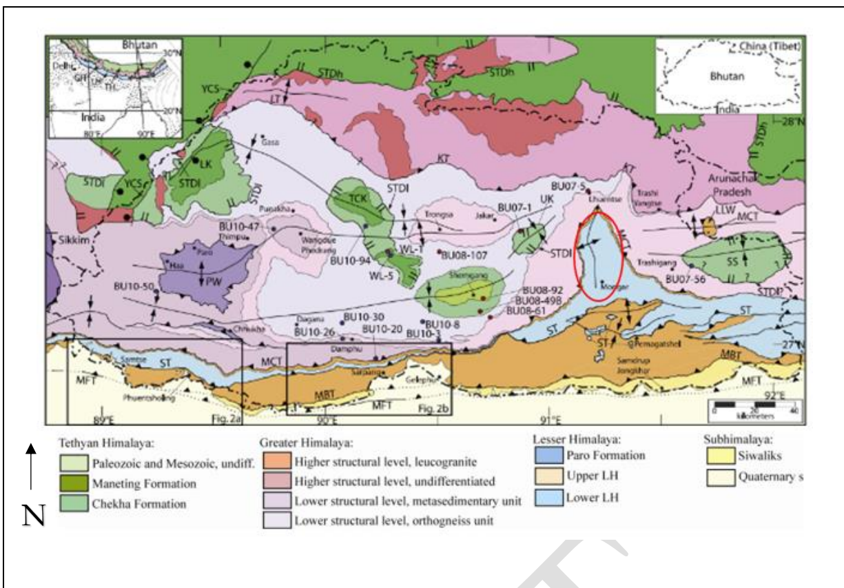
Figure 24: Geological map of Bhutan
