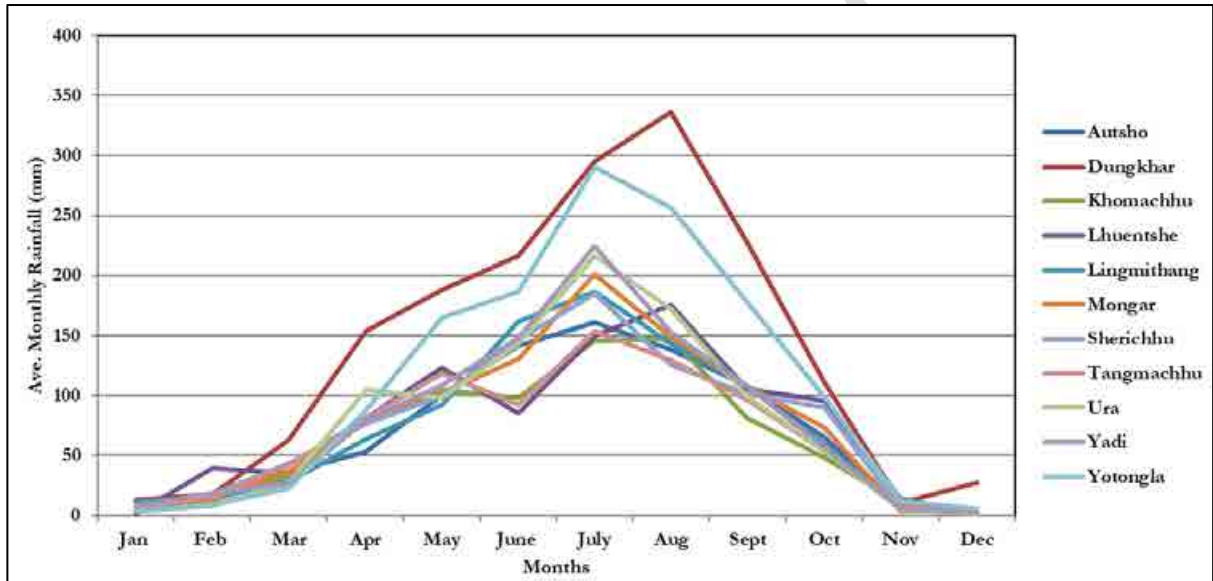
Figure 20: Average Monthly Rainfall in the Dorjilung catchment
