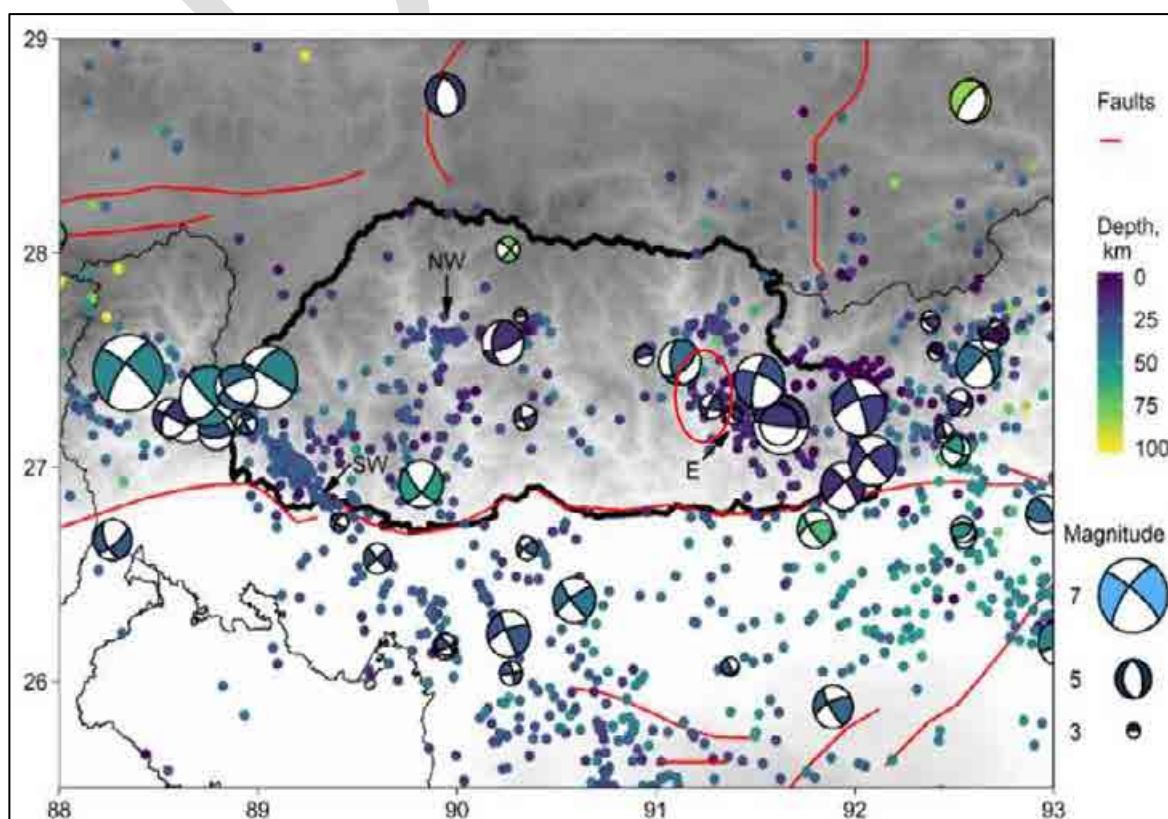
Figure 50: Geological setting of Bhutan (borders in thick line)
