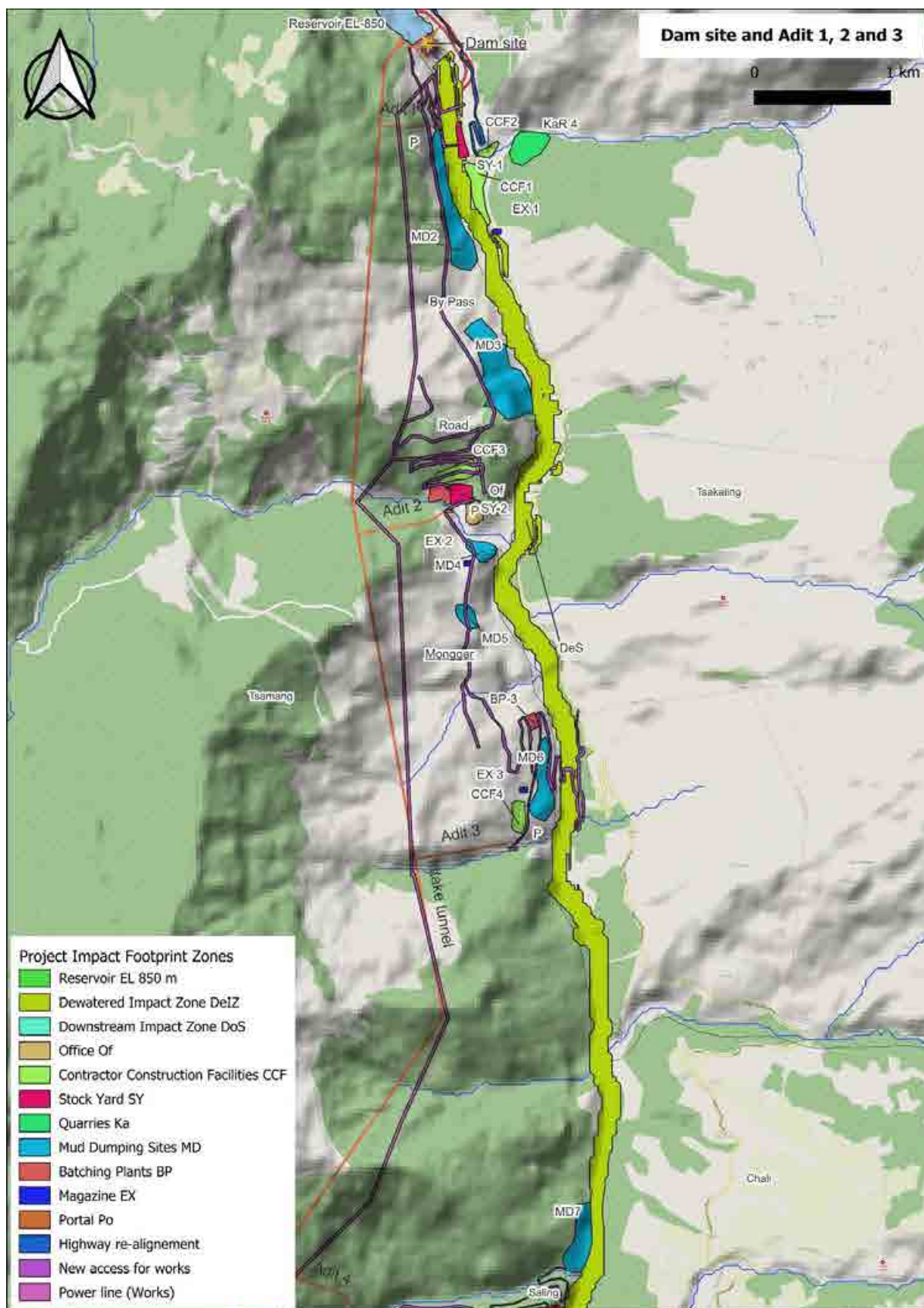
Figure 6: General Arrangement of Dorjilung HPP – Dam Site and Adit 1,2 & 3
