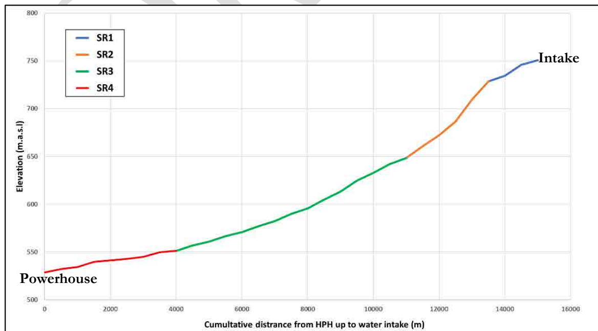
Figure 13: Longitudinal Profile of the Affected Reach of the Dorjilung HPP
