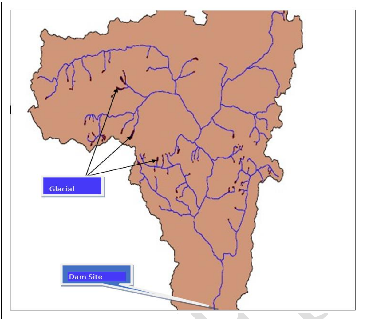
Figure 49: Dorjilung catchment model with identified glacial lakes
