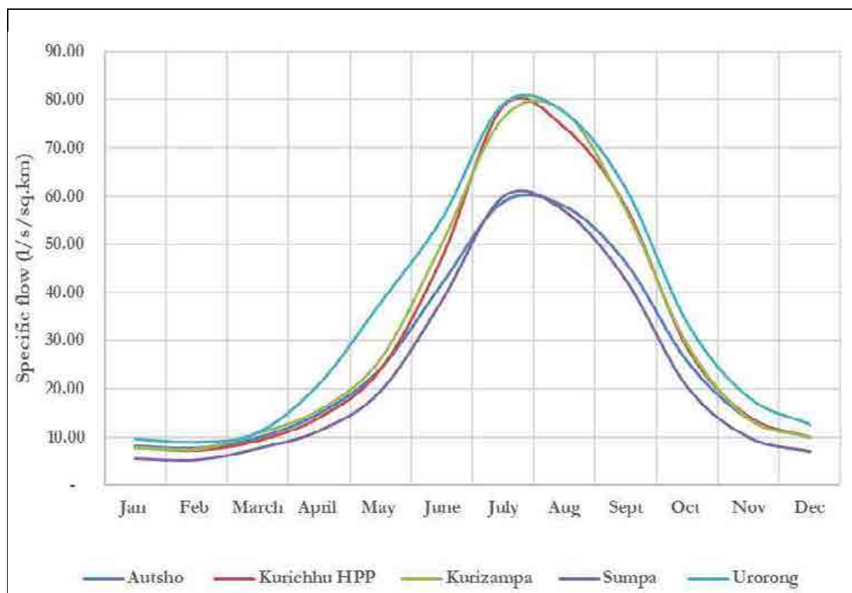
Figure 31: Monthly flows in the Kurichhu catchment
