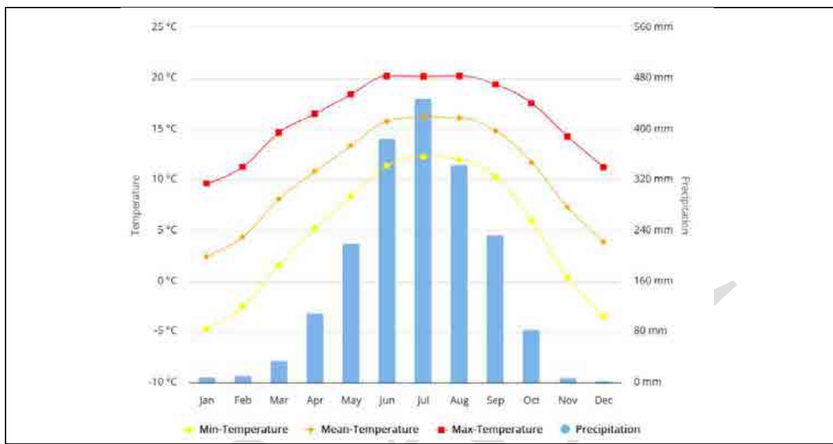
Figure 19: Climograph for Bhutan 1991-2020
