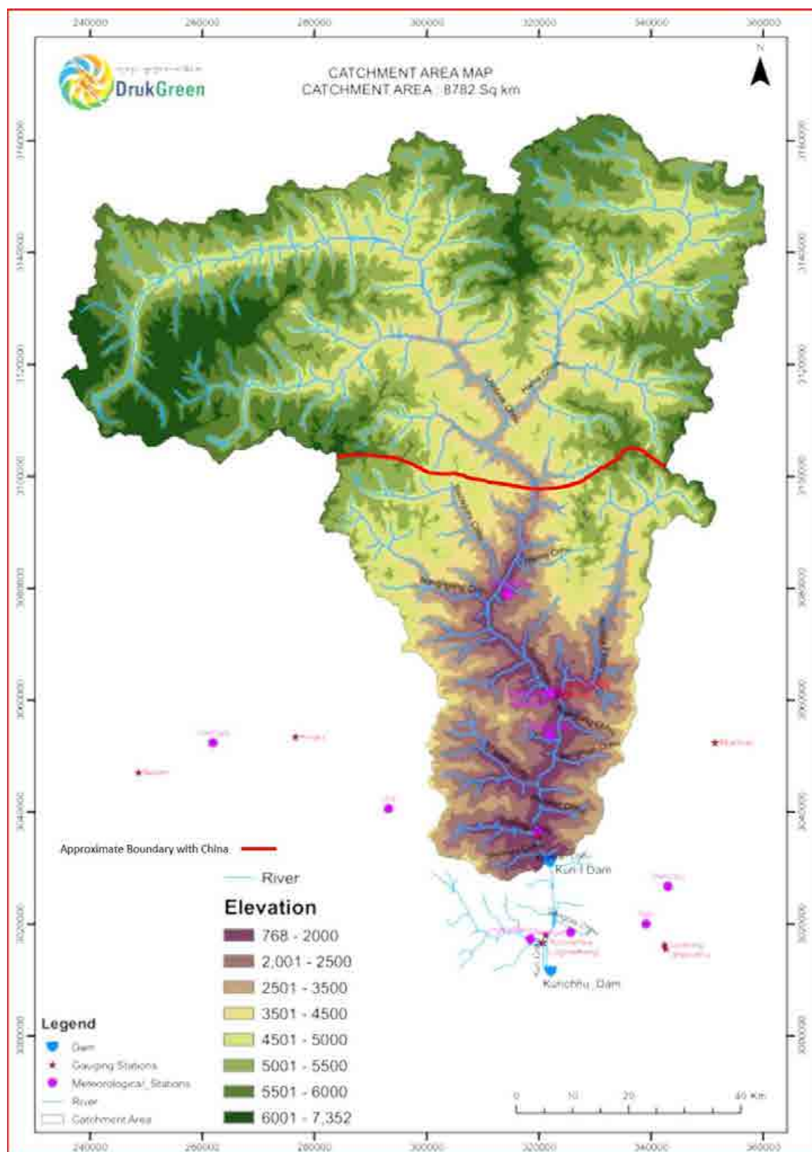
Figure 29: Catchment area of the Kurichhu River
