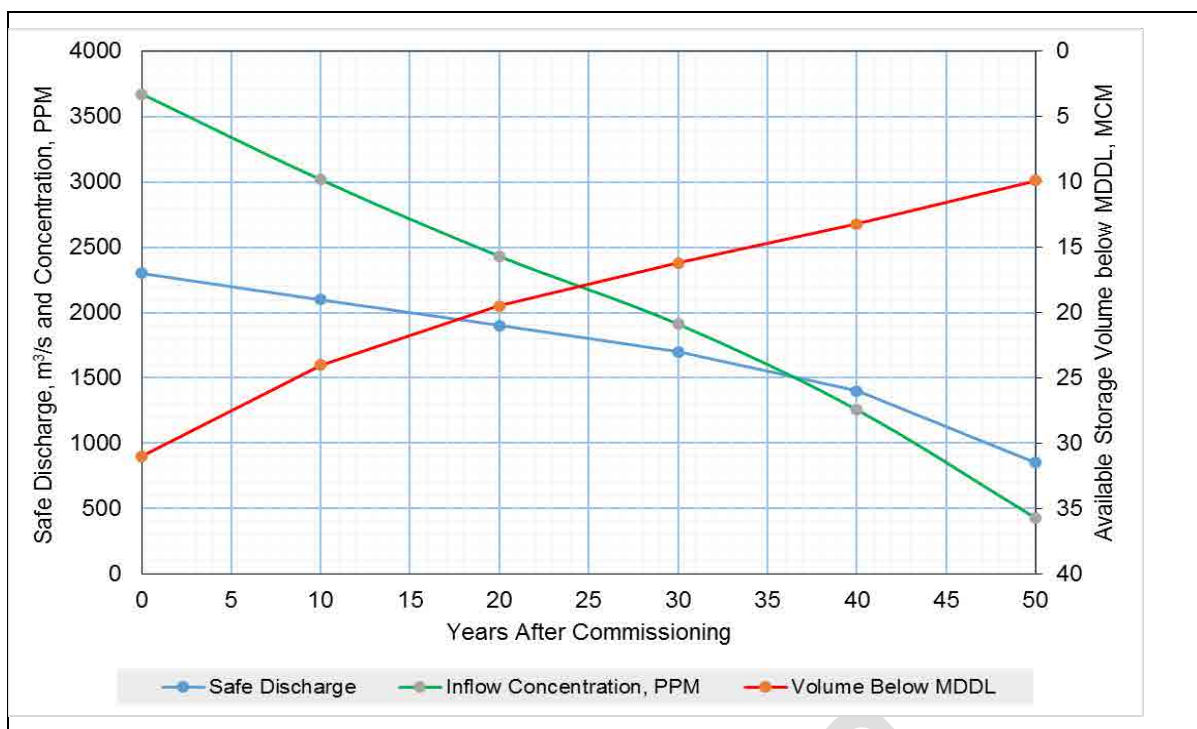
Figure 43: Plot of Safe Q with Available Storage Volume at MDDL and Concentration of Particle Size of 0.2mm at Reservoir Tip after different periods of reservoir operation
