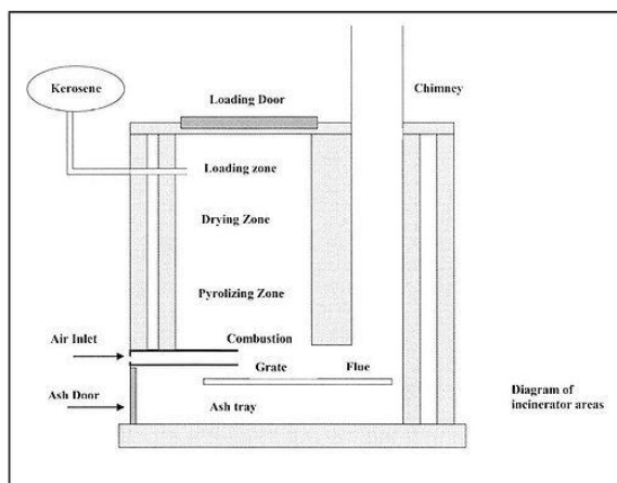
Figure 6-3 Incinerator Designs
