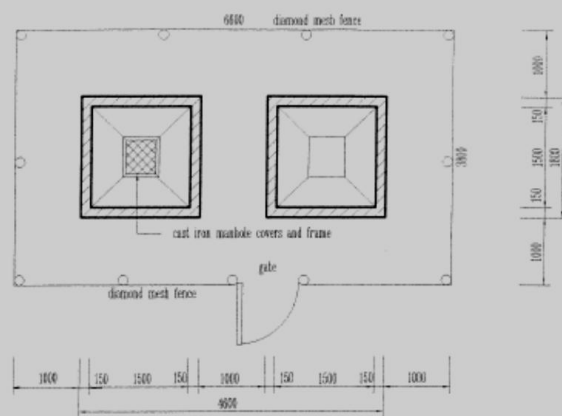
FLOOR PLAN
