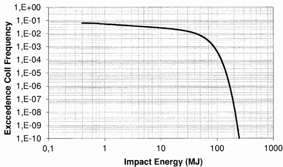
Figure 7.10 Infield Vessel Impact Energy Exceedance Spectra
