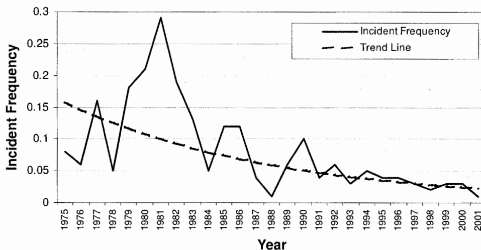
Figure 7.2 Infield Ship Collision Frequency with Fixed Installations
