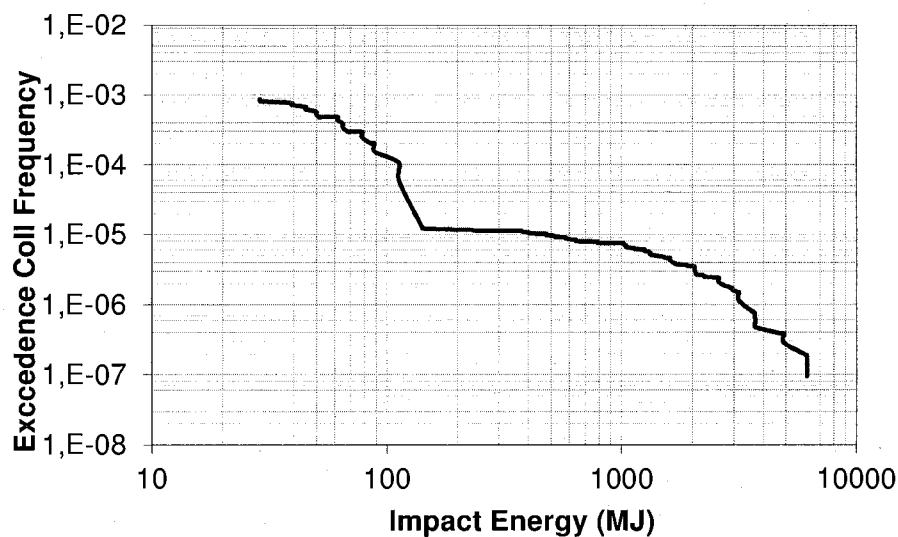
Figure 5.2 Passing Powered Impact Energy Spectrum for Banda
