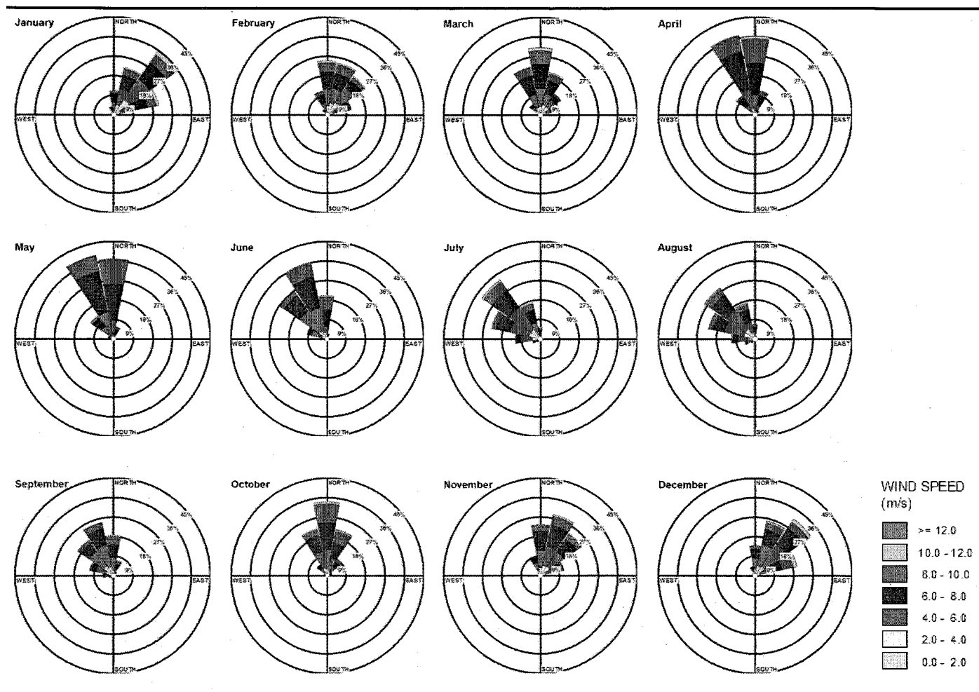
Figure 2.3 Monthly Wind Roses (direction wind blowing from) in the Banda Field Offshore Mauritania
