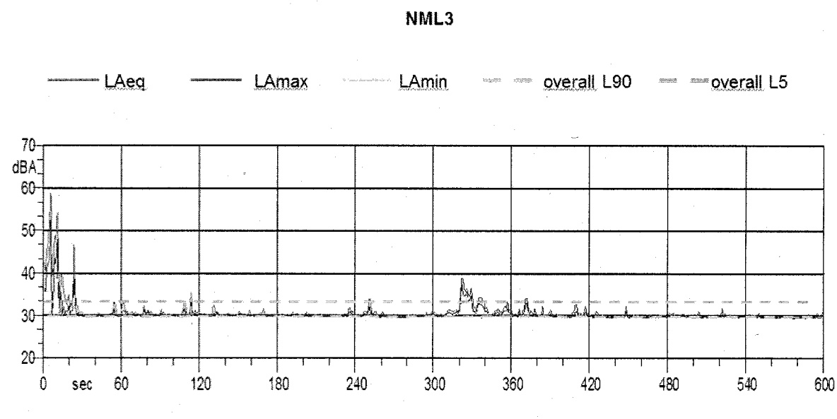
Figure 2.6 Receptor NML3
