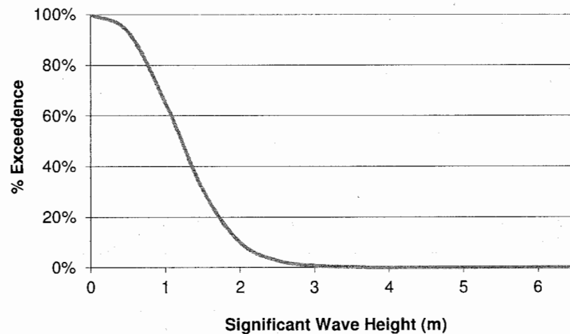
Figure 2.4 Annual Wave Height Exceedence Curve for the Banda Area (Ref. i)
