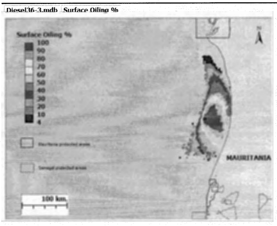
Figure 3.1 Diesel Spill: Probability of Visible Surface Oiling
