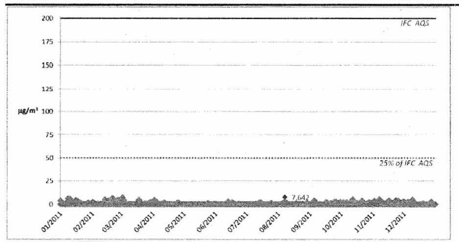
Figure 4.8 Time series of NO 2 hourly concentrations at the receptor NML9 (University)
