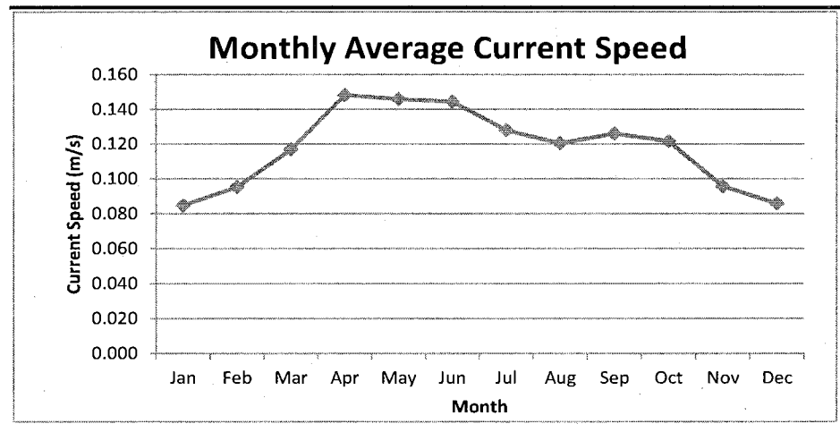
Figure 2.7 Monthly Average Surface Currents
