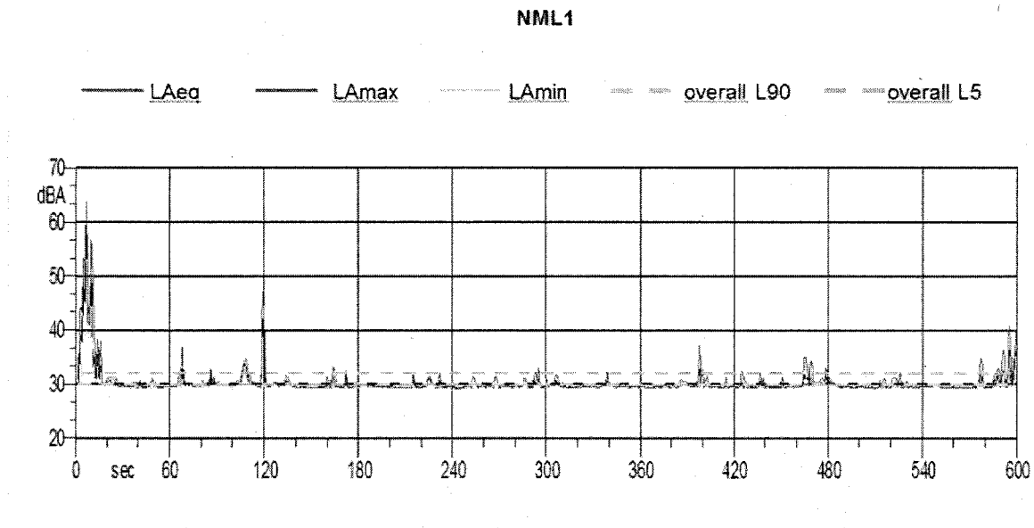
Figure 2.4 Receptor NML1
