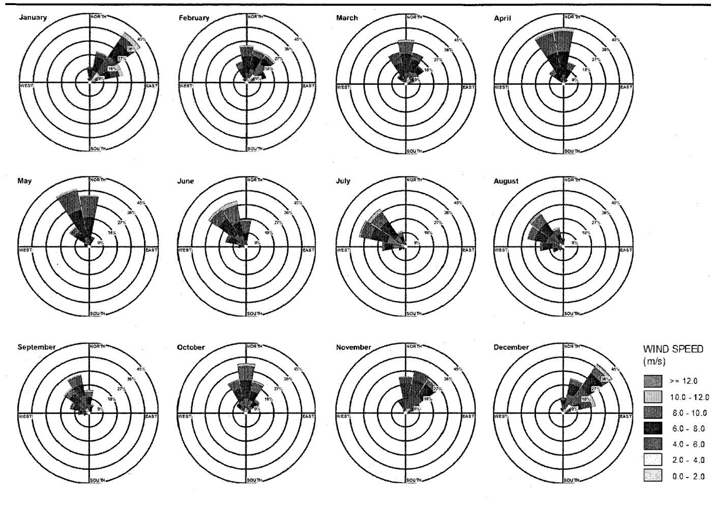
Figure 2.4 Monthly Wind Roses (direction wind blowing from) at Coastal Mauritania
