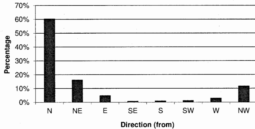
Figure 2.3 Annual Wind Direction Distribution for the Banda Area (Ref. i)
