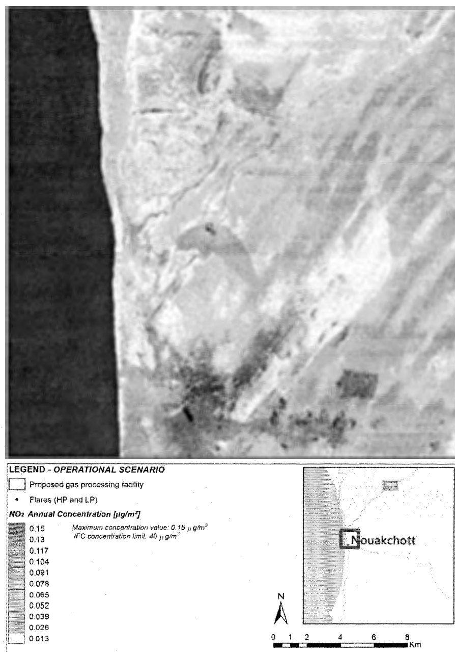
Figure 4.1 Operational Scenario: Predicted Annual Average Concentration for NO 2
