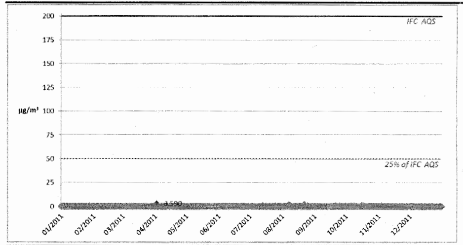
Figure 4.7 Time series of NO 2 hourly concentrations at the receptor NML8 (Settlement near Nouakchott- Nouadhibou road)
