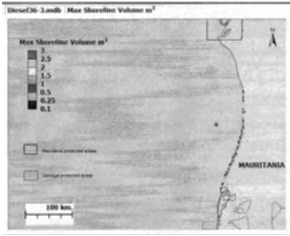
Figure 3.4 Diesel spill: Maximum Shoreline Oiling Volume
