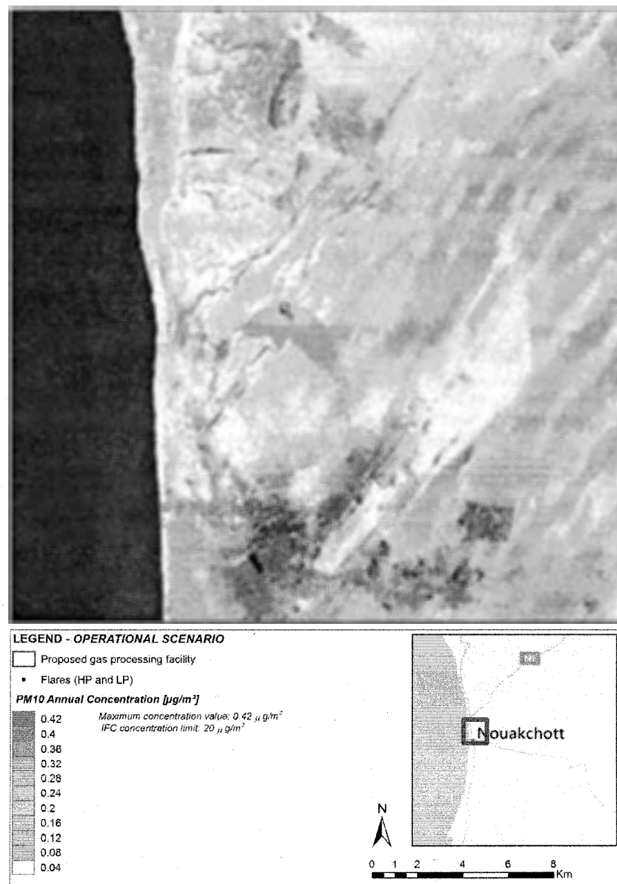
Figure 4.3 Operational Scenario: Predicted Annual Average Concentration for PM 10
