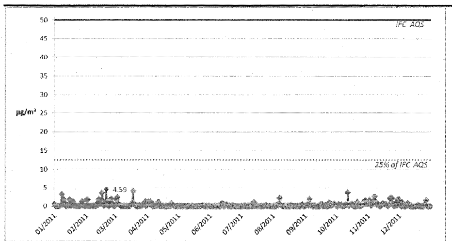
Figure 4.10 Time series of PM 10 daily concentrations at the receptor NML9 (University)
