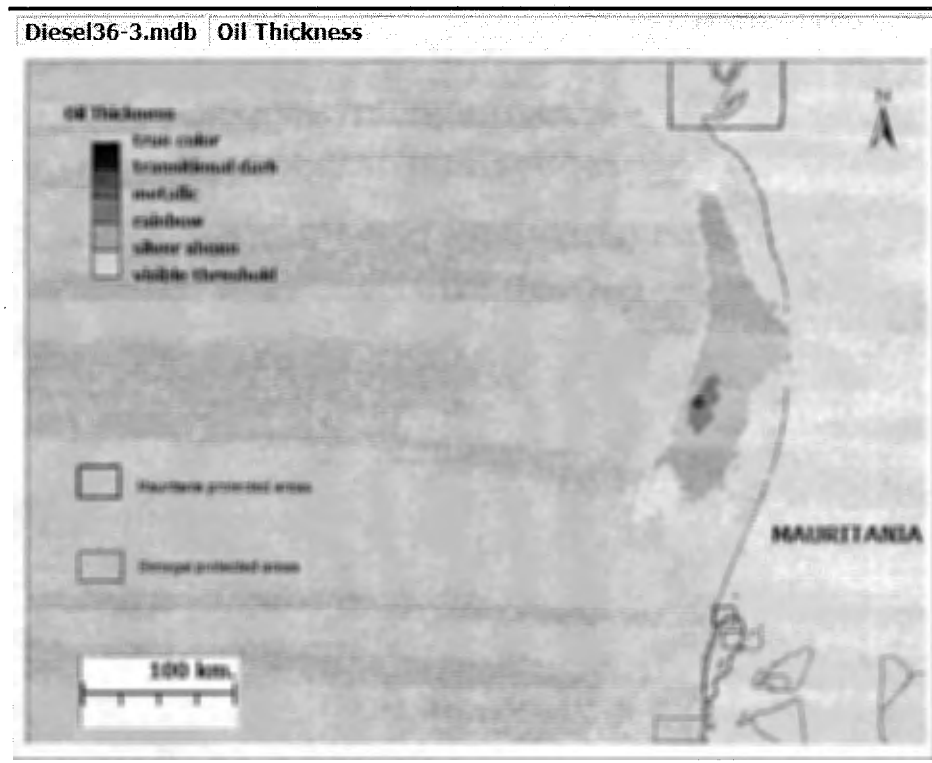
Figure 3.2 Diesel Spill: Maximum Oil Thickness
