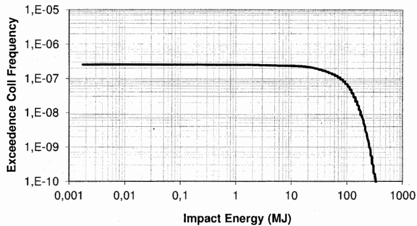
Figure 6.2 Passing Drifting Impact Energy Spectra
