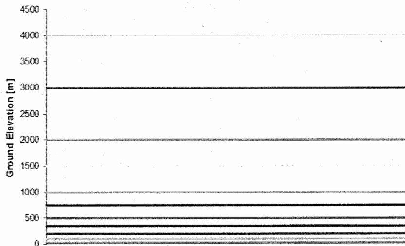
Figure 3.4 Models Vertical Resolution
