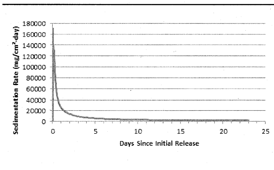
Figure 4.6 Maximum Sedimentation Rates over Time
