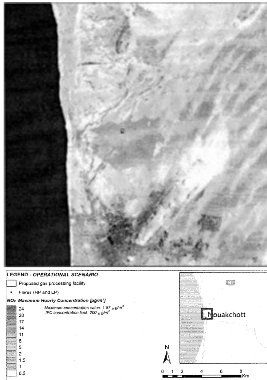
Figure 4.2 Operational Scenario: Maximum Predicted Hourly Concentration for NO 2
