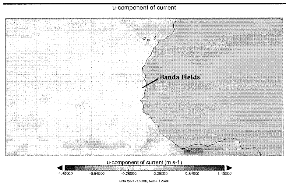
Figure 2.8 Example CFSR east-west Component of the Current for 1 June 1996 midnight, 5 m depth (positive is to the east)
