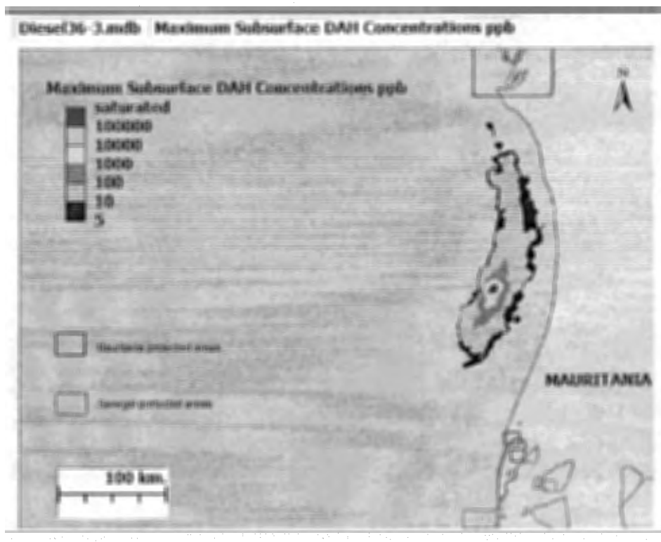
Figure 3.5 Diesel Spill: Maximum Dissolved Aromatic Hydrocarbon Concentrations
