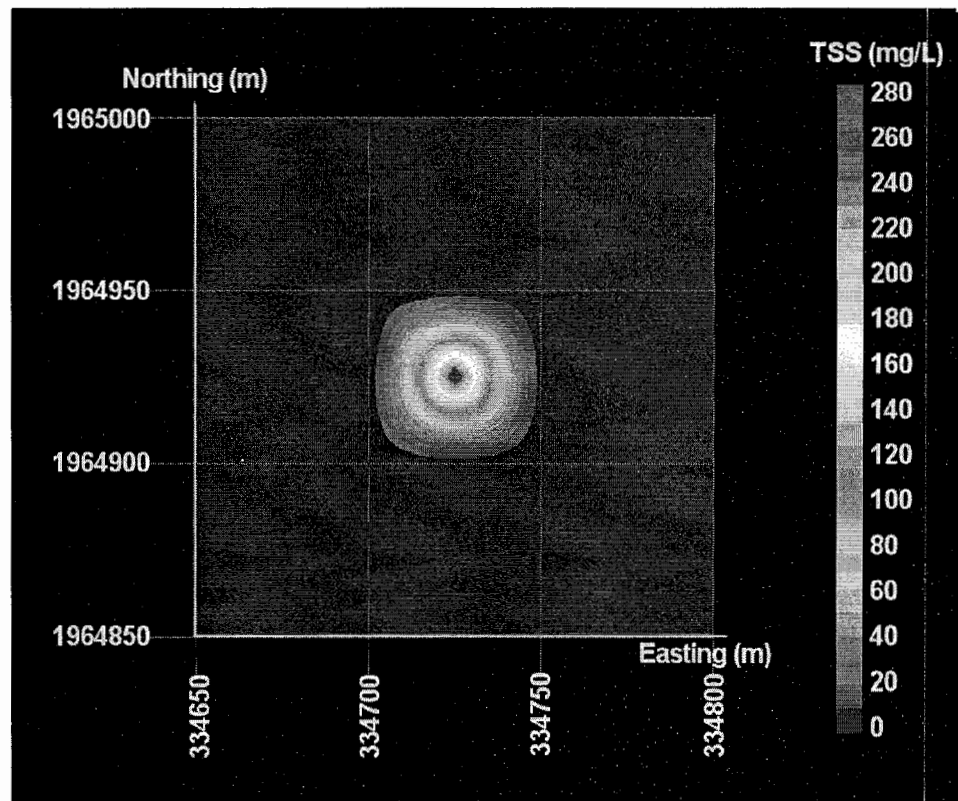
Figure 4.4 Maximum TSS Concentration Increase over Ambient Conditions near Seabed
