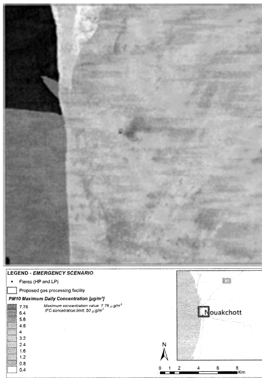
Figure 4.6 Emergency Scenario: Maximum Predicted Daily Concentration for PM 10
