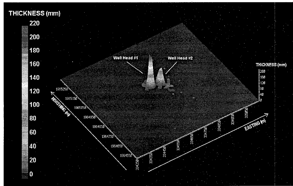
Figure 4.2 Bottom Deposition Thickness - 3-D Perspective (vertically exaggerated)
