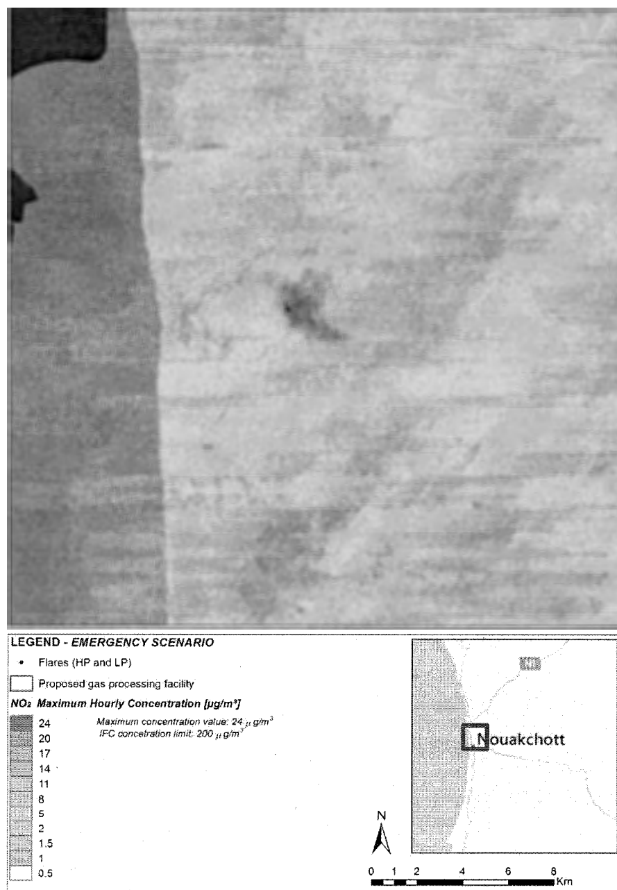
Figure 4.5 Emergency Scenario: Maximum Predicted Hourly Concentration for NO 2
