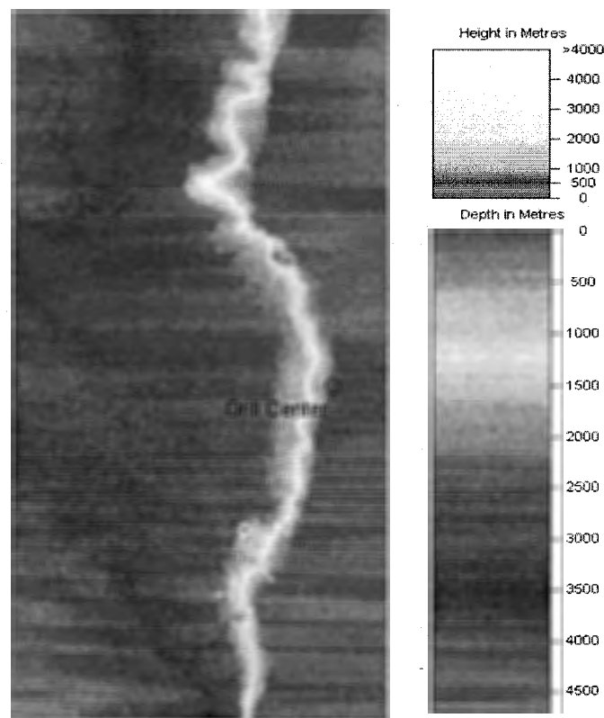
Figure 2.2 GEBCO Bathymetry Map
