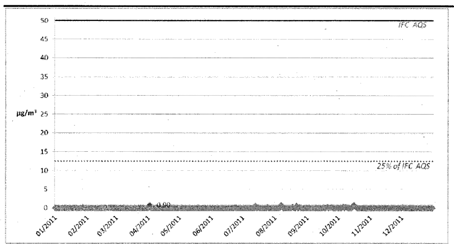
Figure 4.9 Time series of PM 10 daily concentrations at the receptor NML8 (Settlement near Nouakchott- Nouadhibou road)
