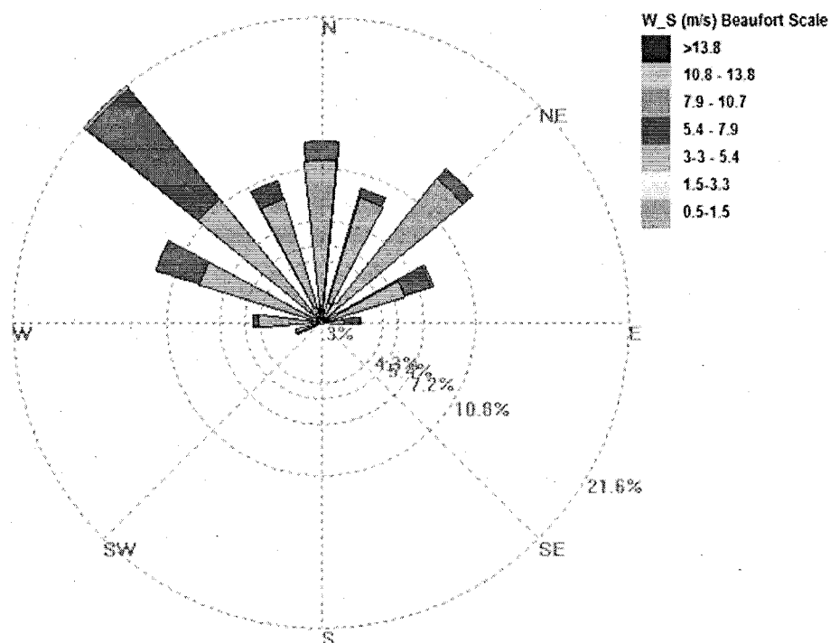
Figure 3.5 Wind Rose Extracted from the CALMET run (2011) at the Flares Location
