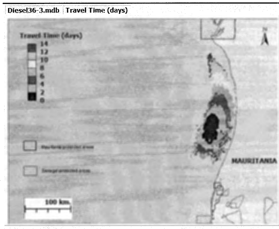
Figure 3.6 Diesel Spill: Travel Time for Visible Oil
