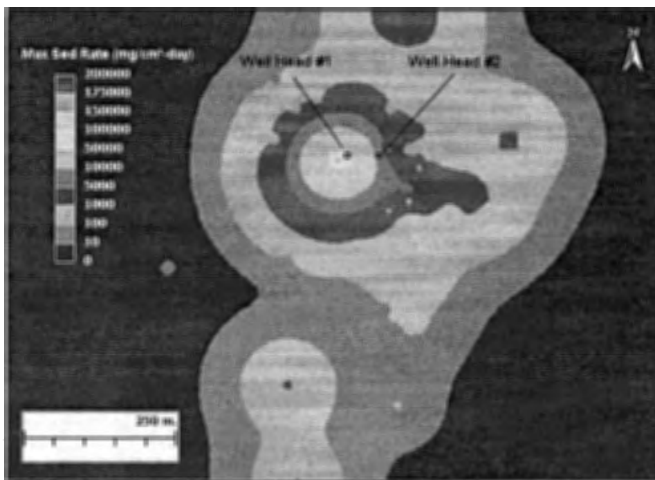
Figure 4.5 Maximum Sedimentation Rate
