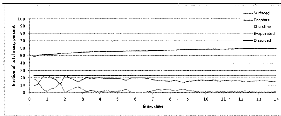
Figure 3.8 Mass Balance Plot: Diesel Spill
