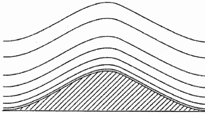
Figure 3.3 Concept of Terrain Following Vertical Coordinate System
