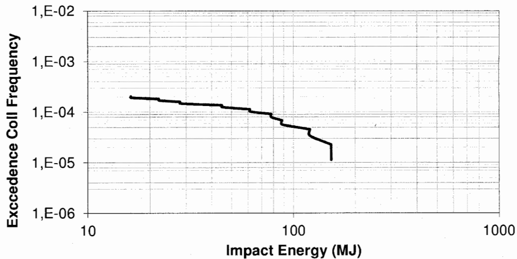
Figure 8.5 Passing Fishing Impact Energy Spectrum for Banda
