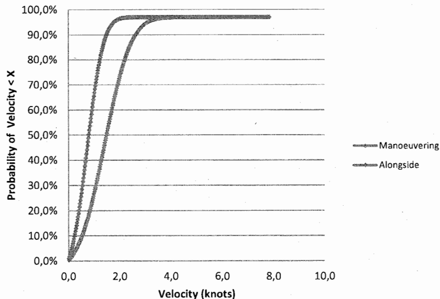
Figure 7.3 Infield Vessel Velocity Profile
