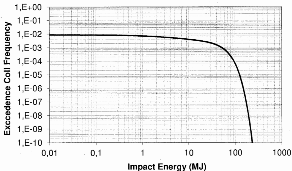
Figure 7.9 Combined Supply Vessel Annual Collision Frequency Infield Vessel Impact Energy Exceedence Spectra for Supply vessel performing ERRV Duties
