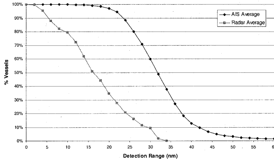
Figure 9.1 AIS versus Radar Detection Comparison (Anatec live trials)
