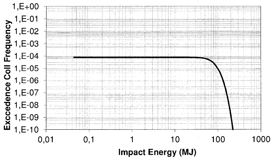
Figure 7.8 Annual Collision Frequency On Approach (Powered) Infield Vessel Impact Energy Exceedence Spectra for Supply vessel performing ERRV Duties
