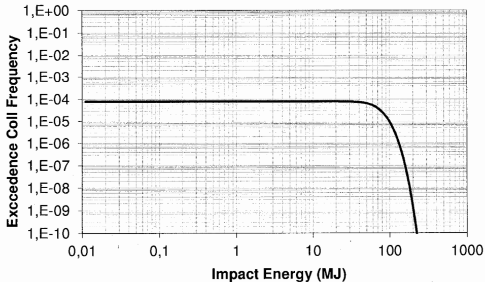
Figure 7.5 Annual Collision Frequency On Approach (Powered) Infield Vessel Impact Energy Exceedence Spectra for supply vessels
