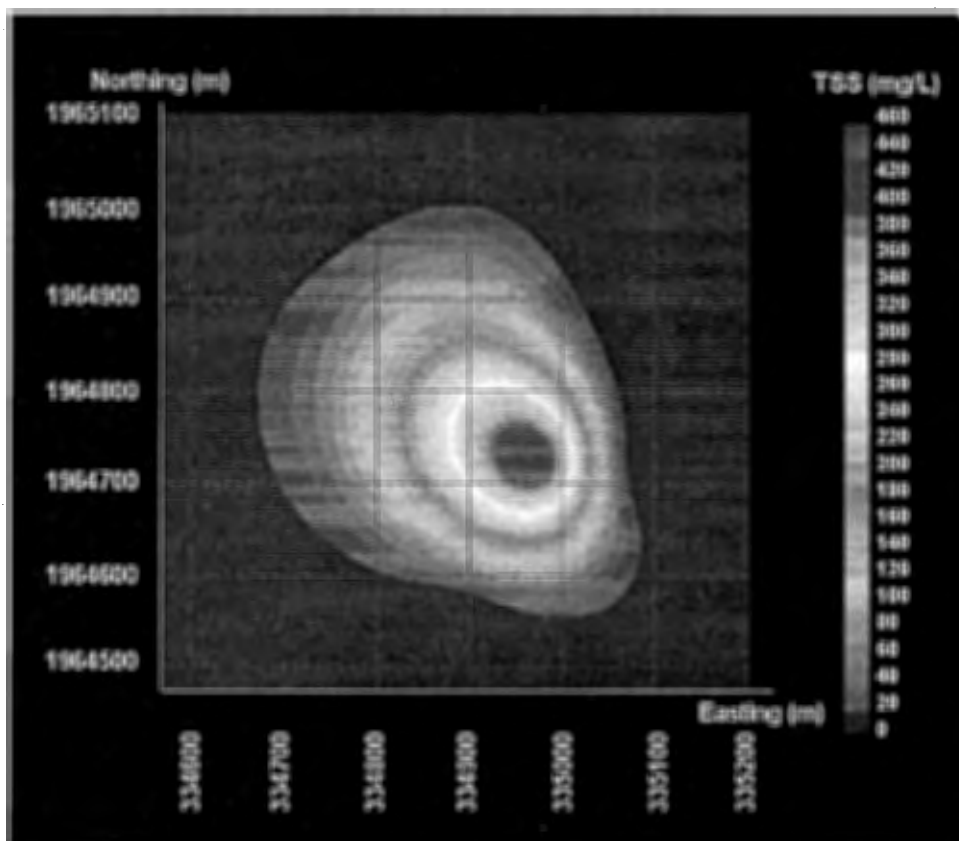
Figure 4.3 Maximum TSS Concentration Increase over Ambient Conditions near Surface
