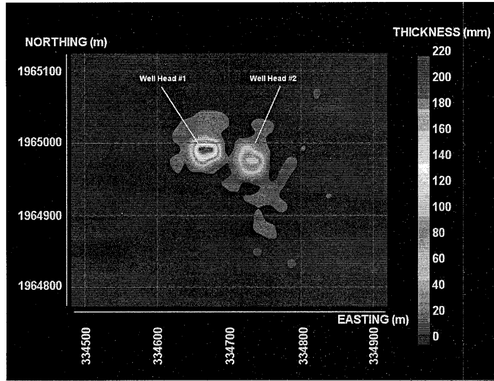
Figure 4.1 Bottom Deposition Thickness
