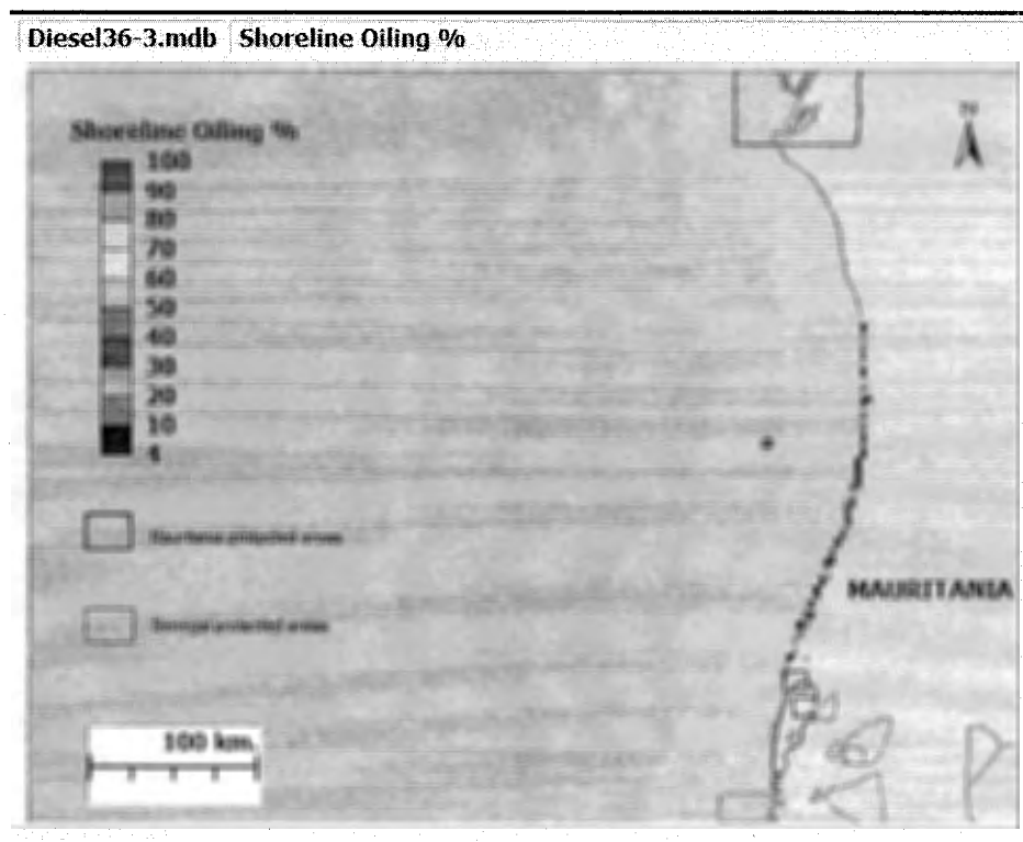
Figure 3.3 Diesel spill: Probability of Shoreline Oiling
