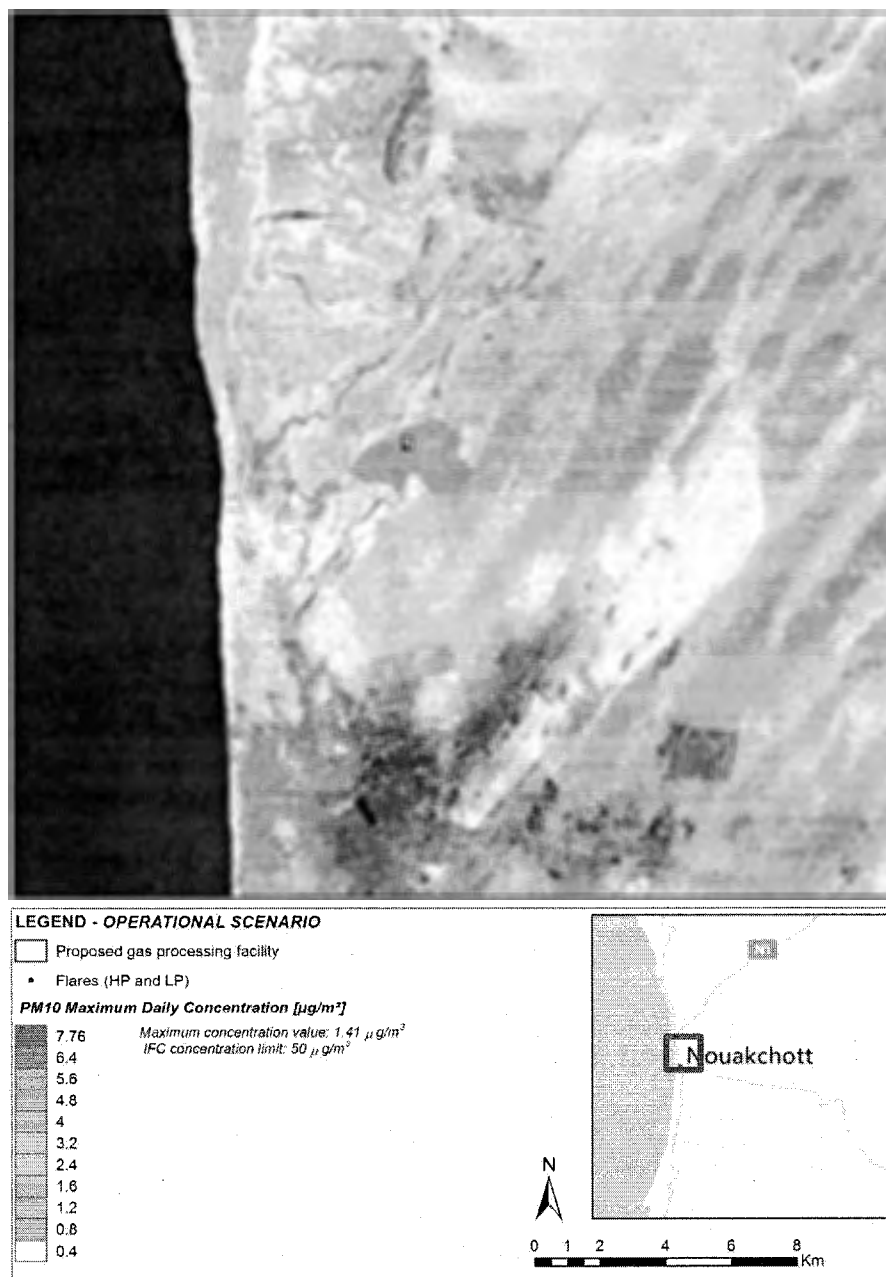
Figure 4.4 Operational Scenario: Maximum Predicted Daily Concentration for PM 10
