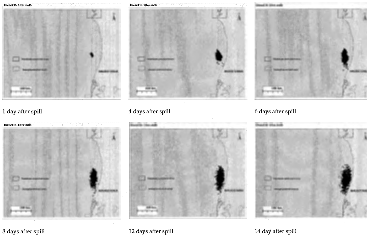
Figure 3.7 Example of the Evolution of a 1,200 m 3 Diesel Spill during 2 Weeks
