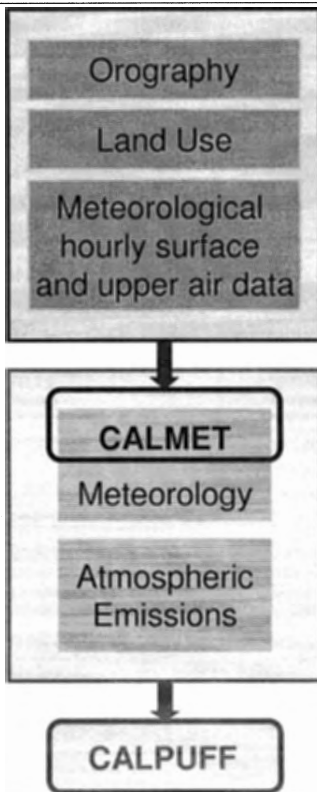
Figure 3.1 CALPUFF Modelling System Inputs
