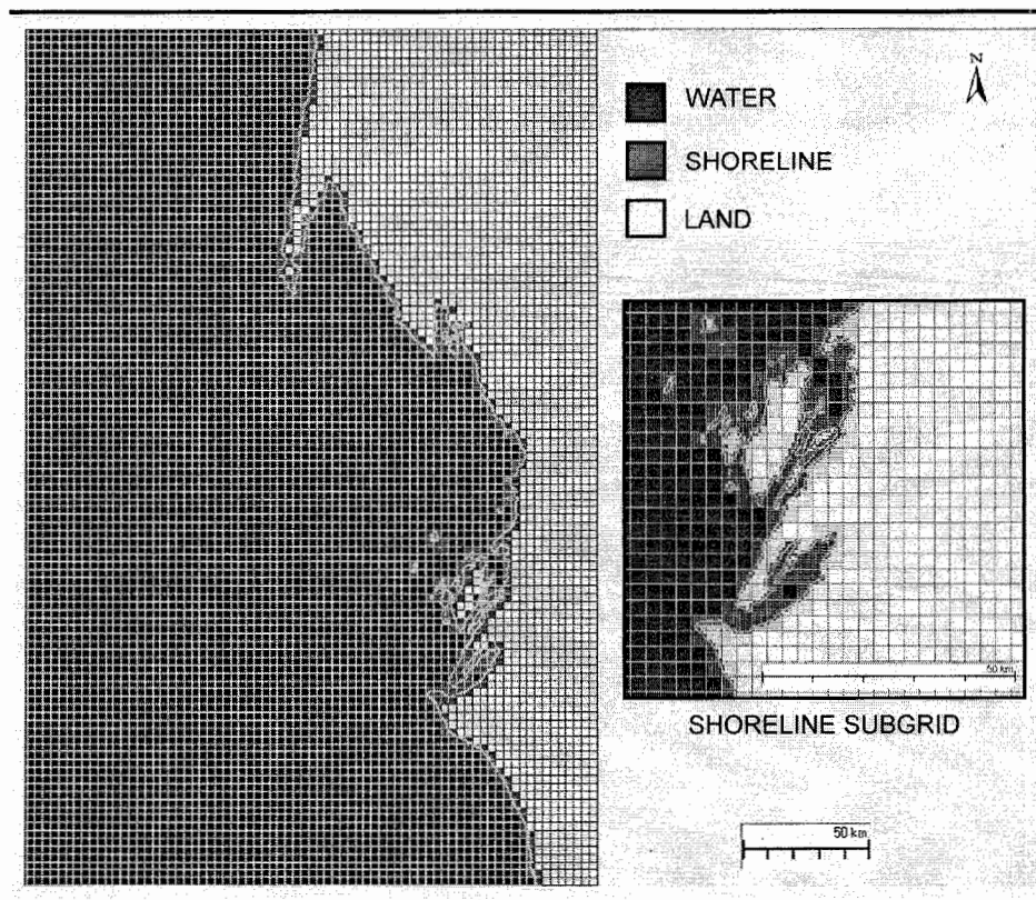
Figure 2.1 Oil Spill Grid Excerpt and Detail of Subgrid
