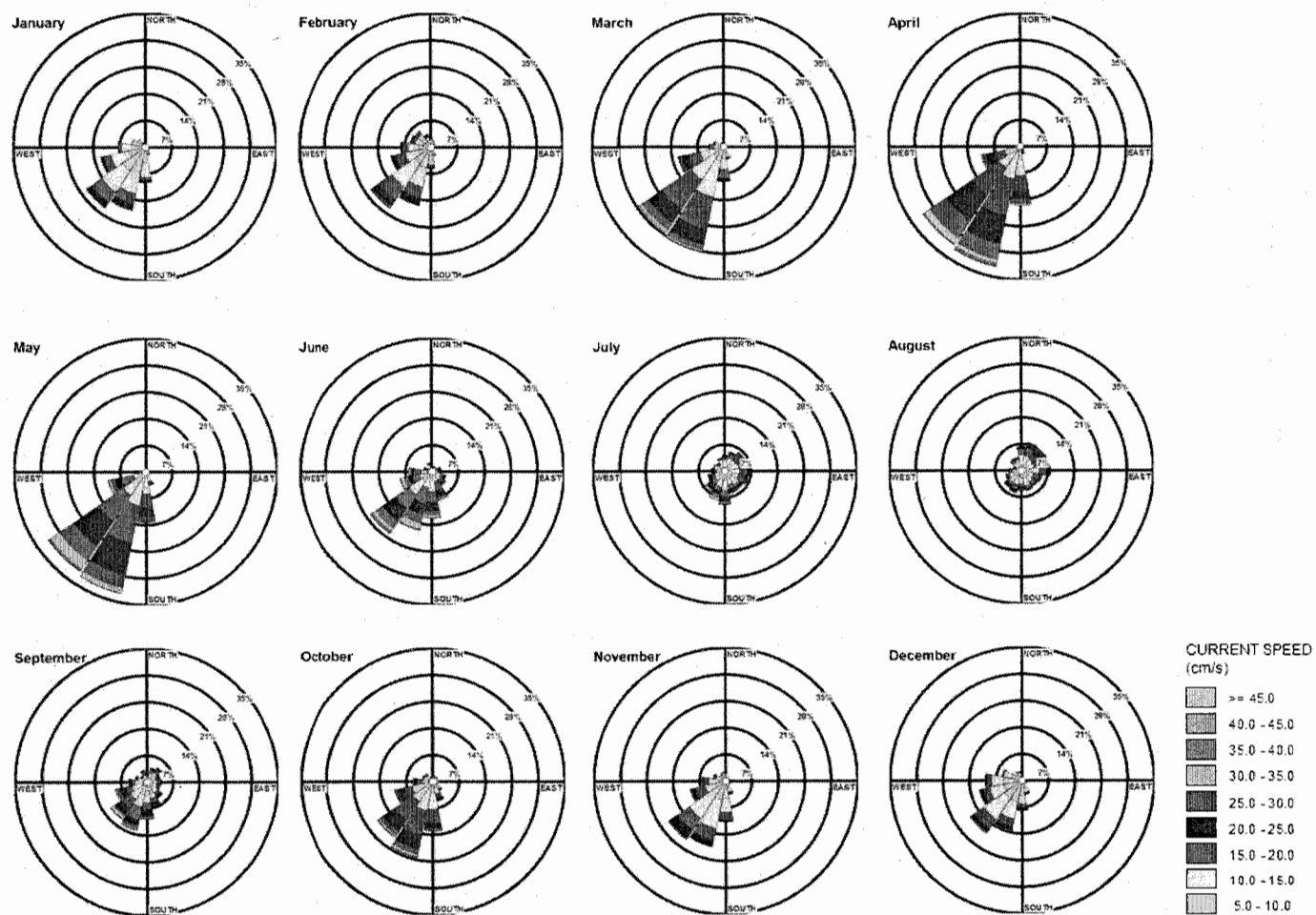
Figure 2.6 Monthly Current Roses (direction current travelling to) in the Banda Field Offshore Mauritania (1995-2001)
