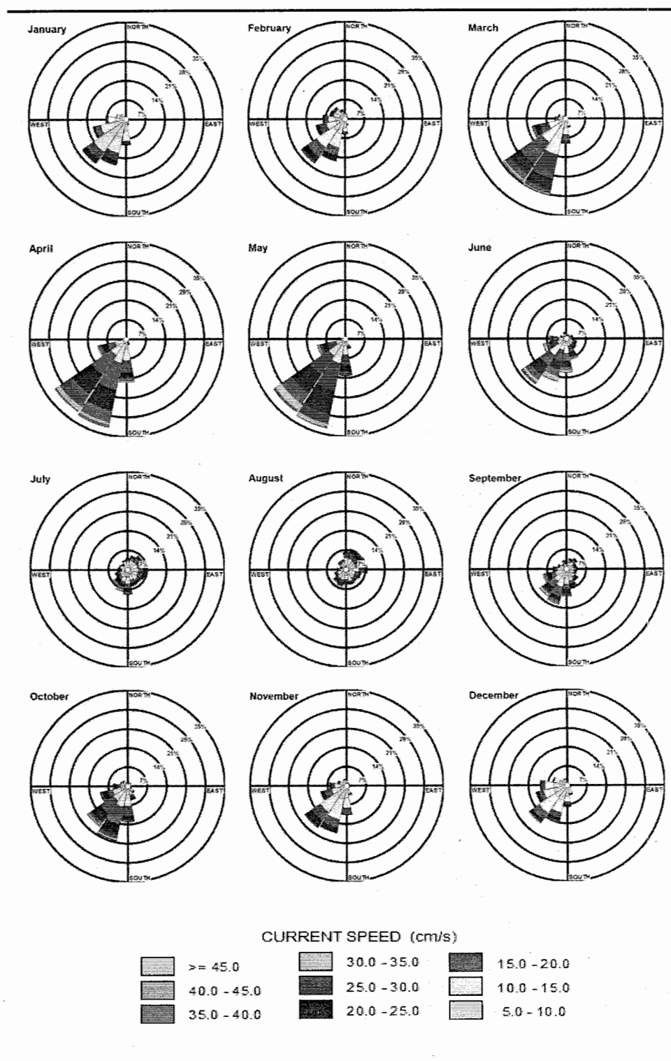
Figure 2.2 Monthly Current Roses (direction Current Traveling to) in the Banda Fields offshore Mauritania (1995-2001)
