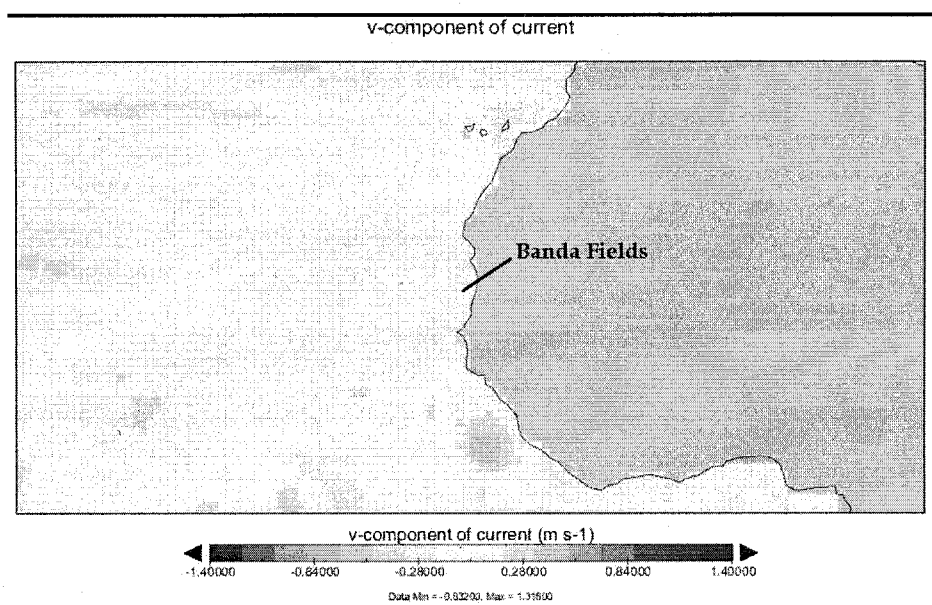
Figure 2.9 Example CFSR north-south Component of the Current for 1 June 1996 midnight, 5 m depth (positive is to the north)
