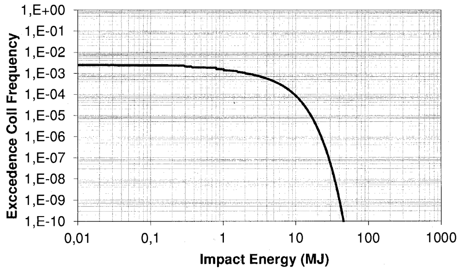
Figure 7.7 Annual Collision Frequency (Manoeuvring/ Alongside/ Drifting) Infield Vessel Impact Energy Exceedence Spectra for Supply vessel performing ERRV Duties
