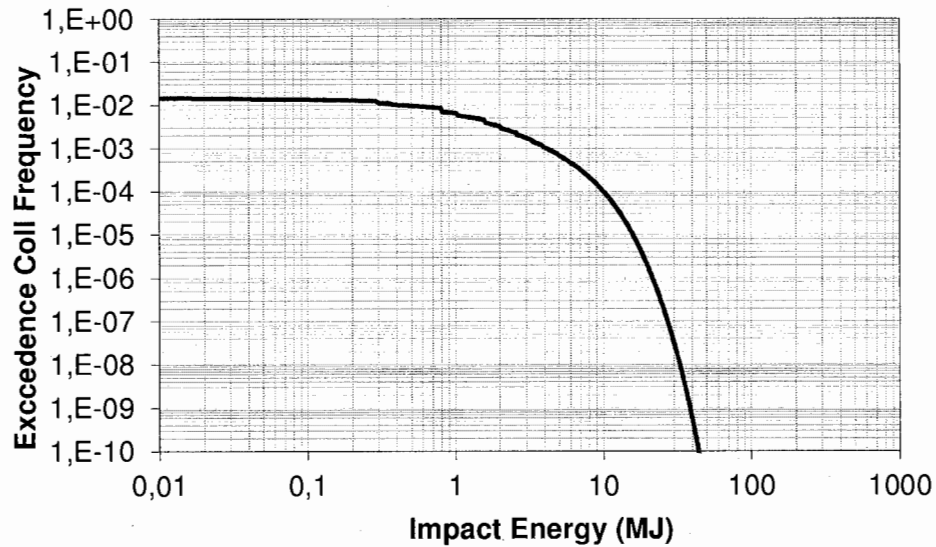
Figure 7.4 Annual Collision Frequency (Manoeuvring/ Alongside/ Drifting) Infield Vessel Impact Energy for supply vessels Exceedence Spectra
