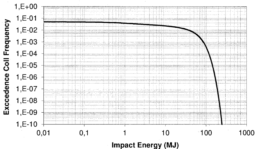
Figure 7.6 Combined Supply Vessel Annual Collision Frequency Infield Vessel Impact Energy Exceedence Spectra for supply vessels
