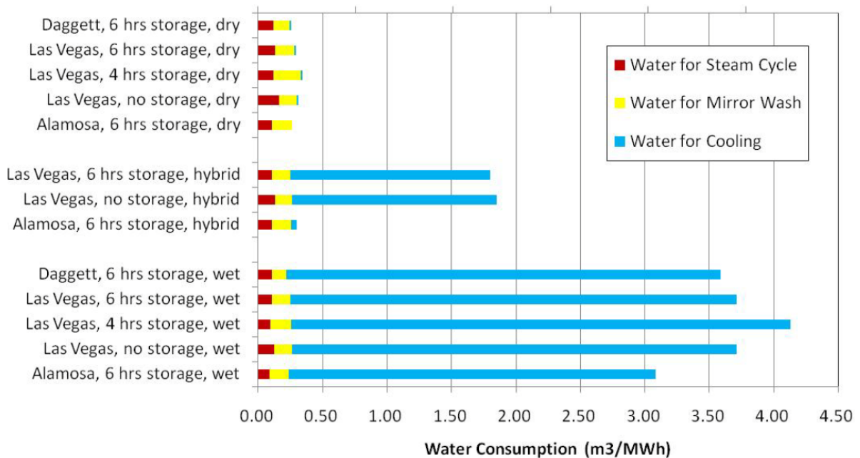
Figure 11-3 Water use of Parabolic CSP plants by different cooling options
