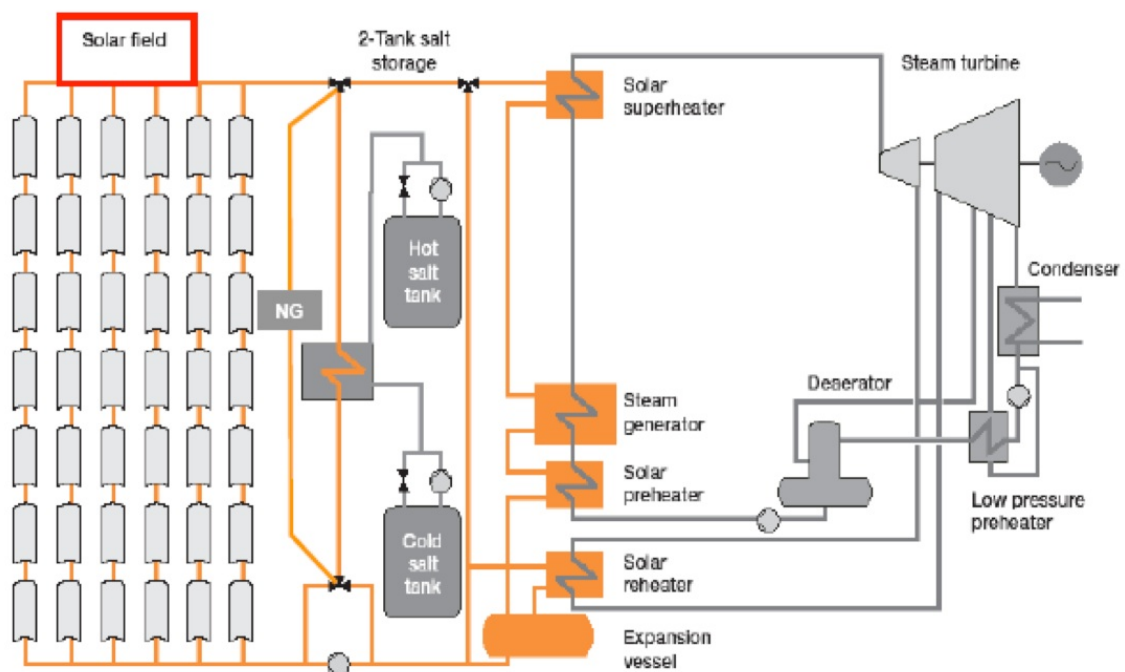
Figure 2 7 Basic Plant Process Sketch
