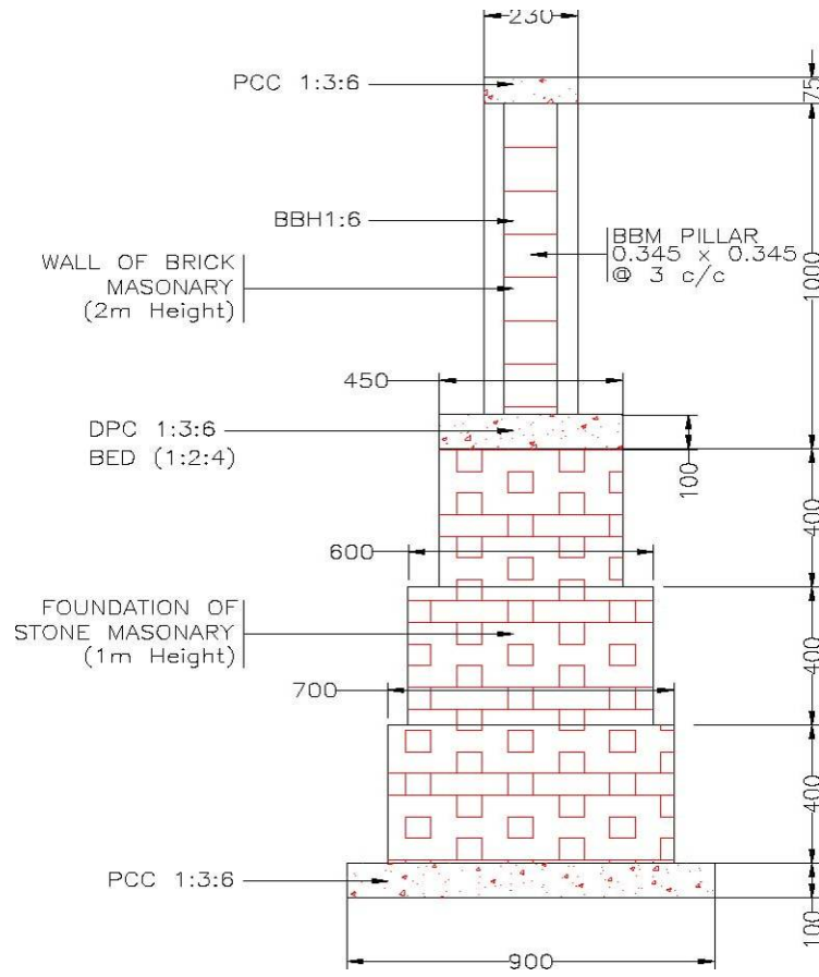
Figure 1. Typical Cross Section of a Noise Barrier
