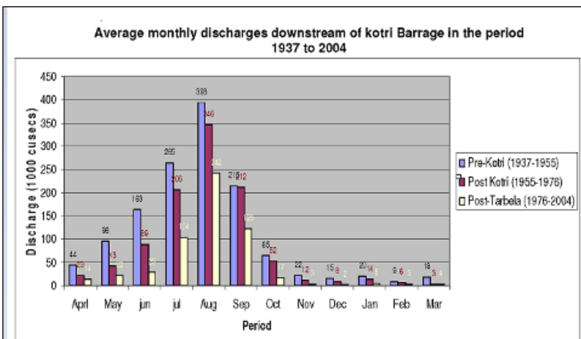
Figure 8: Monthly Discharges Downstream of Kotri Barrage
