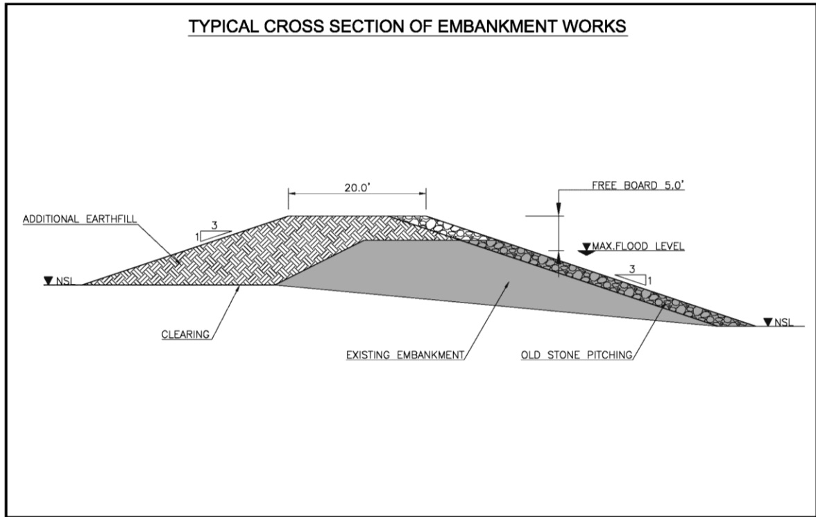
Figure 3: Typical Cross-Section
