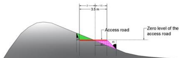
Figure 2.6: Typical Designs of Access Roads
