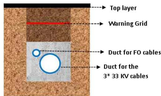
Figure 2.4: Typical Designs of 33 kV UGC cable trench
