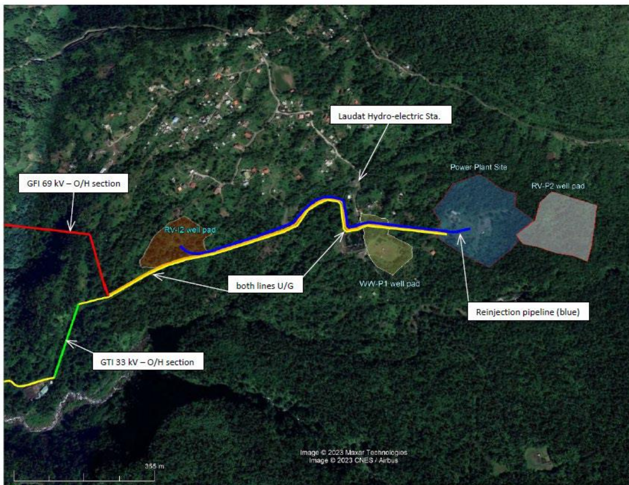
Figure 2.9: Locations of Associated Facilities
