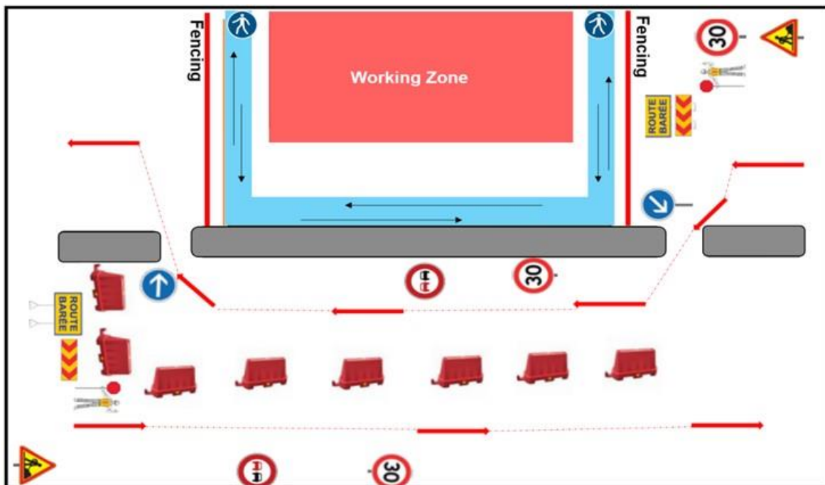
Figure 5.1. Traffic Management at the Construction Sites
