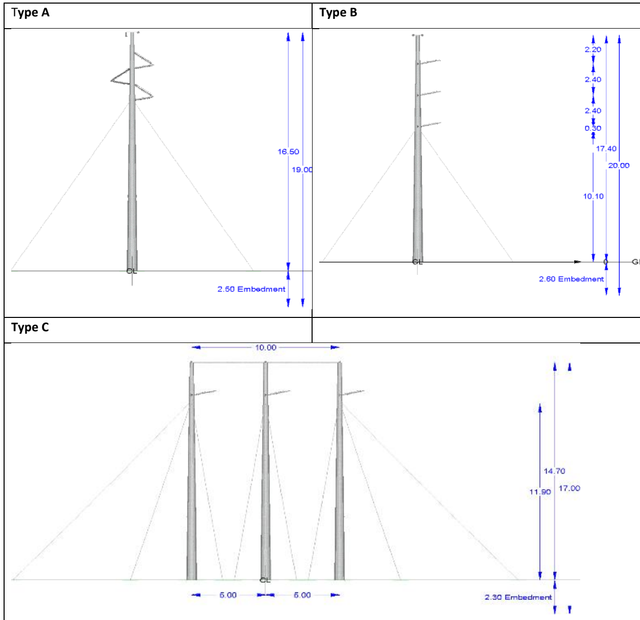
Figure 2.3: Typical Designs of Type A, B and C Structures
