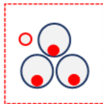
Figure 2.5: Typical Designs of 33 kV UGC cable trench
