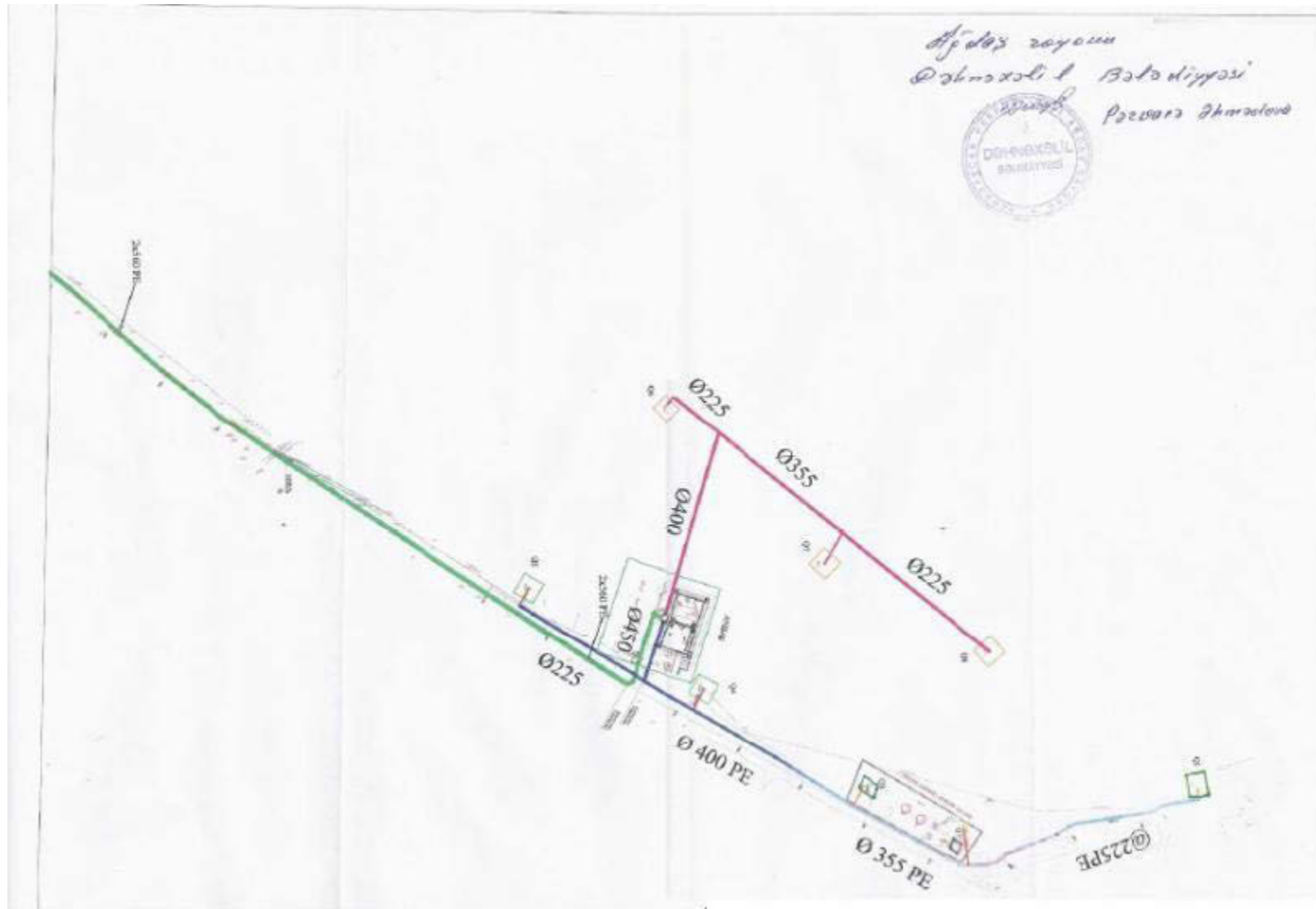
Map 8: Layout Plan of Well Field at Dehne
