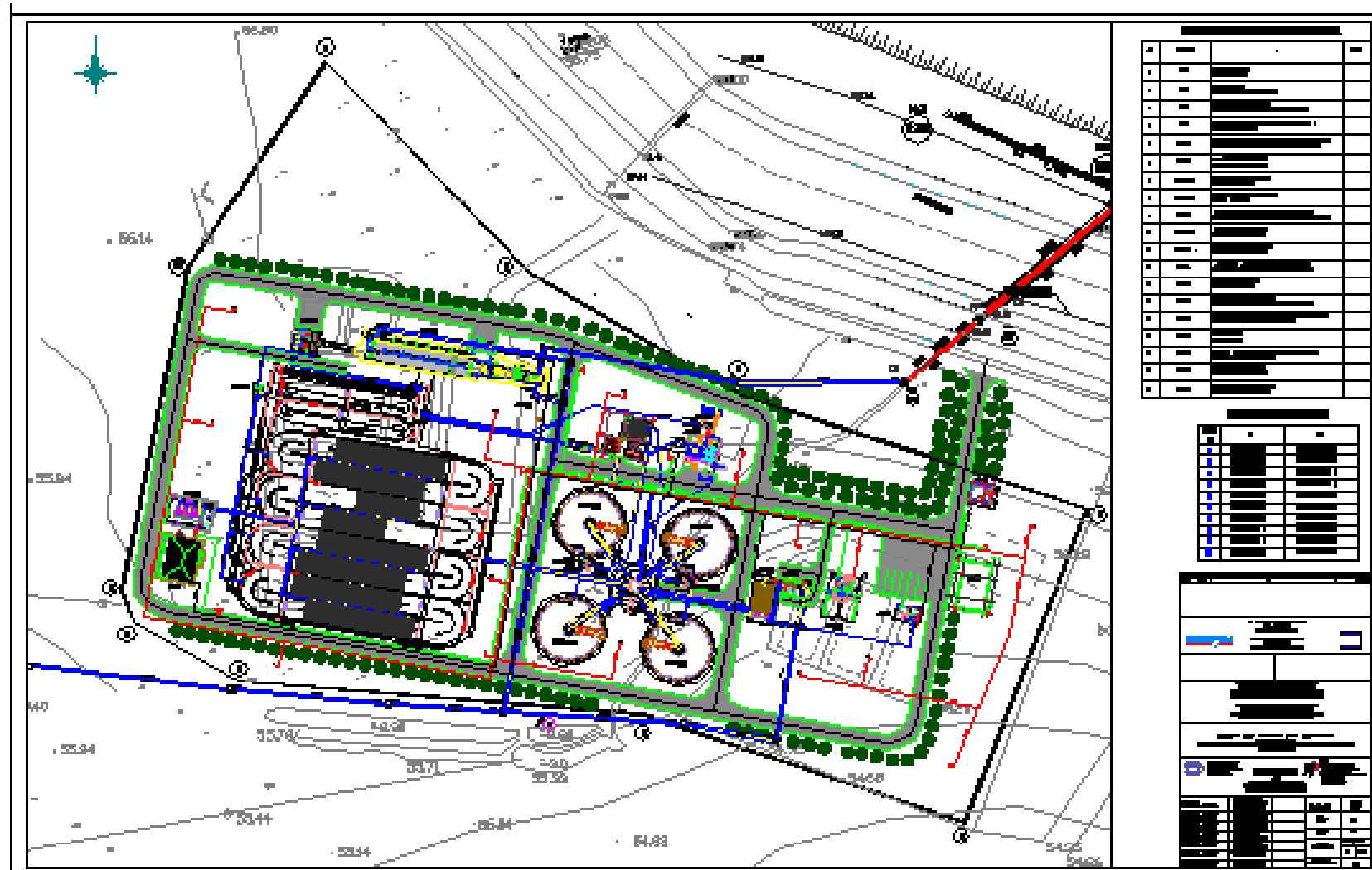
Map 10: Layout Plan of Wastewater Treatment Plant
