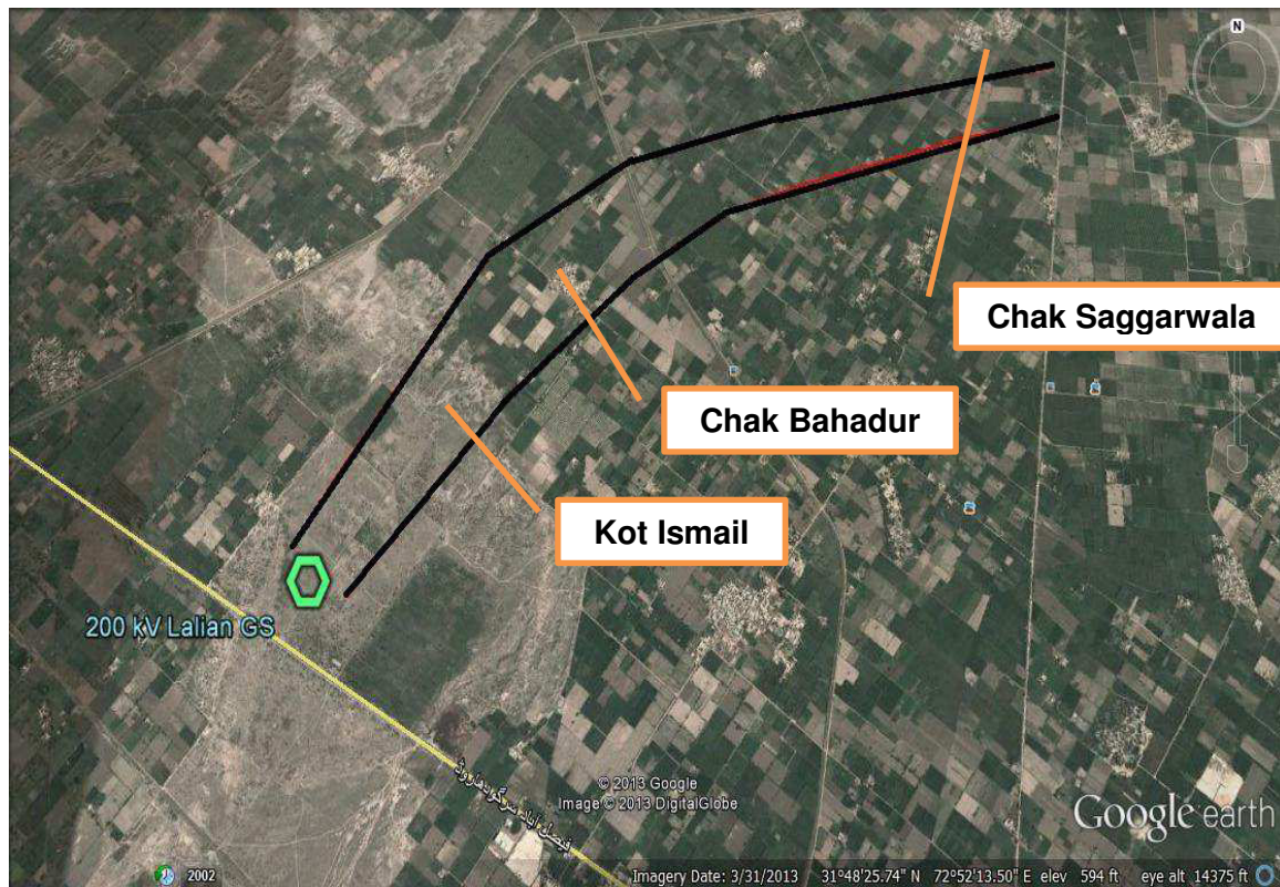
Fig 3.2: Google Image of 220 kV Lalian Allied Transmission Lines Route and Settlements along the Route
