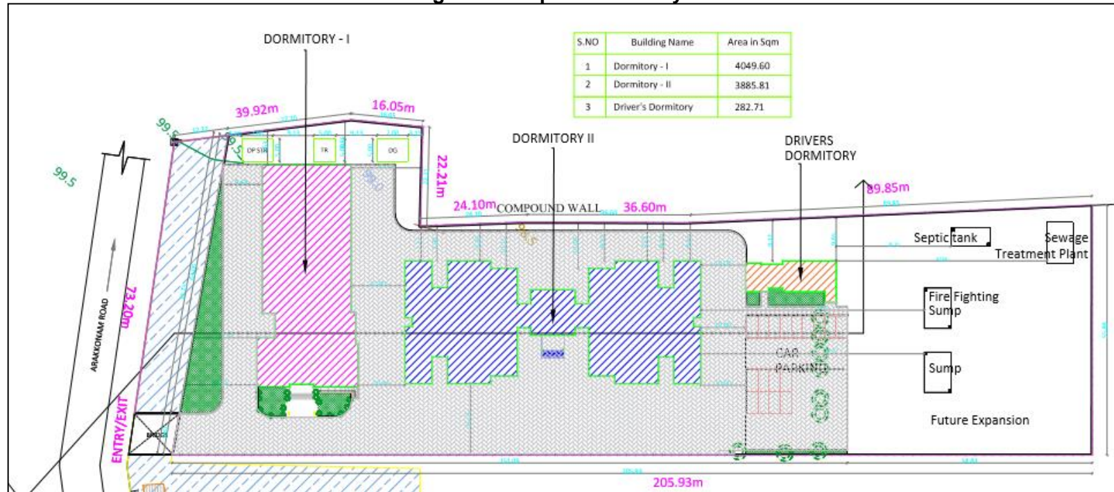
Figure 4: Proposed Site Layout
