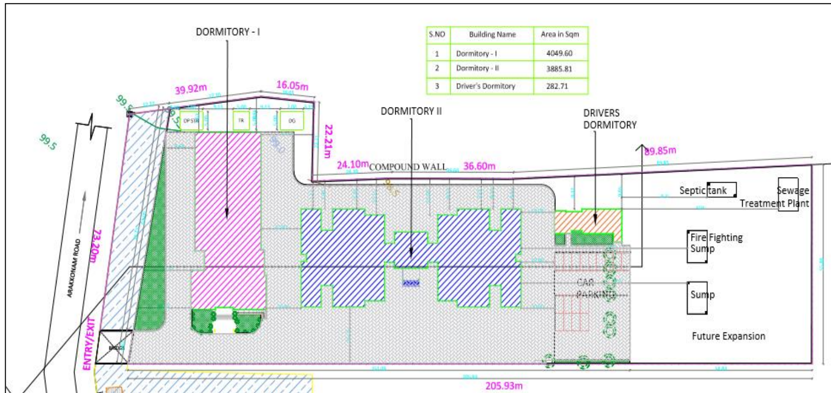
Figure 3: Proposed site plan for subproject components
