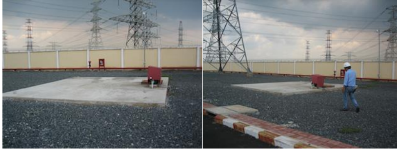
Photo 7: Oil Containment for Existing Transformers
