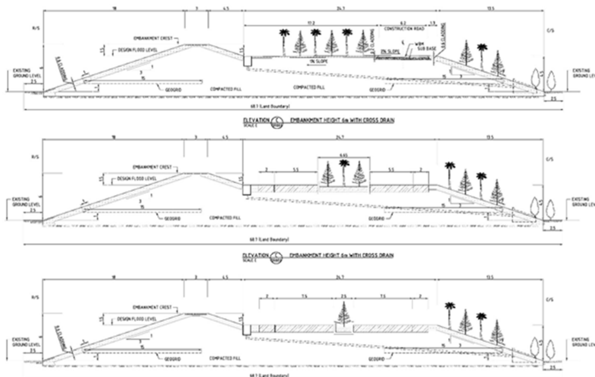
Figure 2: Cross section of the proposed embankment with developing road solutions
