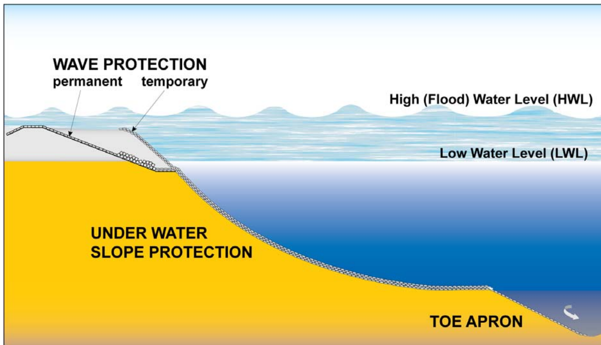
Figure 3: Layout of Bank Protection Works
