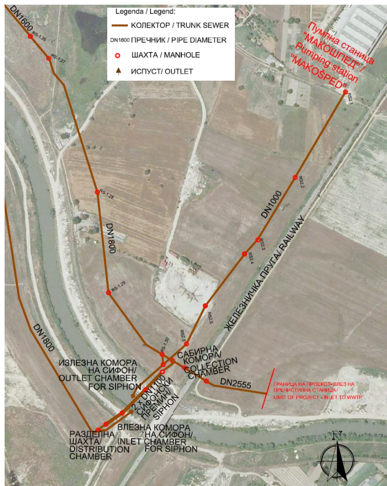
Picture 15. Map of Trunk Sewer on Left and Right Bank of the Vardar River, Siphon and WWTP Location (source: Book 2 Detailed Design of Siphon Crossing below the Vardar River and Connection to the WWTP)
