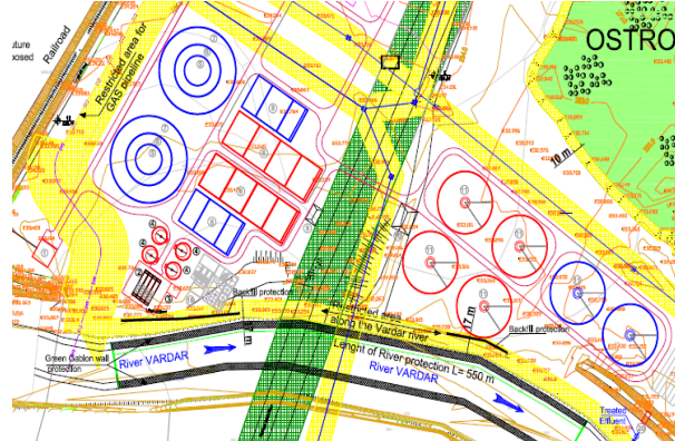
Picture 25. Location and length of riverbank to be protected
