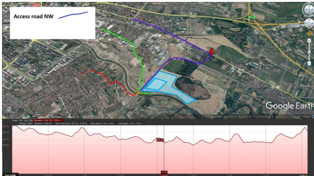
Picture 59. Position of Access Roads - from SW (red), W (green) and NW (purple) (source: Google Earth)
