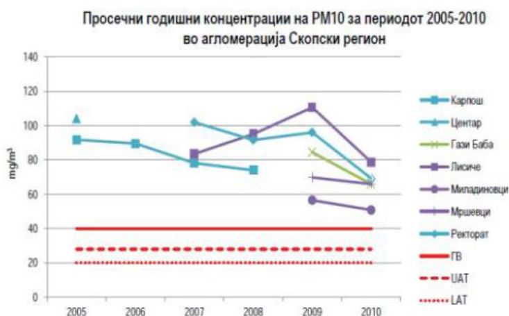
Picture 38. Average annual concentration in the period 2005-2010 for PM 10 in Skopje, agglomeration
