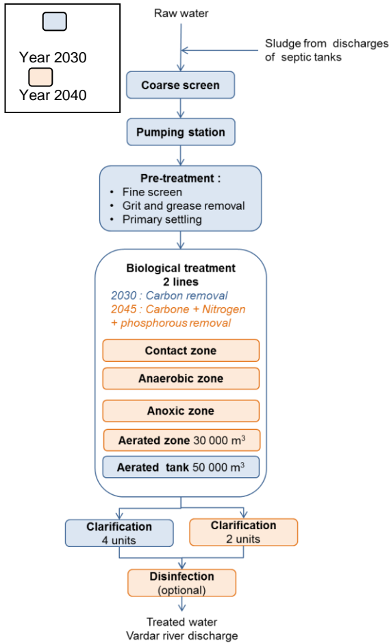
Picture 18. Wastewater treatment diagram
