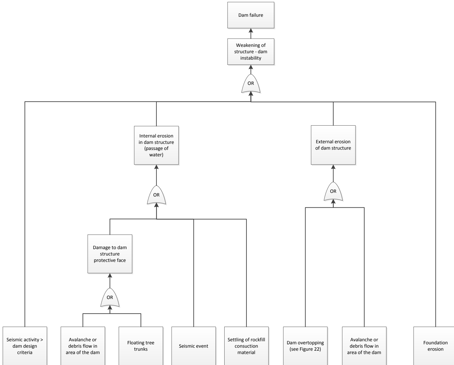
Figure 19 – Fault tree for dam failure during operation
