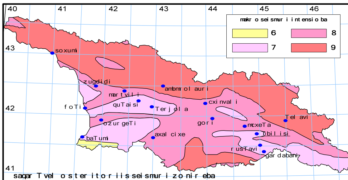
Map 3: Seismic Zone Map of Georgia
