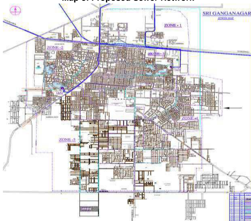
Map 3: Proposed Sewer Network
