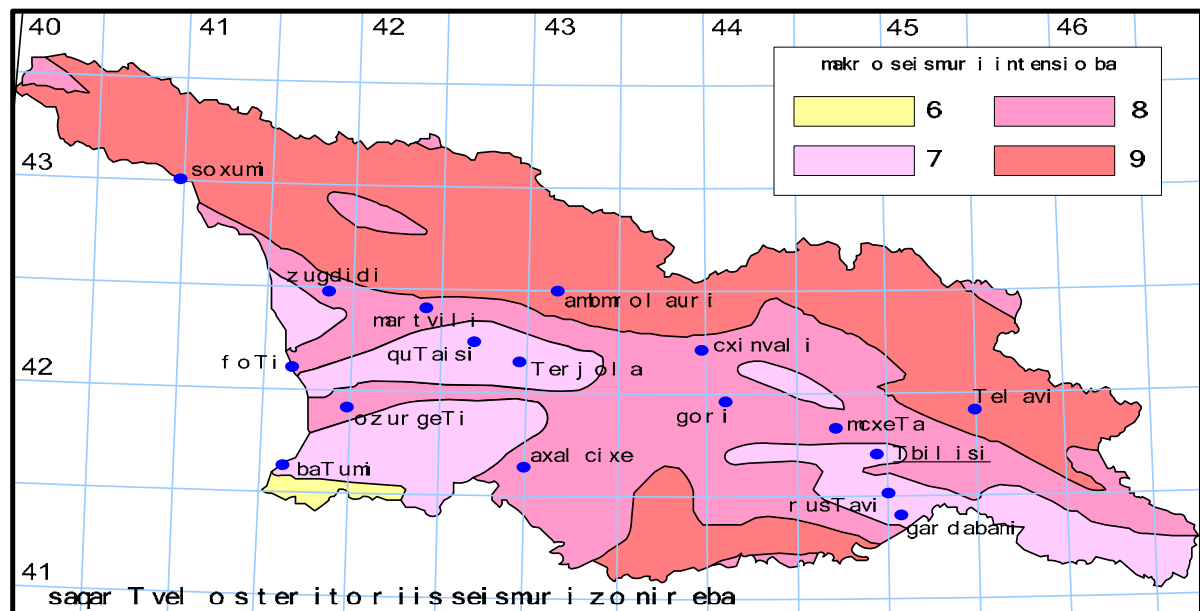
Map 4: Seismic Zones of Georgia
