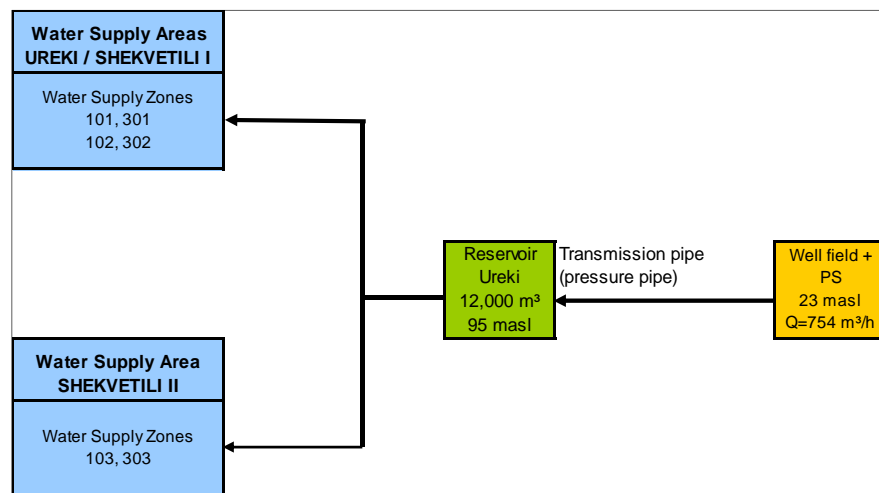
Fig. 3 Simplified Water Supply Flow Scheme – Option 1
