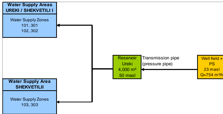
Fig. 4 Simplified Water Supply Flow Scheme – Option 2
