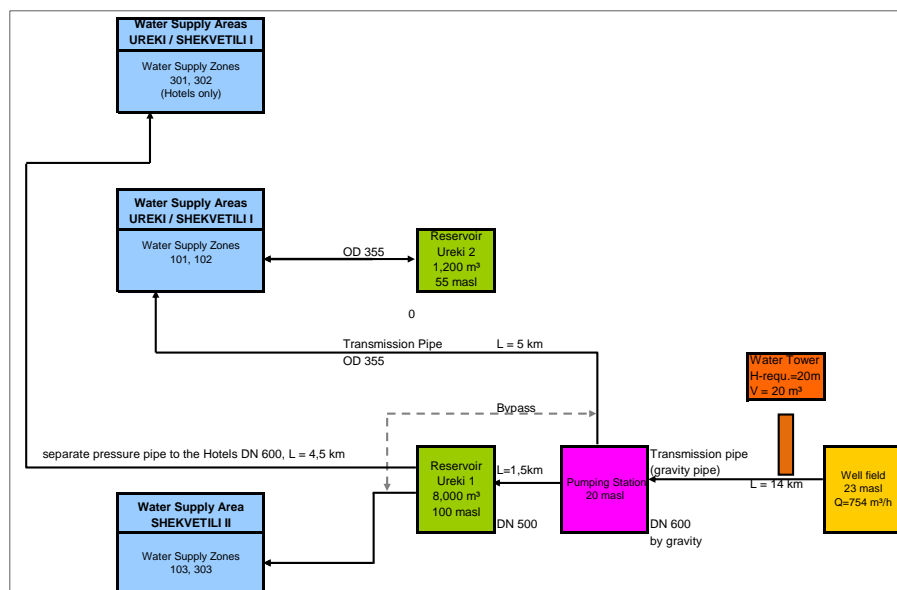
Fig. 5 Simplified Water Supply Flow Scheme – Option 3
