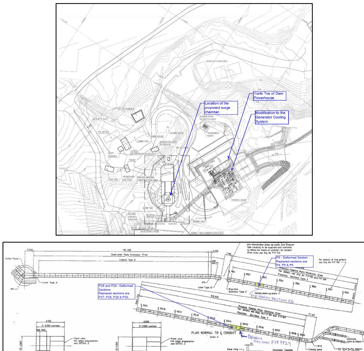
Figure 2 Yonki Toe of Dam Work
