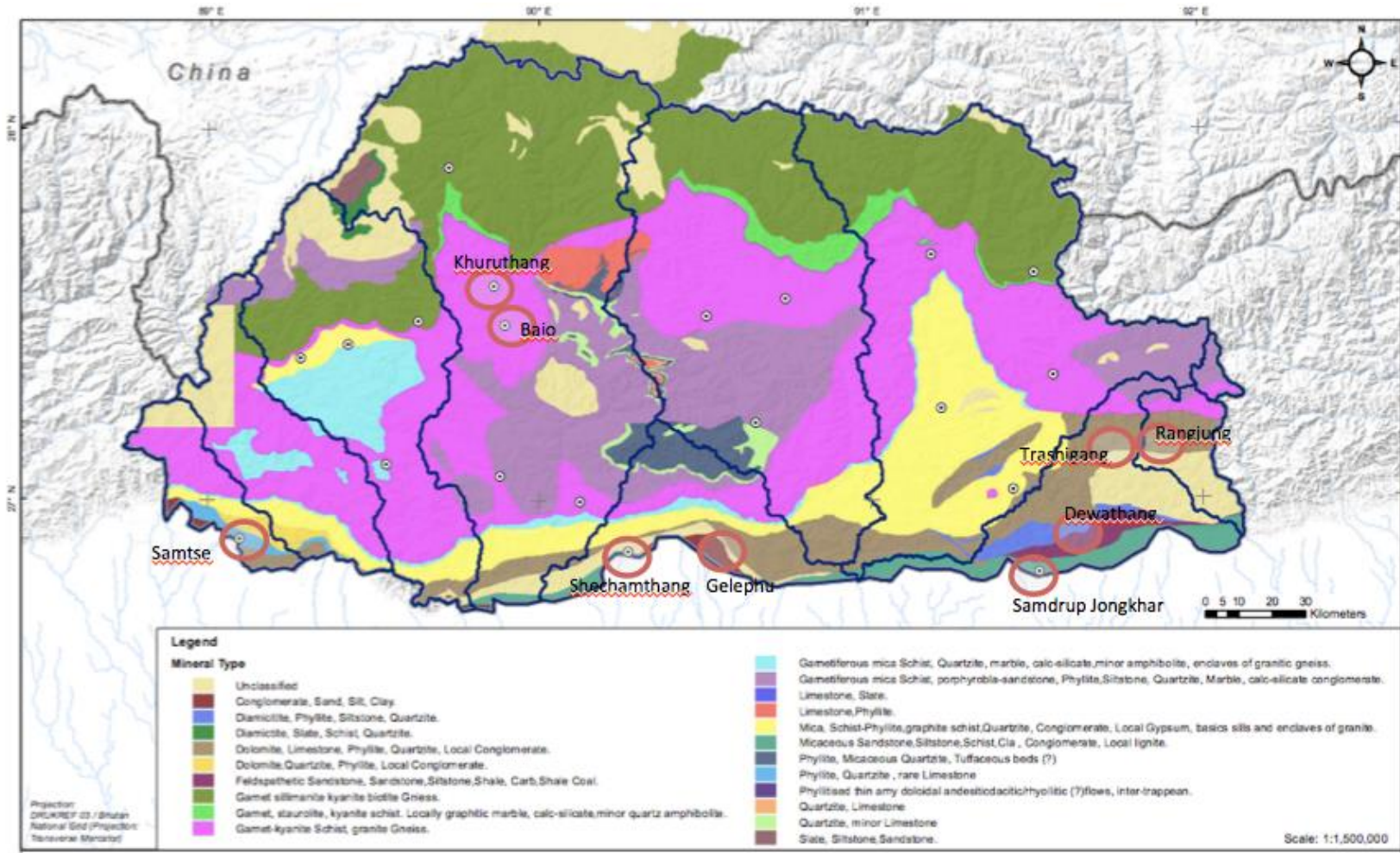
Figure 5: Geology of the Sites in Samdrup Jongkhar and Other Locations under Secondary Towns Urban Development Project and other Proposed Urban Projects
