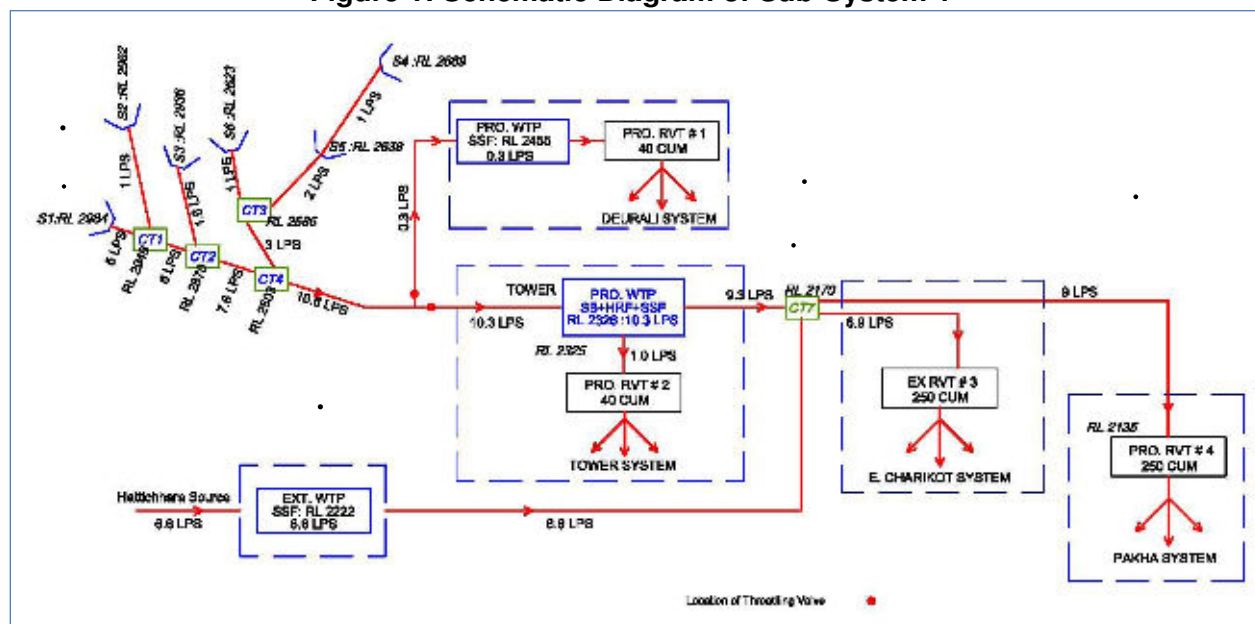
Figure 1: Schematic Diagram of Sub-System 1
