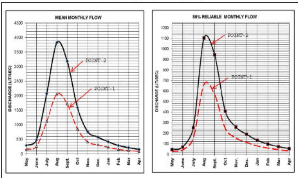
Figure 3: Predicted Mean monthly Flows and Predicted Reliable Flow at Hattichahara and Ghatta Abstraction Locations
