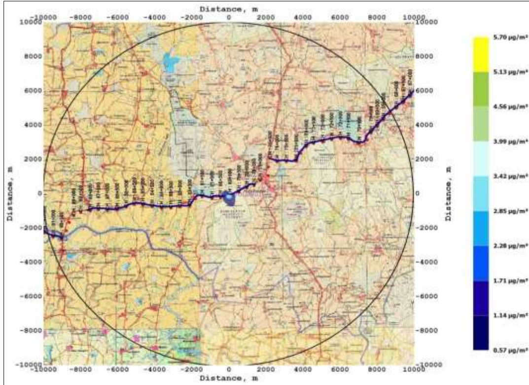
Figure 42 Predicted PM Levels in Traffic Section III for the Year 2040
