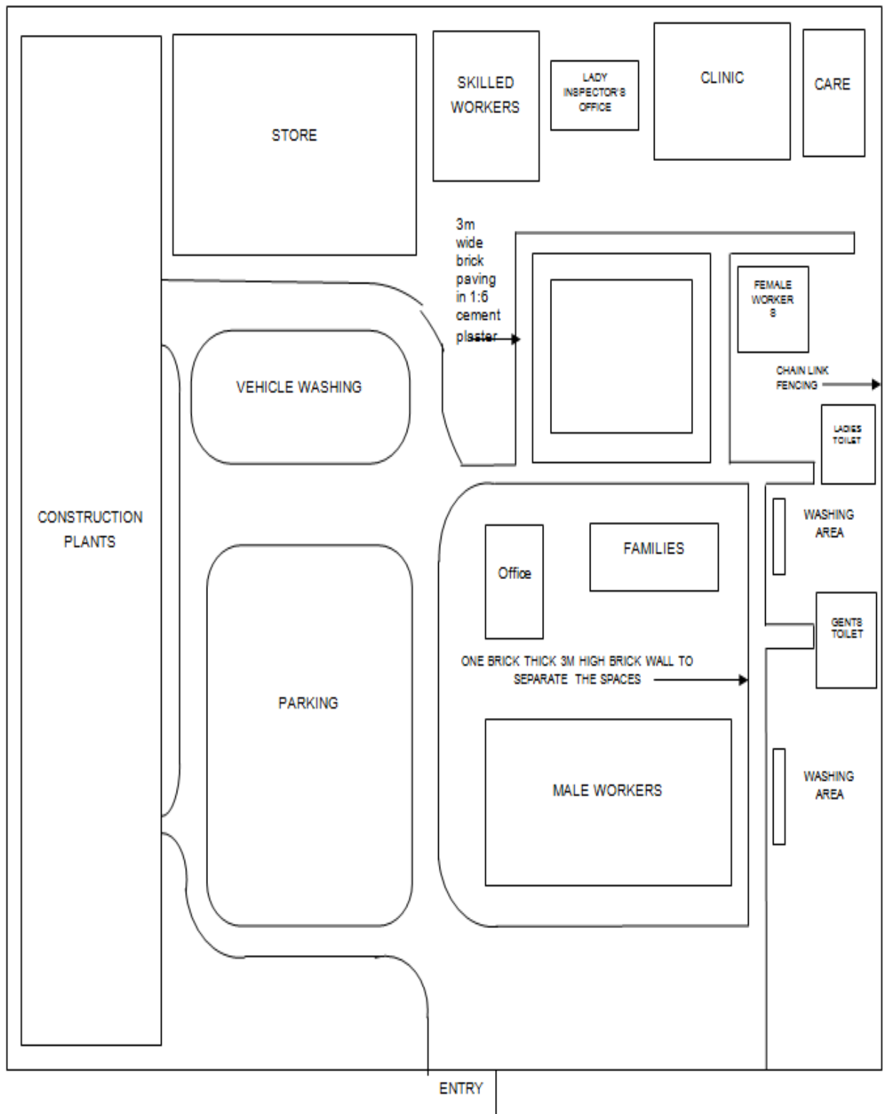
Figure-A Typical Layout of Construction Camp
