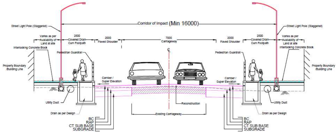
TYPICAL CROSS SECTION FOR 2-LANE WITH PAVED SHOULDER (URBAN SECTION) TCS - 4 - CONCENTRIC WIDENING BUILT UP SECTION
