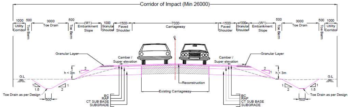
TYPICAL CROSS SECTION FOR 2-LANE WITH PAVED SHOULDER (OPEN COUNTRY) TCS- 1 - CONCENTRIC WIDENING (EMBANKMENT HEIGHT <3M)
