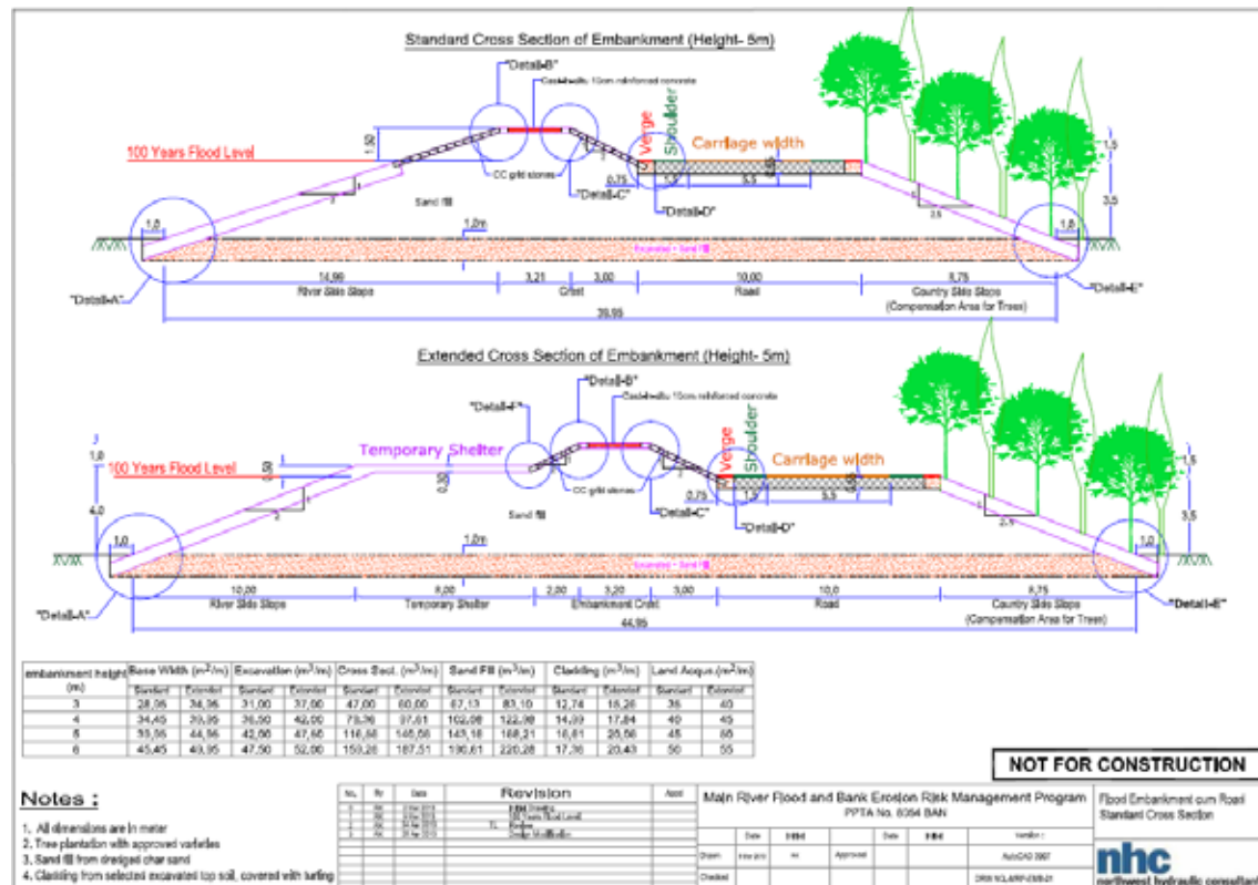
Figure 4.3: Embankment, Representative Cross-Section
