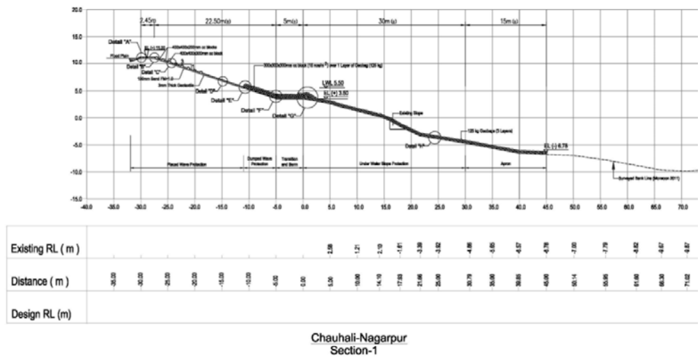
Figure 4-1: Riverbank Protection, Representative Cross-Section
