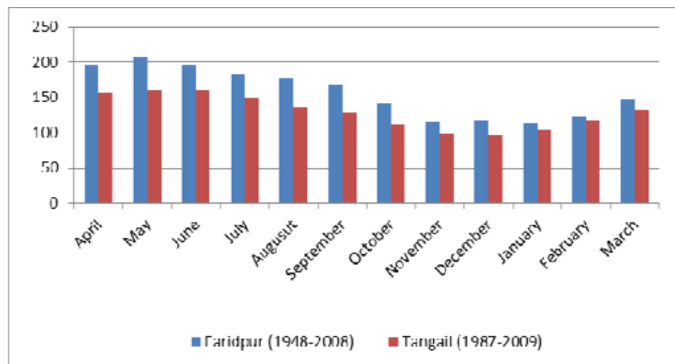
Figure 5.5: Windspeed of the study area
