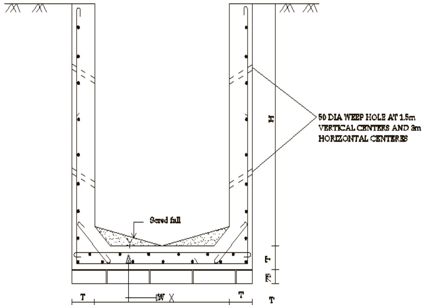
Figure 8: Typical Reinforced Cement Concrete U-drain
