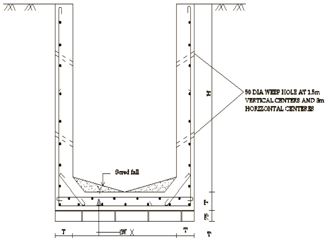
Figure 7: Typical Reinforced Cement Concrete U-drain
