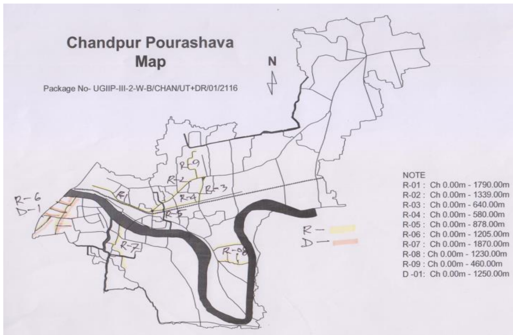
Figure 2: Proposed Road & Drain Sub-projects in Chandpur Pourashava (Package-1)
