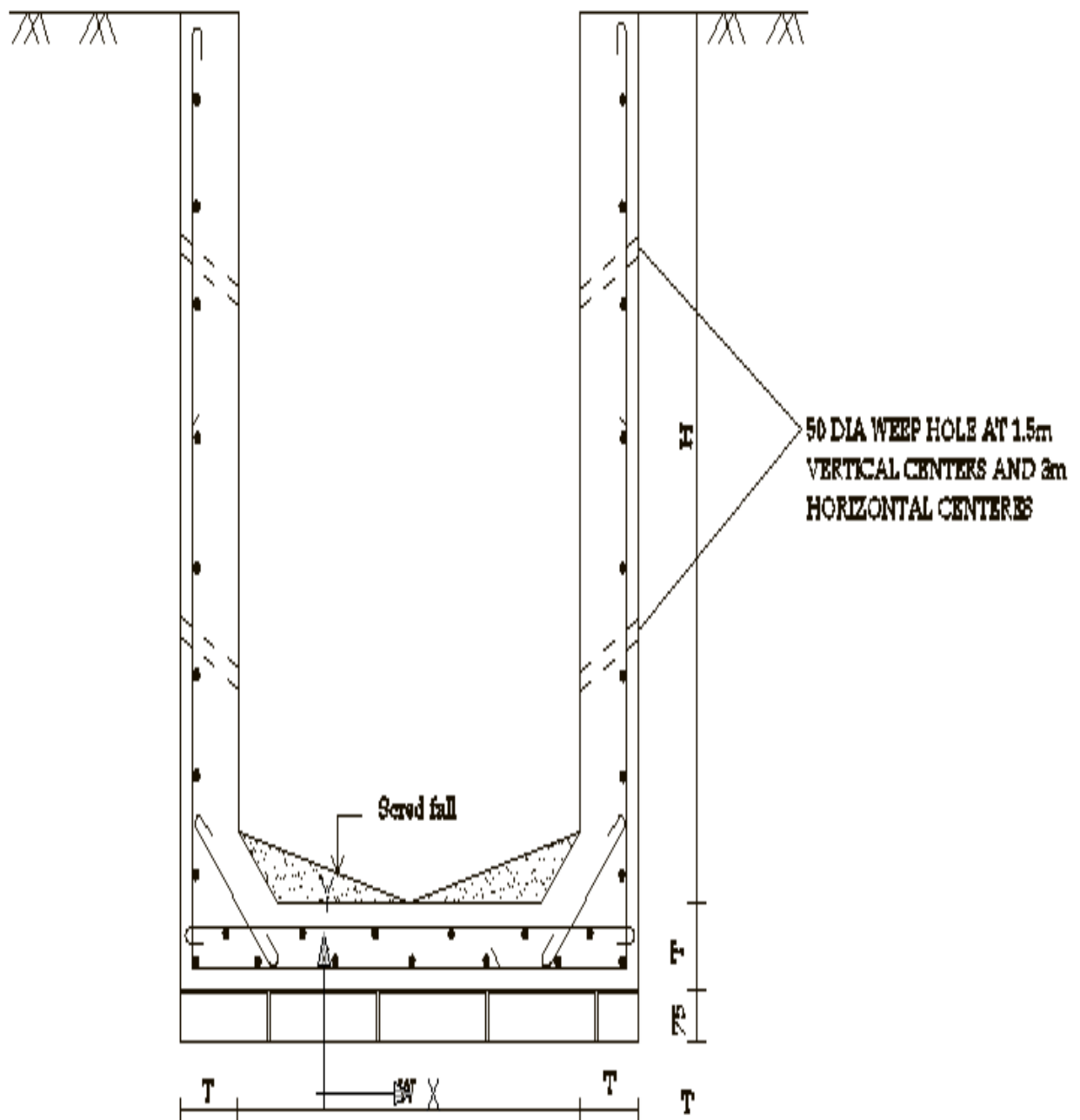
Figure 8: Typical Reinforced Cement Concrete U-drain
