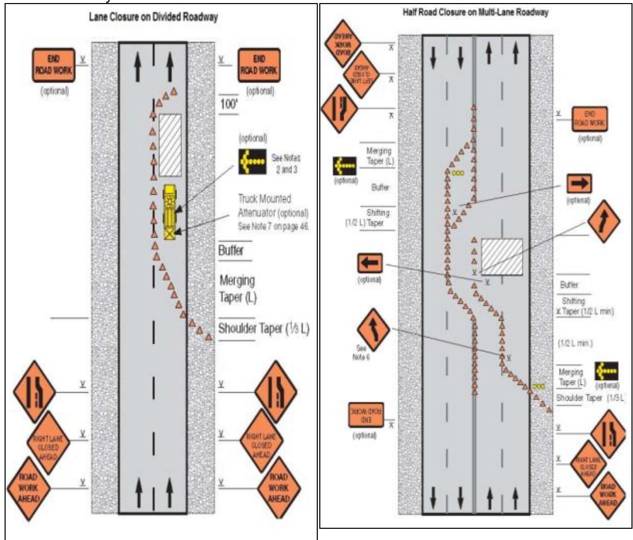
Figure A10 &amp; A11: Lane Closure on Divided Roadway &amp; Half Road Closure On Multi-Lane Roadway
