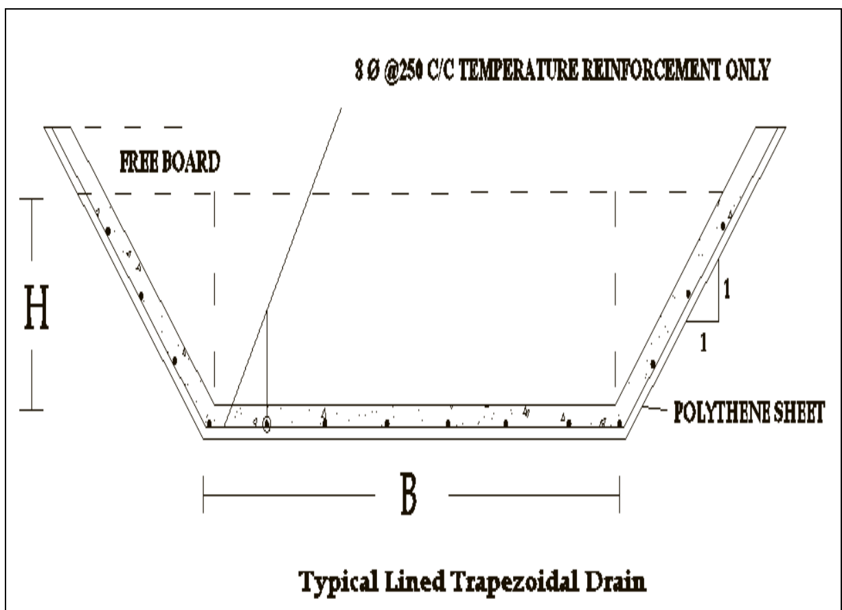
Figure 6: Typical Trapezoidal line Drain
