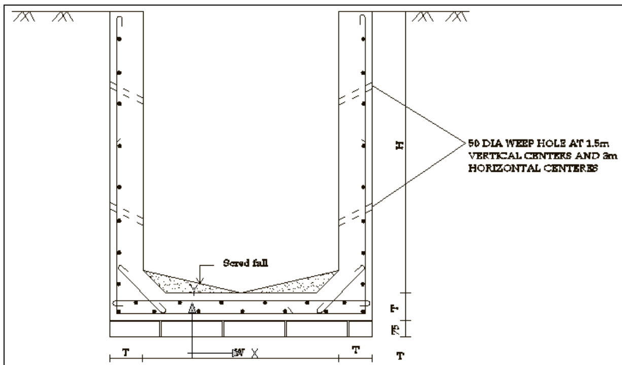
Figure 5: Typical Reinforced Cement Concrete U-drain
