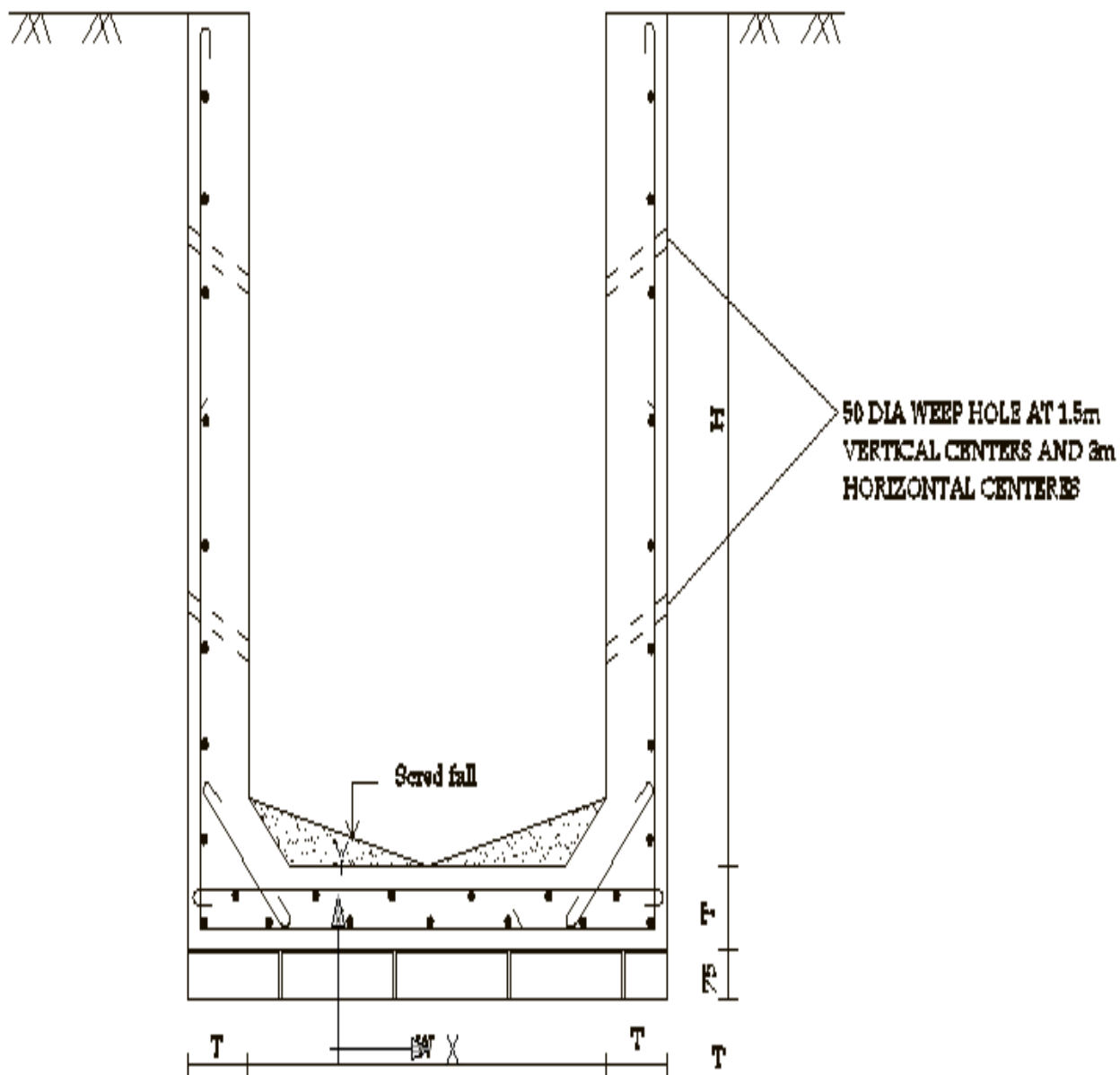
Figure 8: Typical Reinforced Cement Concrete U-drain
