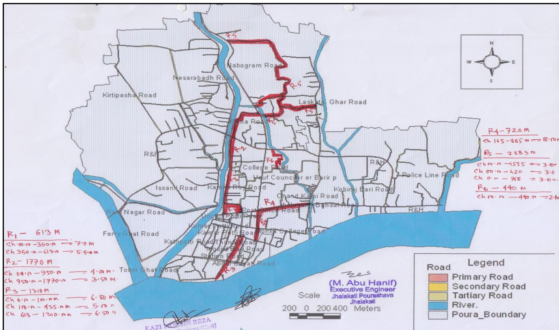
Figure 2: Proposed Roads in Jhalokathi Pourashava
