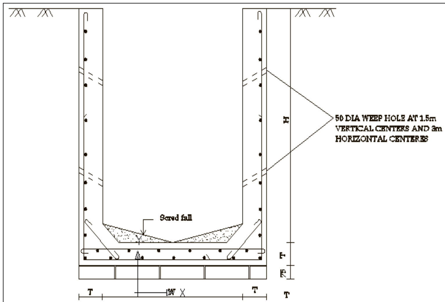
Figure 9: Typical Reinforced Cement Concrete U-drain
