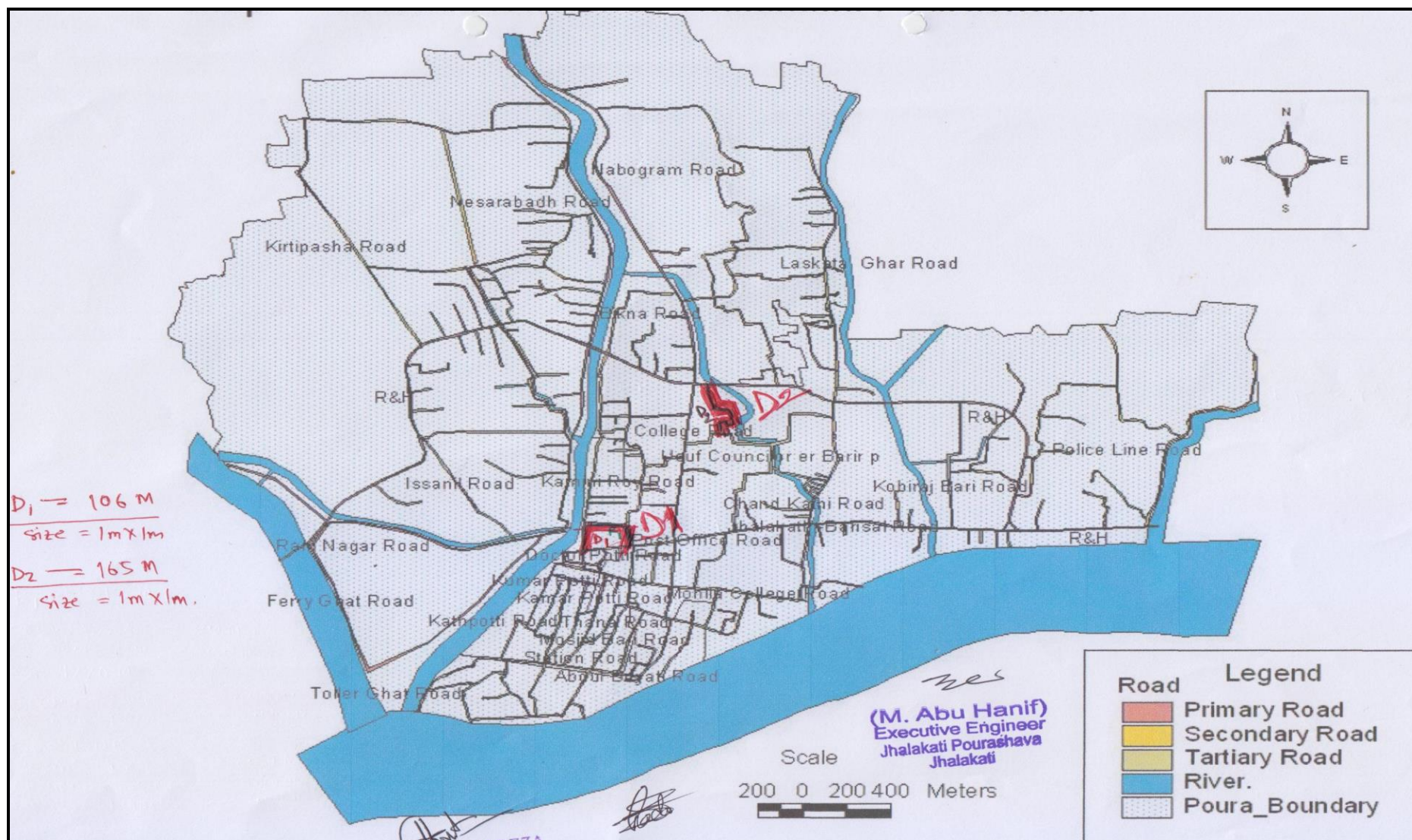
Figure 3: Proposed Drains in Jhalokathi Pourashava
