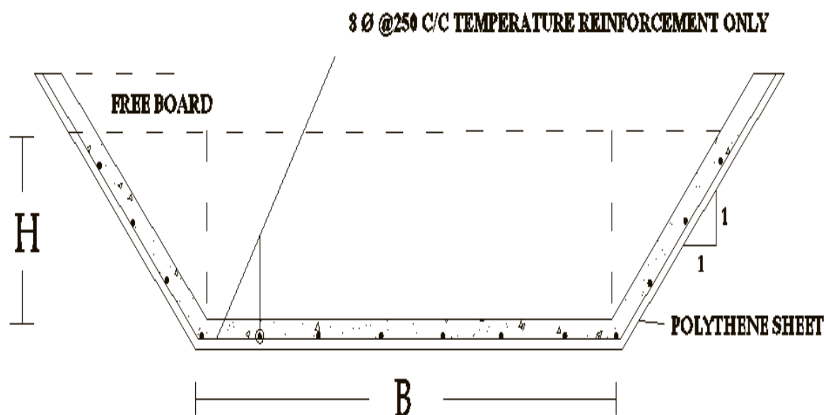
Typical Lined Trapezoidal Drain
