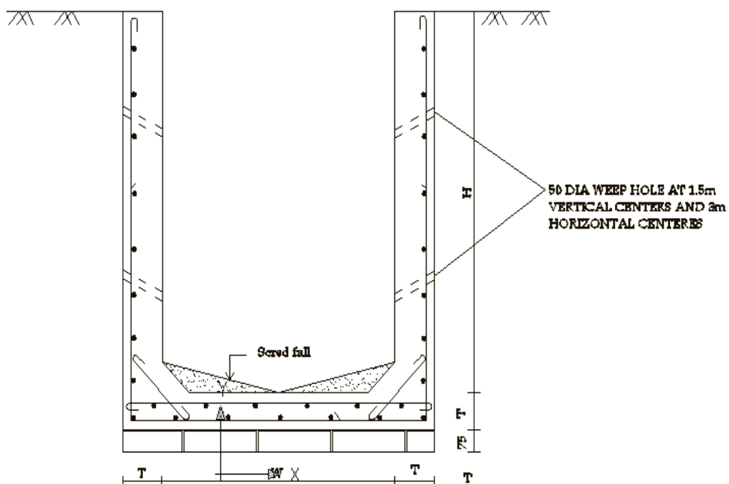
Figure 5: Typical Reinforced Cement Concrete U-drain
