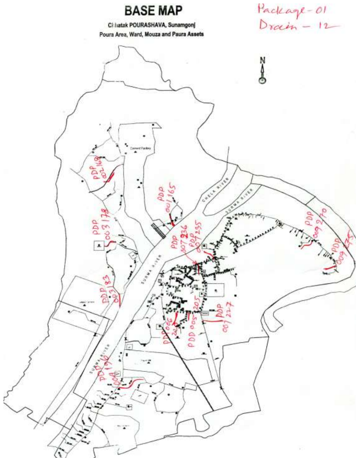
Figure 4: Proposed Drain Sub-projects under Package-1 (Phase-2) Chhatak Pourashava
