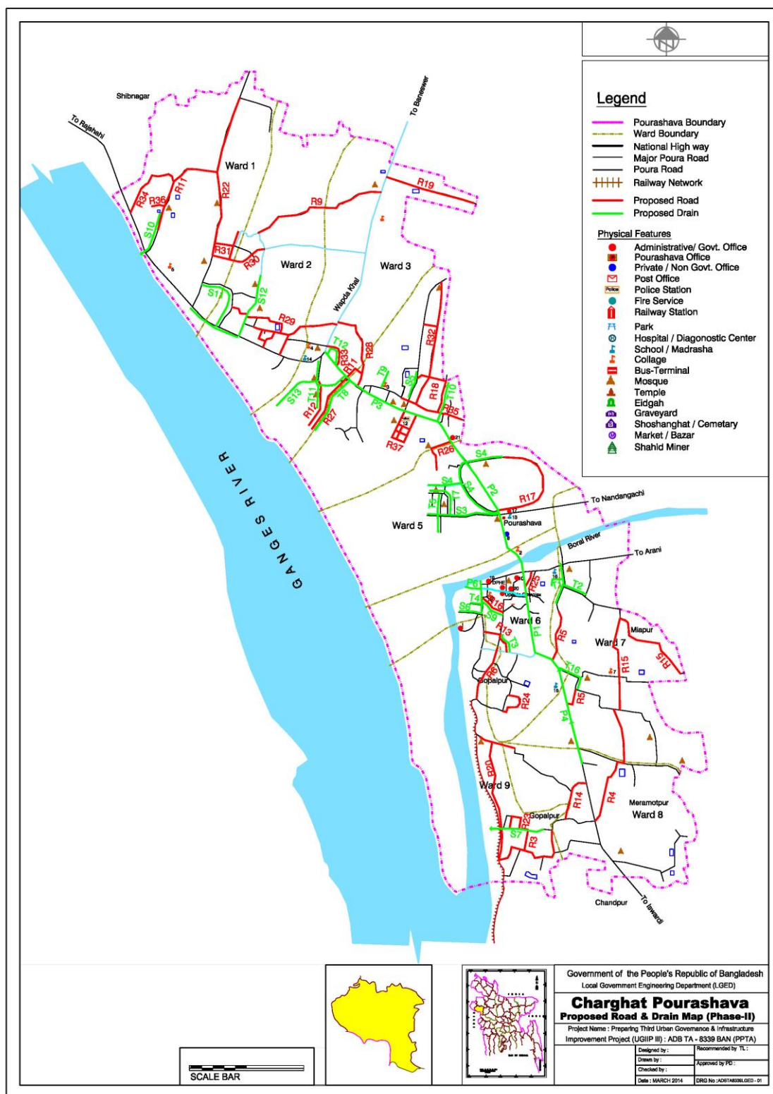
Figure 2: Proposed Drainage Works in Charghat Pourashava
