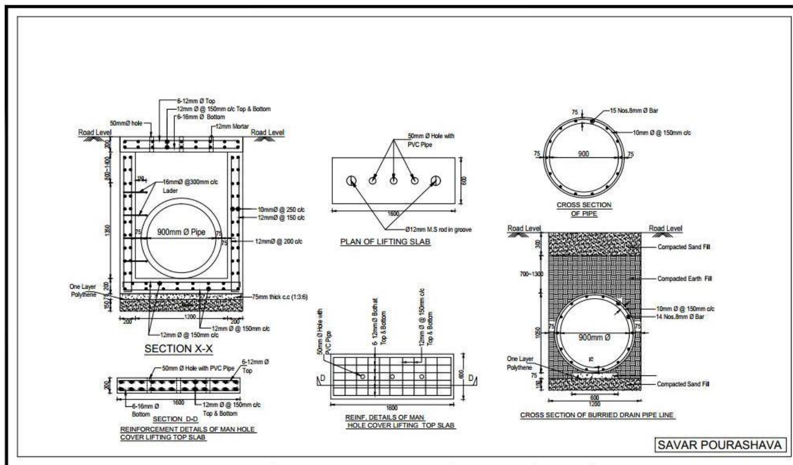
Figure 7: Typical Reinforced Cement Concrete Pipe Drain
