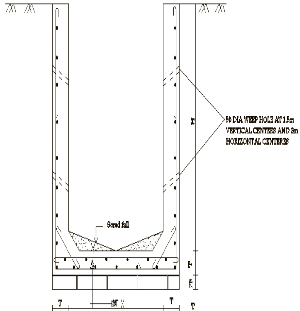
Figure 6: Typical Reinforced Cement Concrete U-drain
