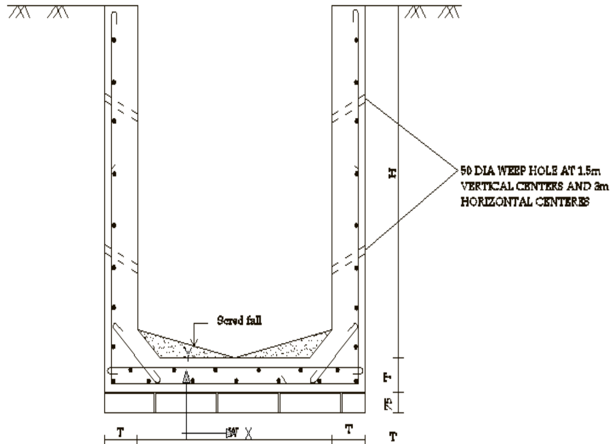
Figure 7: Typical Reinforced Cement Concrete U-drain
