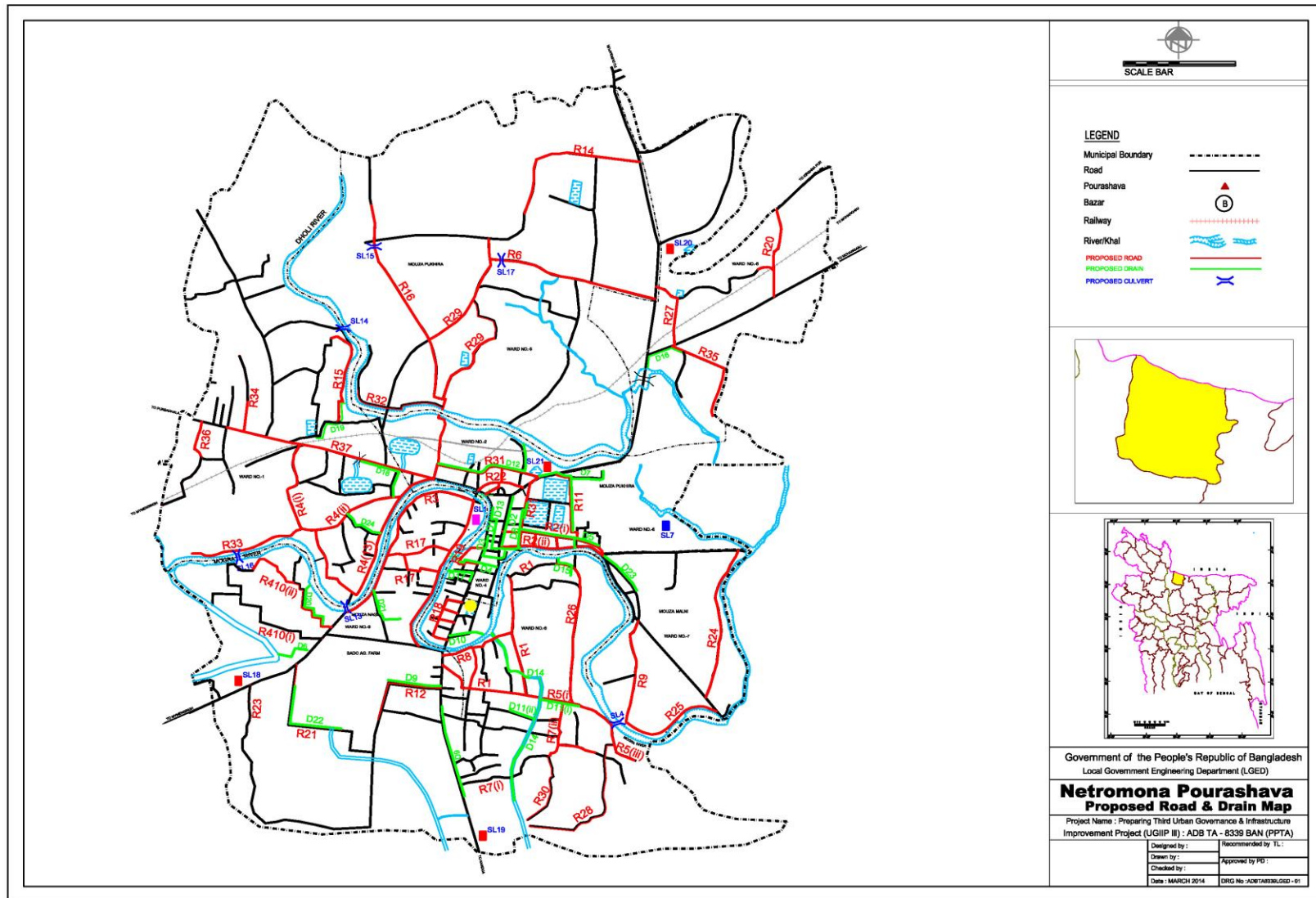
Figure 2: Proposed Drainage Works in Netrokona Pourashava
