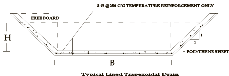
Figure 4: Typical RCC Trapezoidal Line Drain
