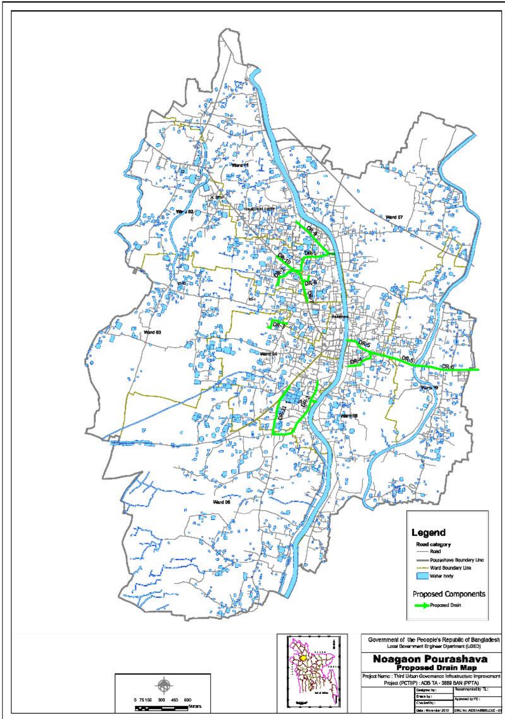
Figure 2: Proposed Drainage Works in NaogaonPourashava
