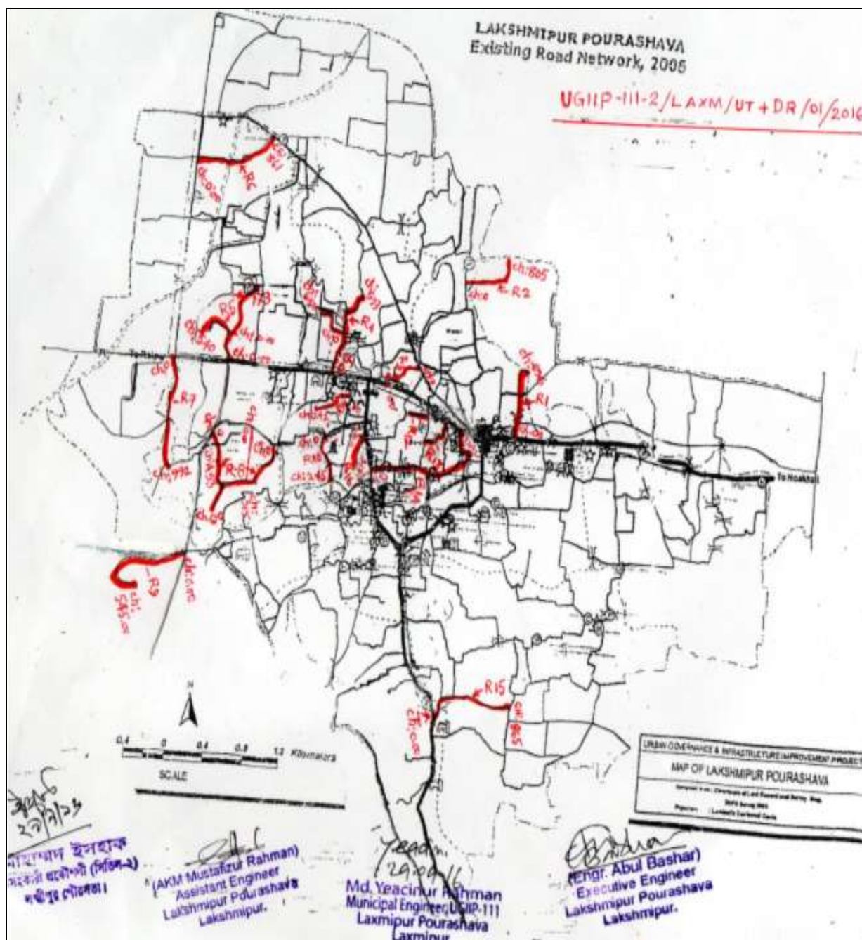
Figure 2: Proposed Road Sub-projects under Package-1 (Phase-2) Laxmipur Pourashava
