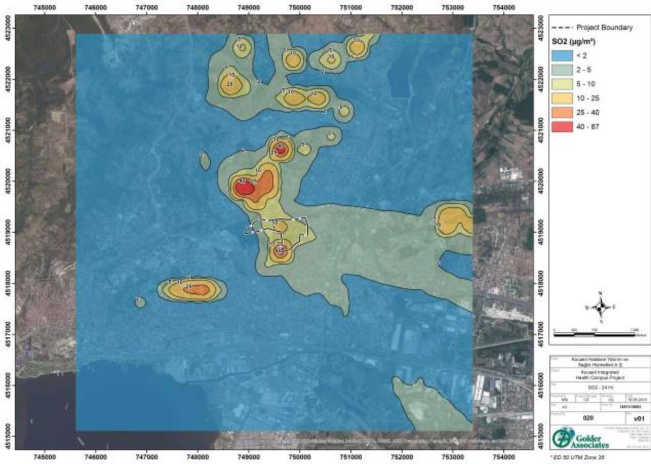
Figure 78: SO2 Daily
