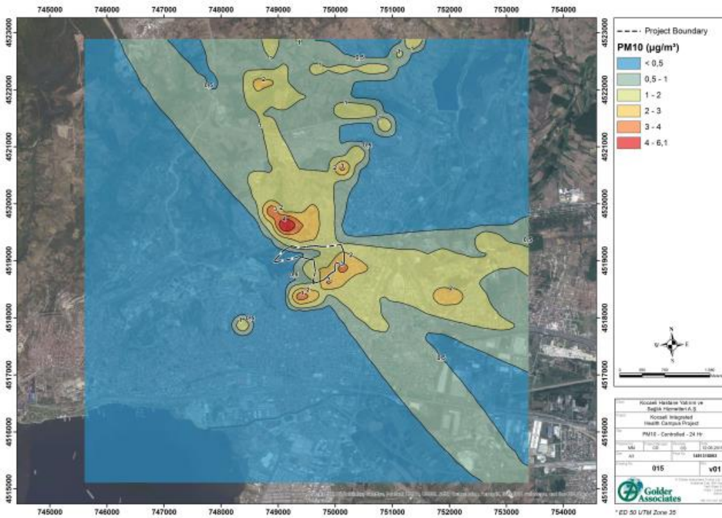
Figure 67: Controlled Daily
