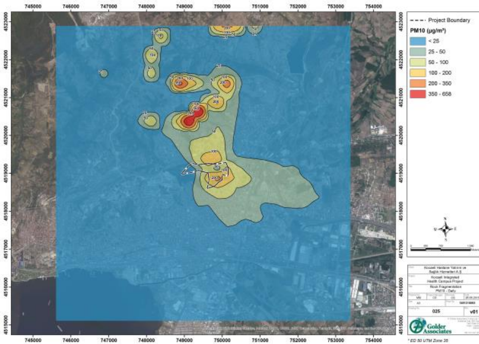
Figure 73: Fragmentation Daily
