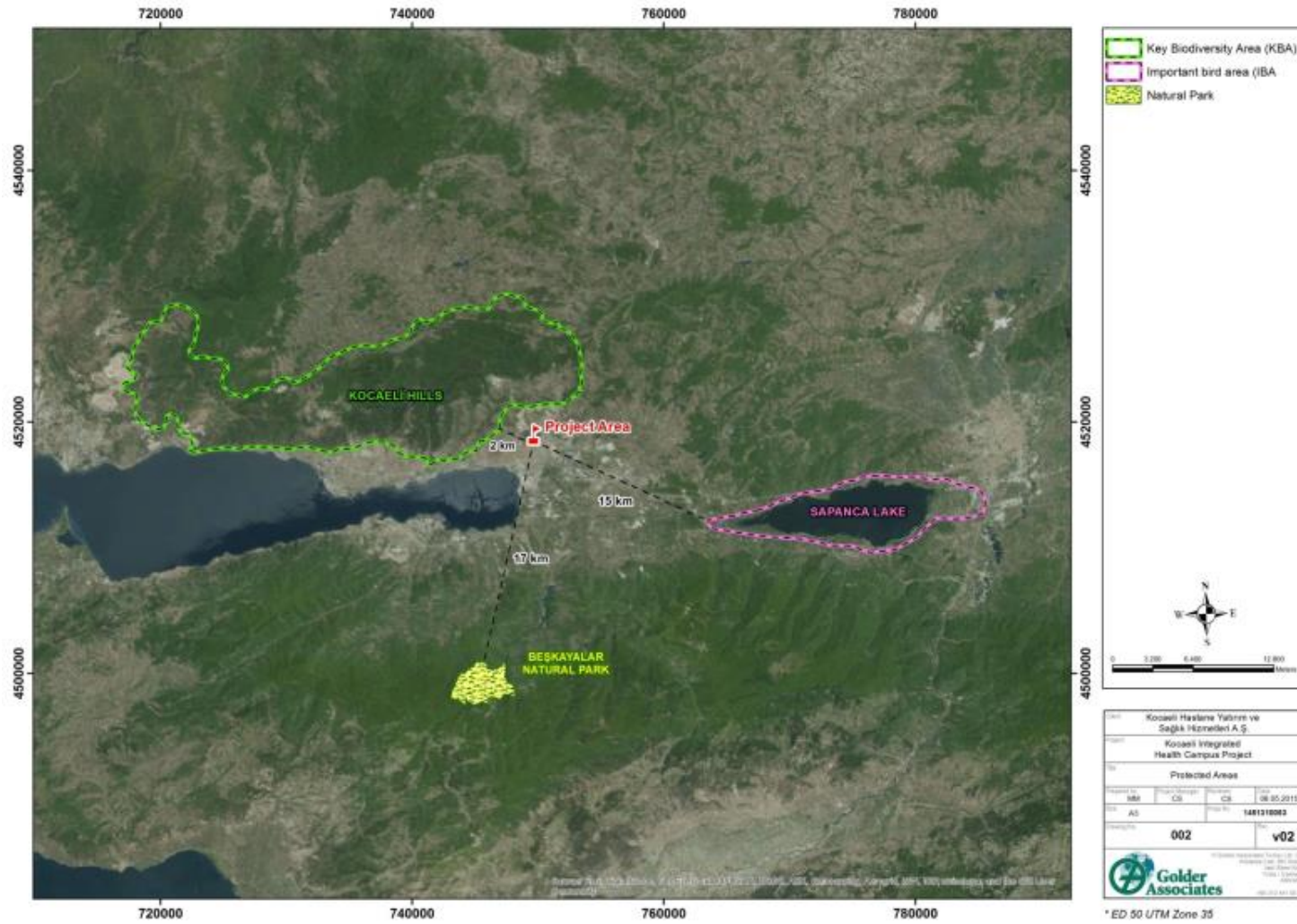
Figure 16: Protected Areas
