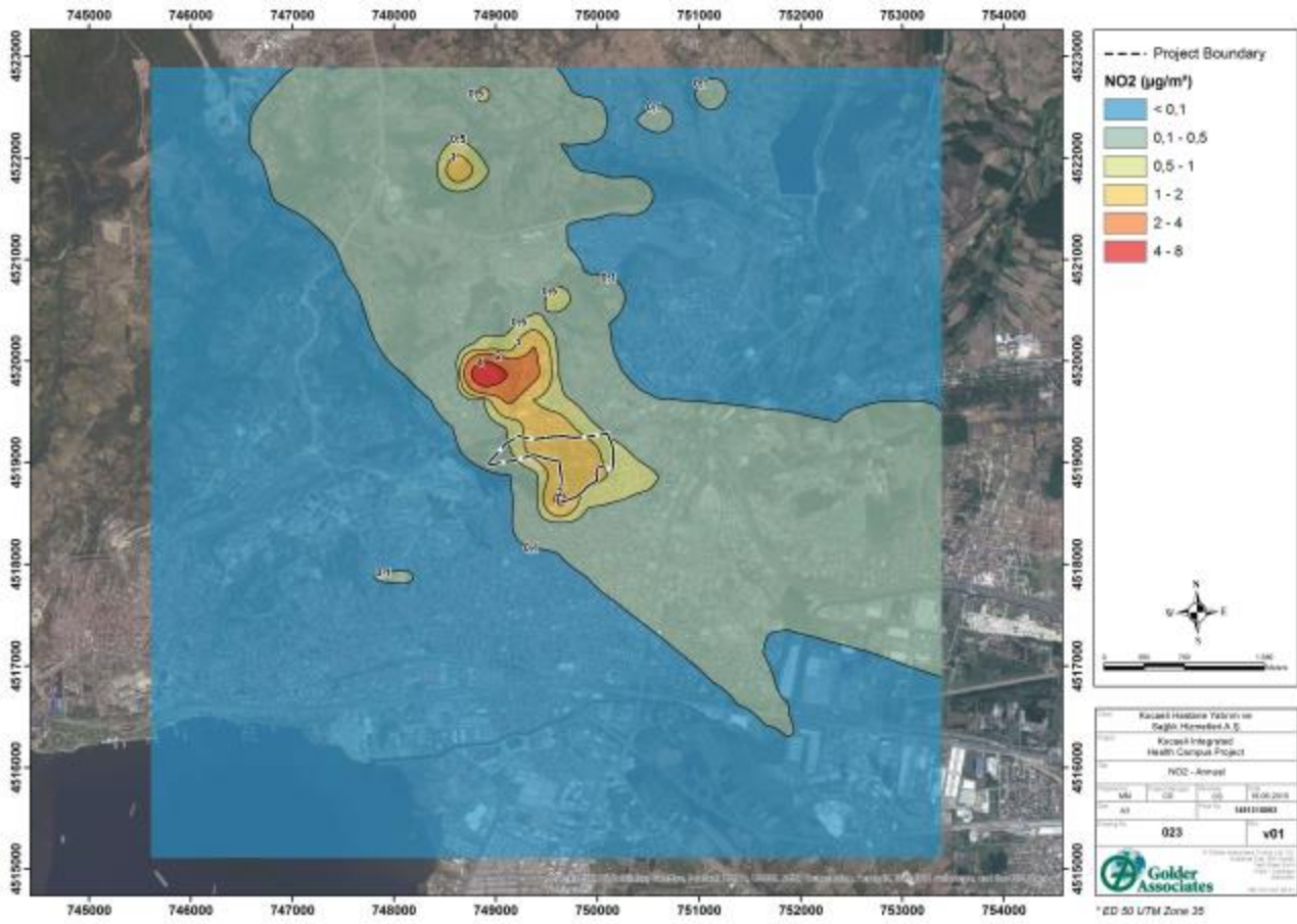
Figure 75: NO2 Annual
