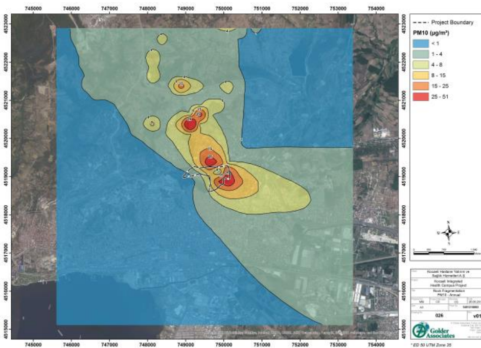
Figure 72: Fragmentation Annual
