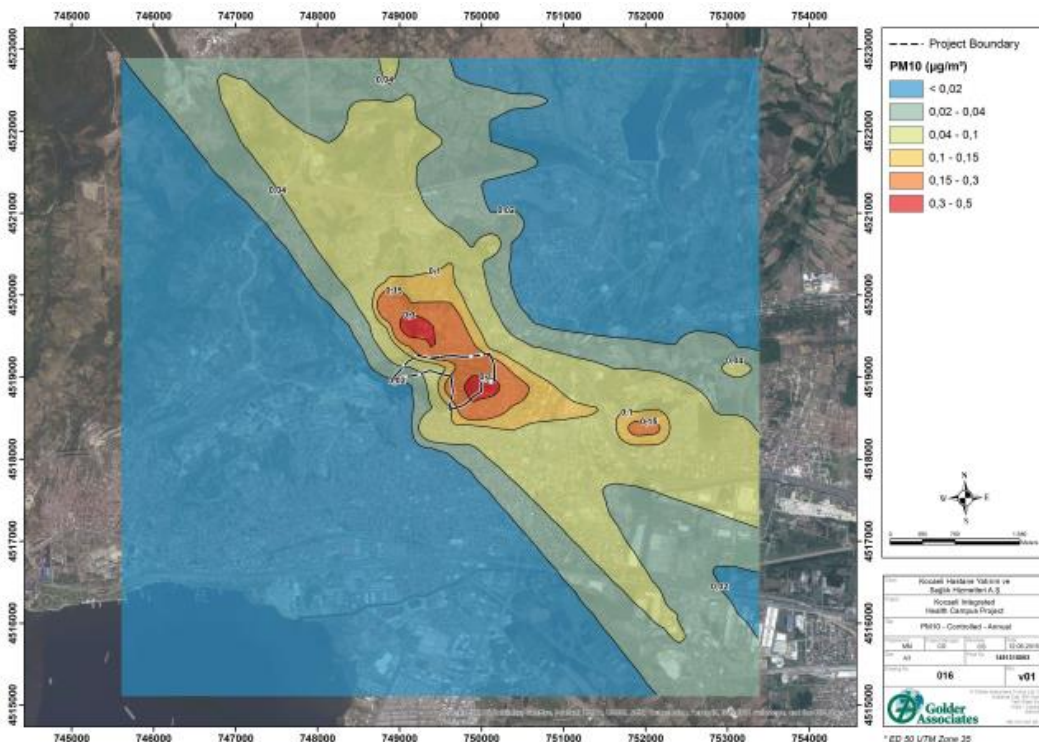
Figure 66: Controlled Annual
