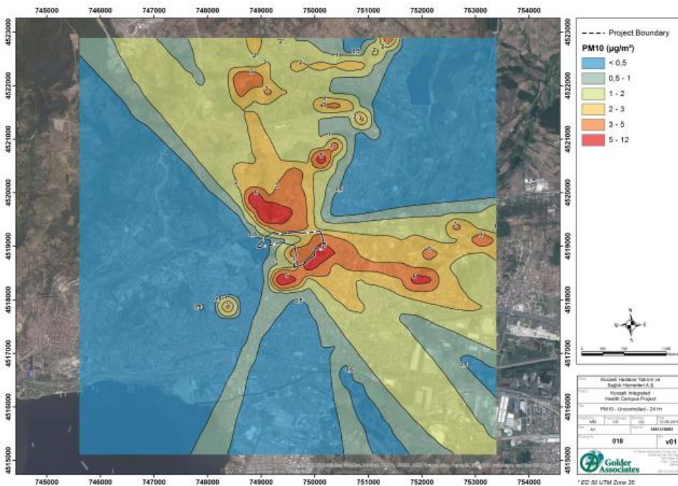
Figure 70: Uncontrolled Daily
