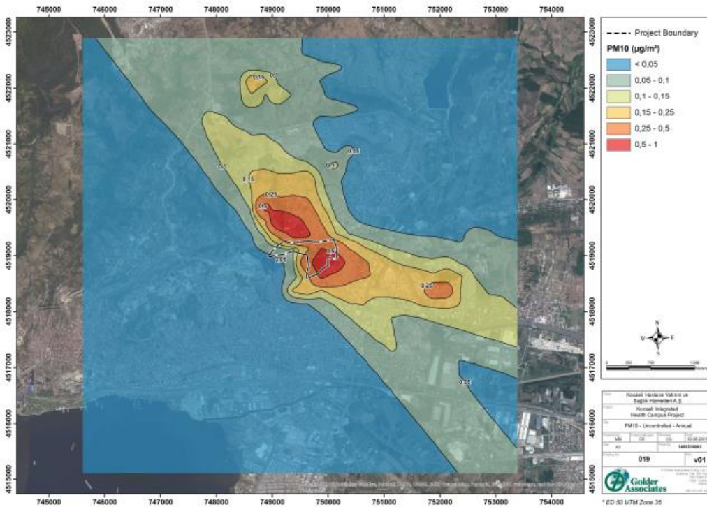
Figure 69: Uncontrolled Annual
