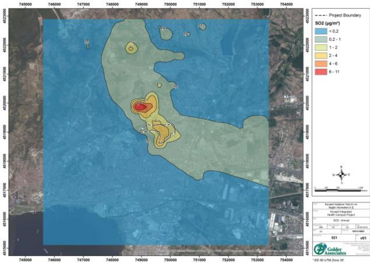
Figure 77: SO 2 Annual
