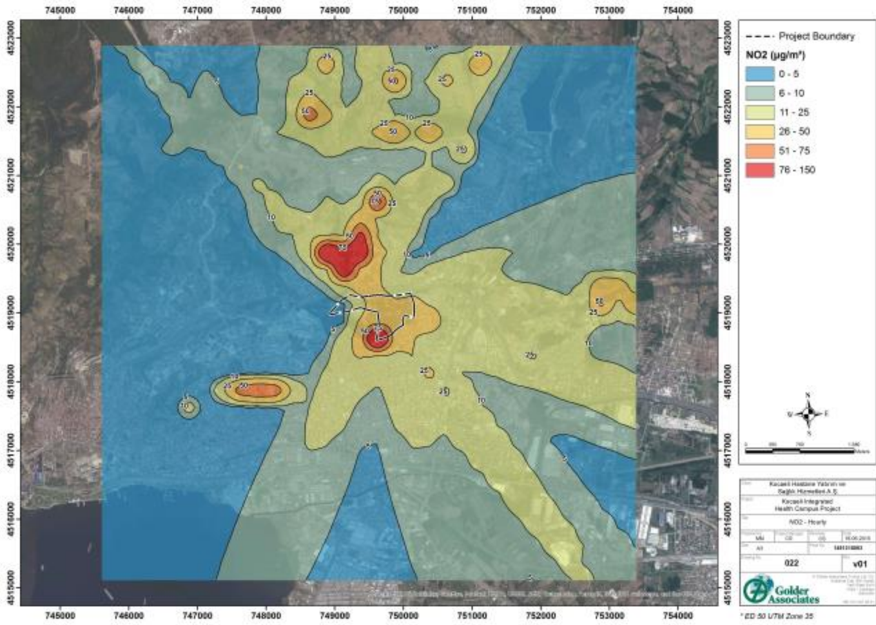
Figure 76: NO 2 Hourly
