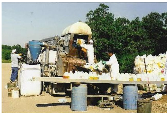
Figure 15 : Mobile shredder
