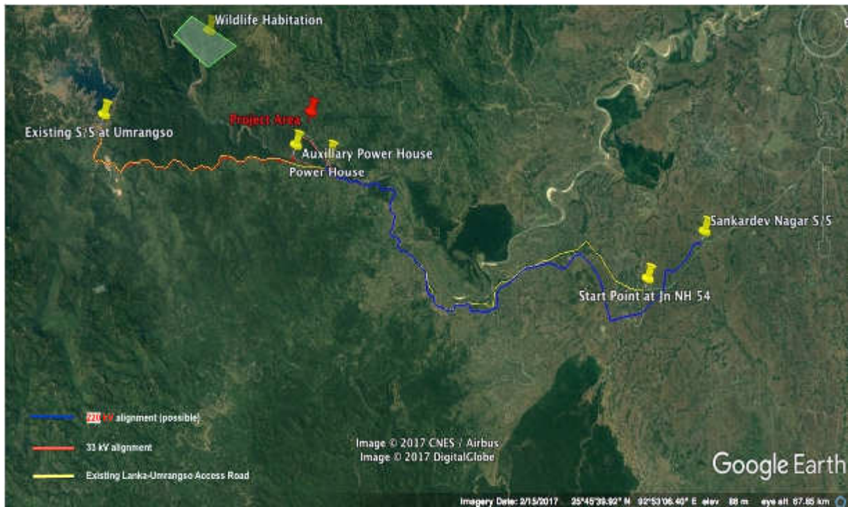
Figure 7: Transmission Line Alignment Corridors and Possible Wildlife Habitat Areas
