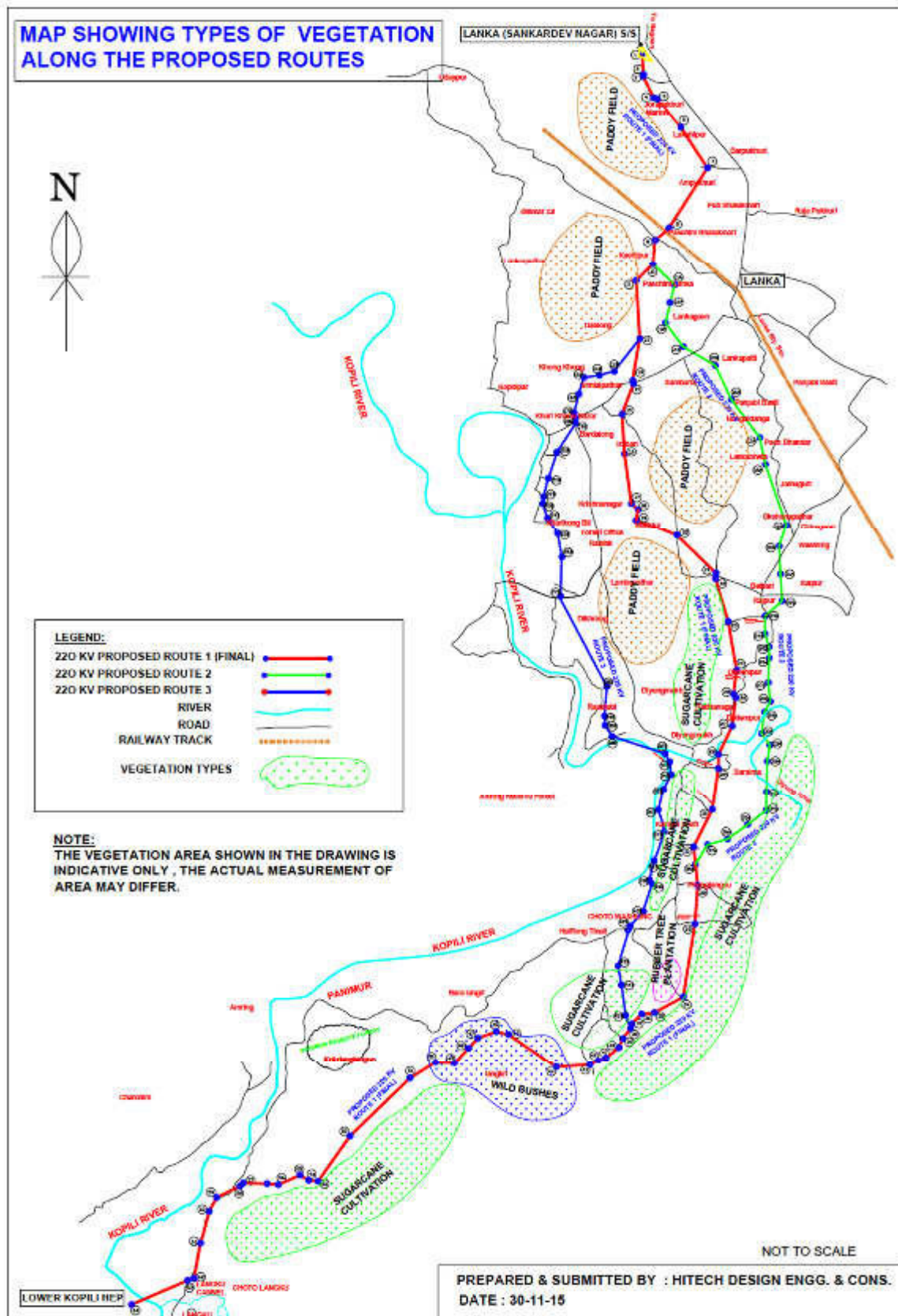
Figure 5: Proposed routes for 220 kV TL with vegetation cover
