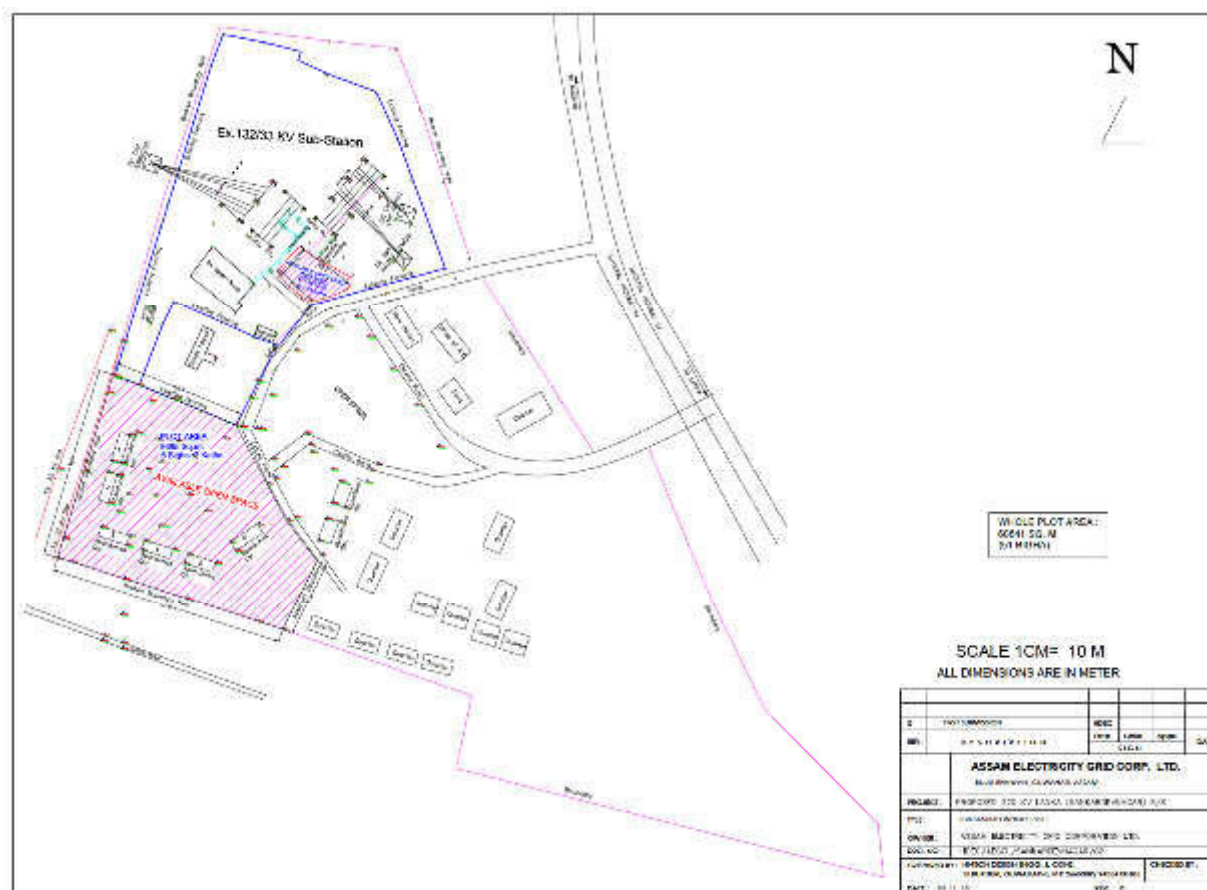
Figure 6: Site Plan of an existing S/S at Lanka
