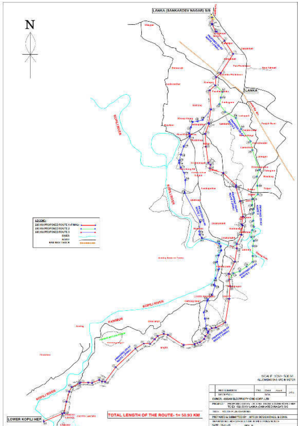
Figure 3: Proposed route map for the 220 kV TL with routing options
